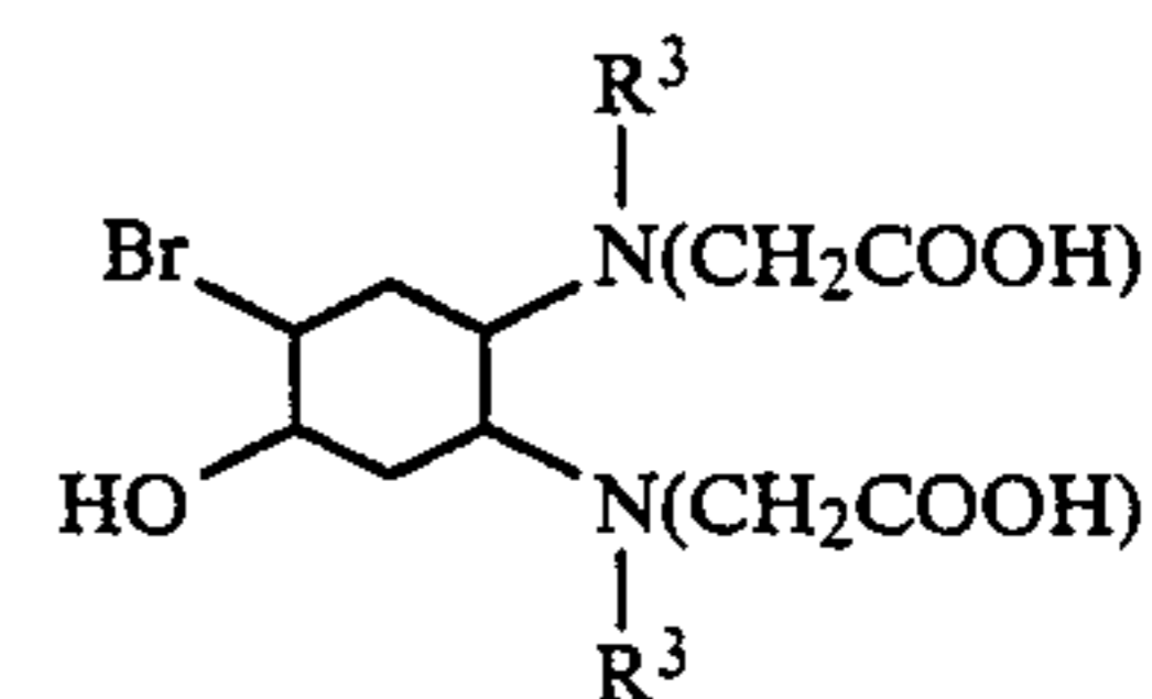
Scheme V:
