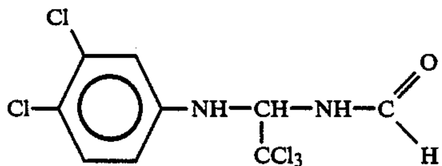
(CHLORANIFORMETHAN)
