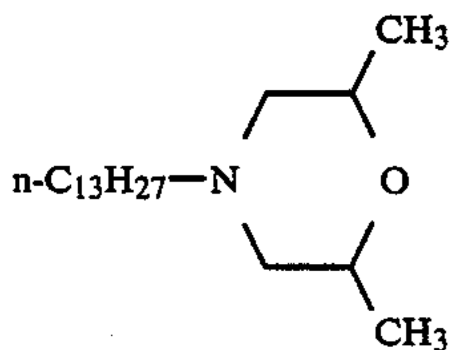
(TRIDEMORPH)
