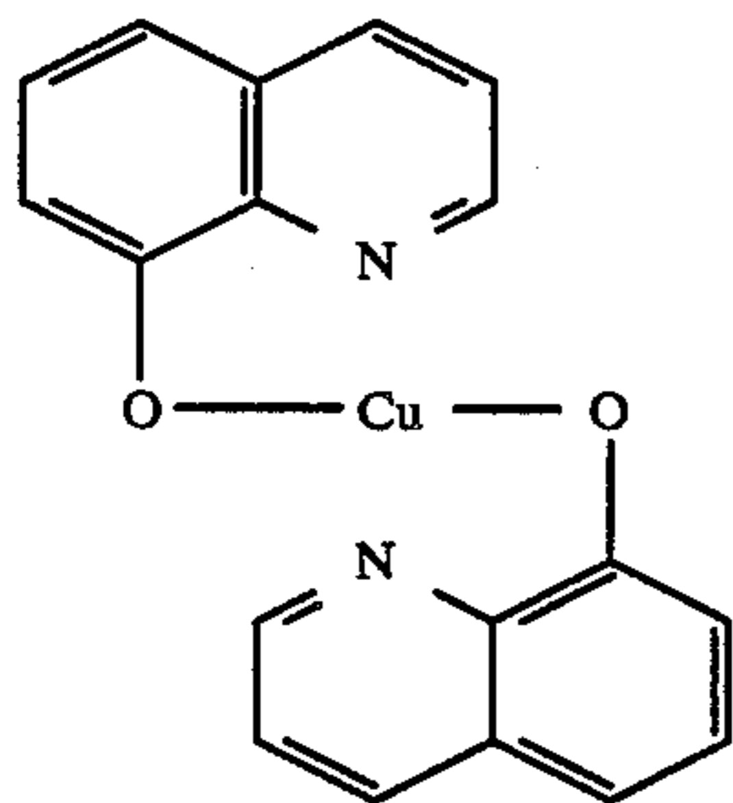
(COPPER OXINATE)
