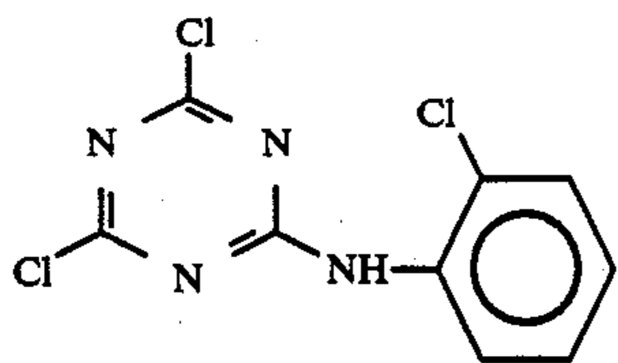
(ANILAZINE)
