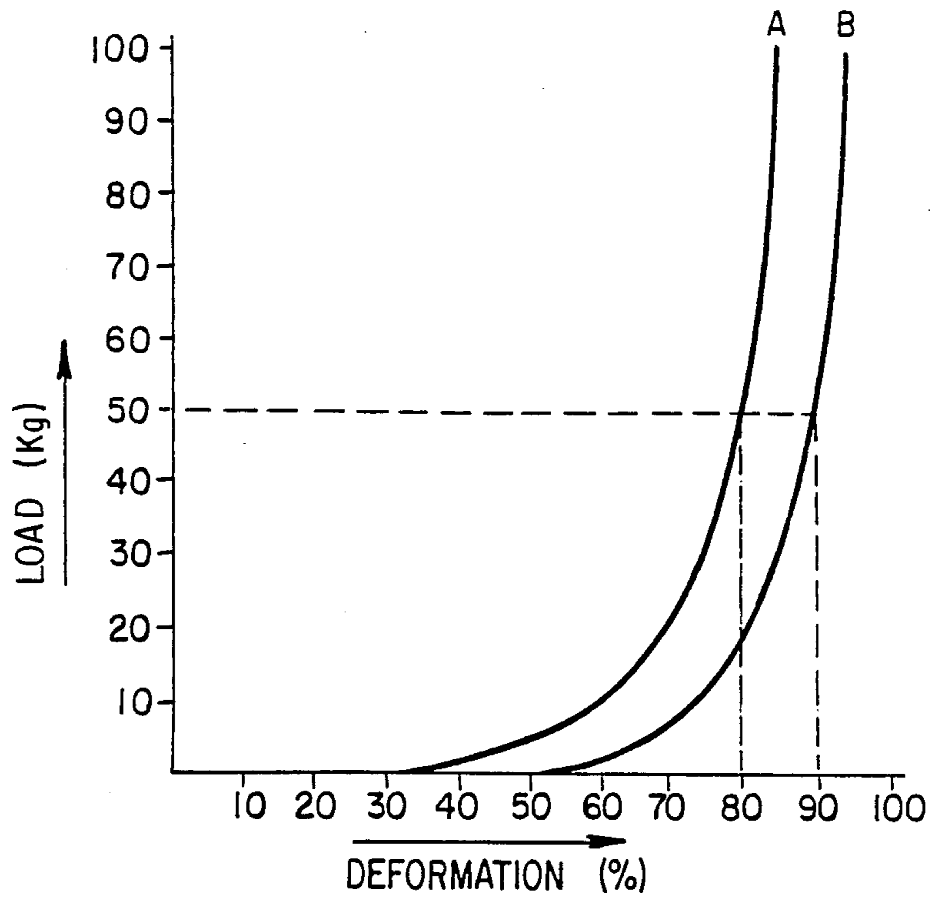
FIG. 12 LOAD DEFORMATION
