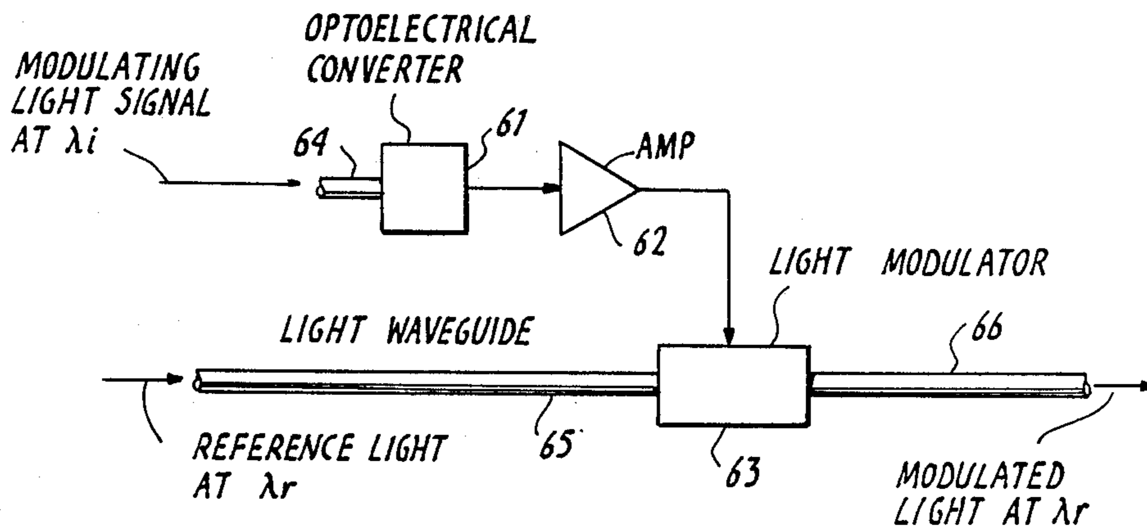
WAVELENGTH CONVERTER
