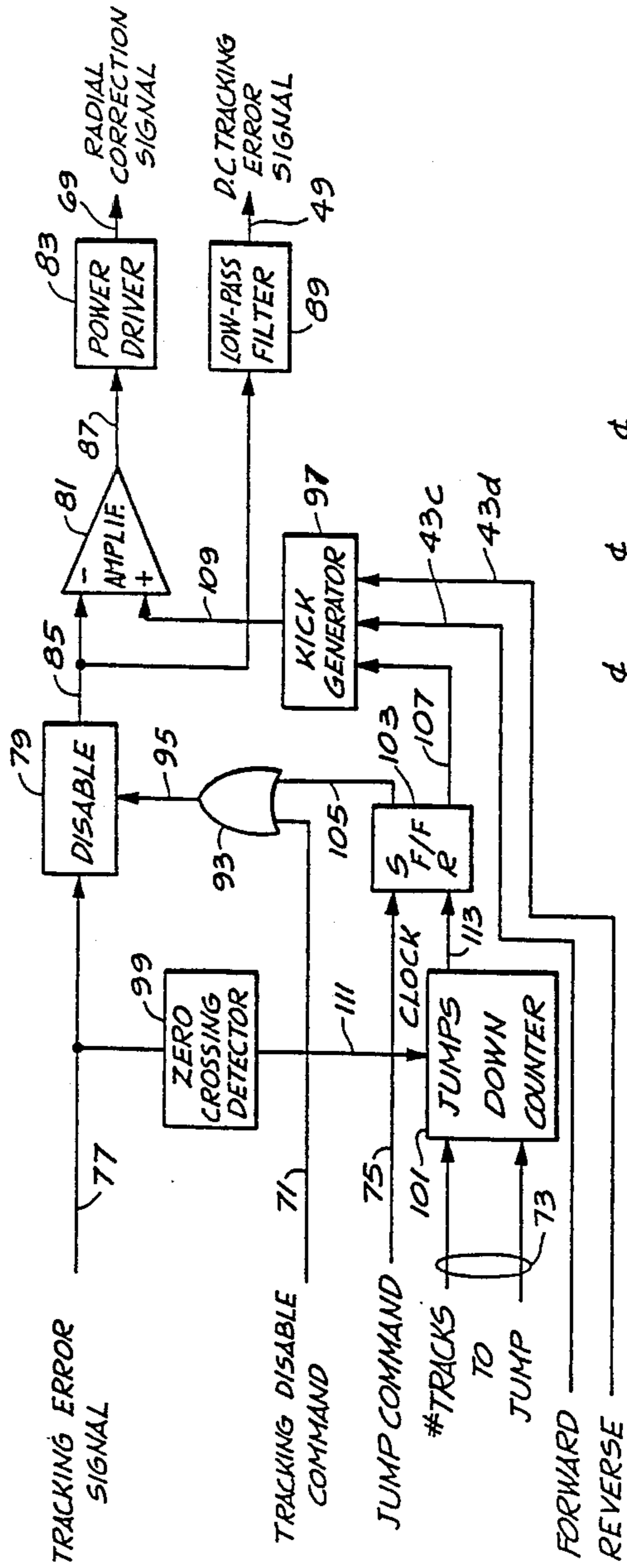
TRACKING CONTROLLER (67)
