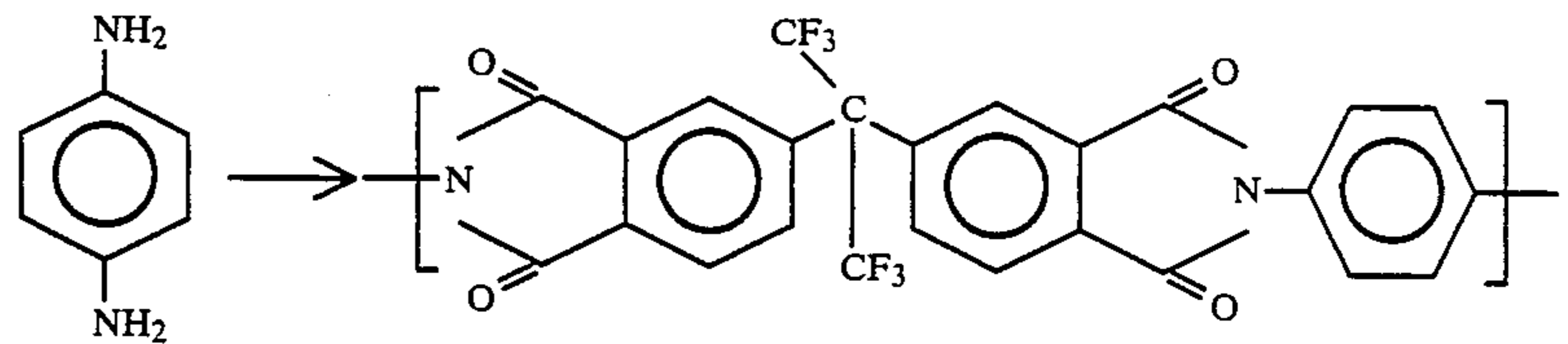
paraphenylenediamine
