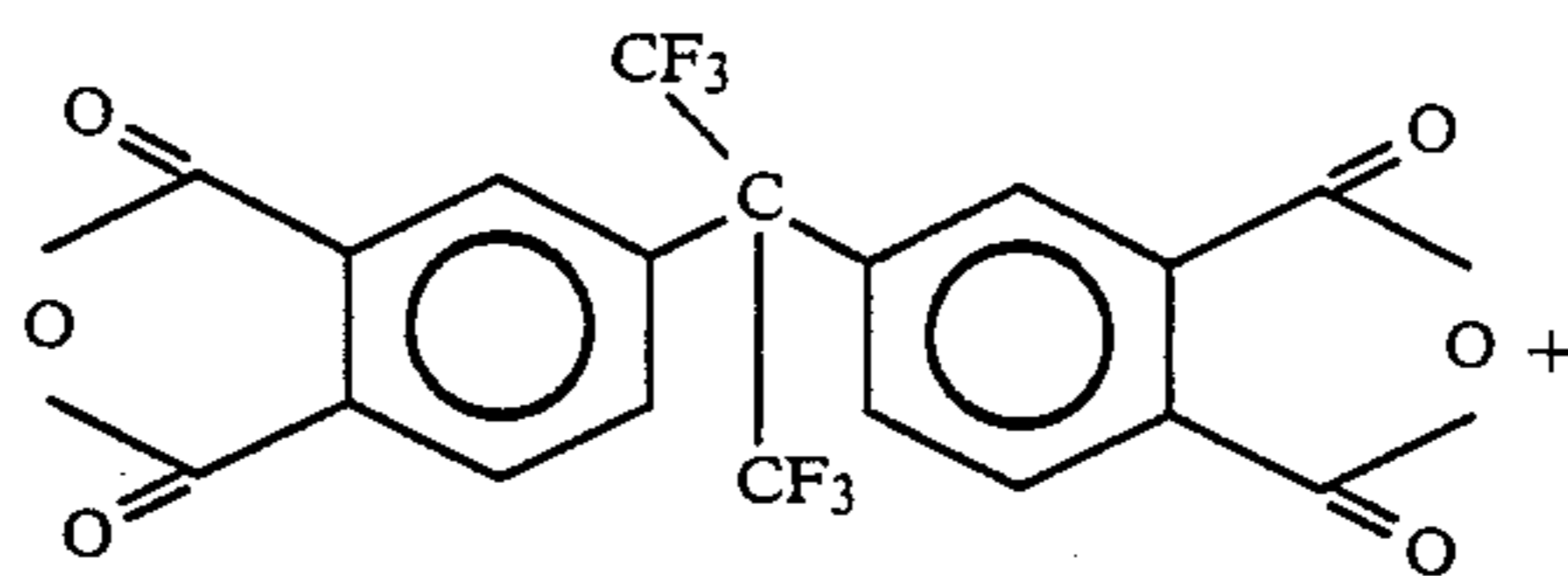
6F Dianhydride
