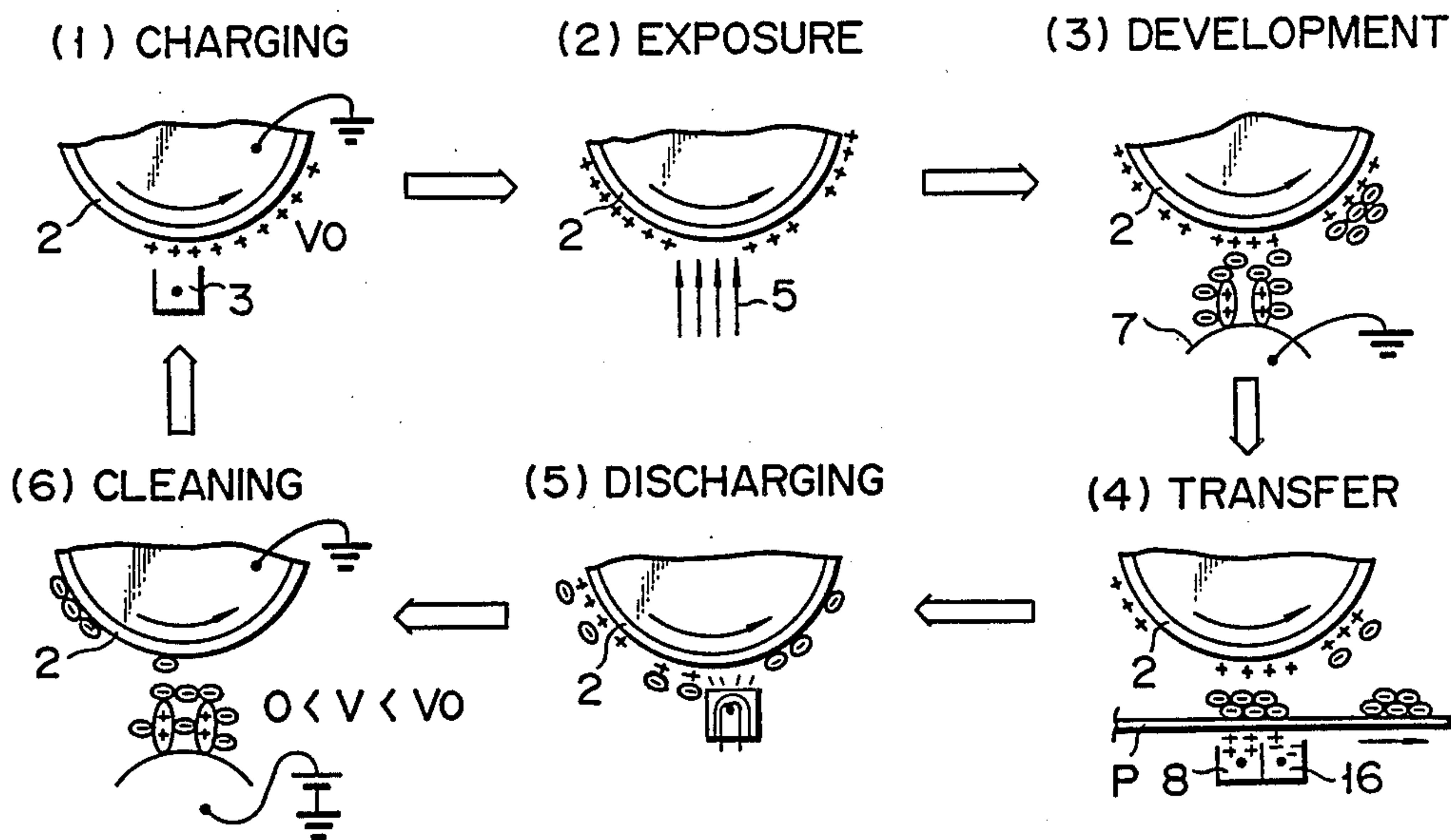
FIG. 4 (PRIOR ART)
