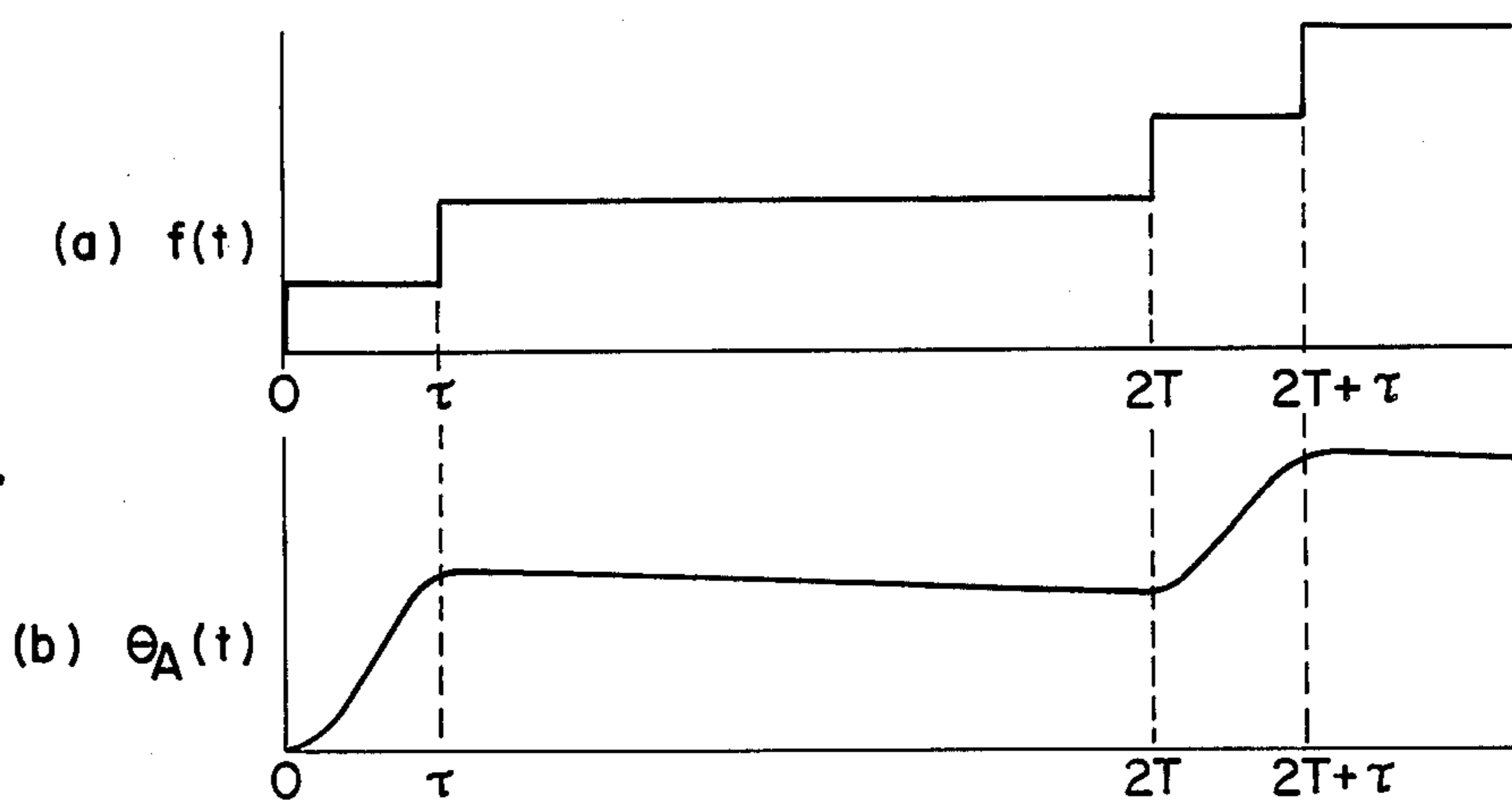
FIG. 2. (PRIOR ART)
