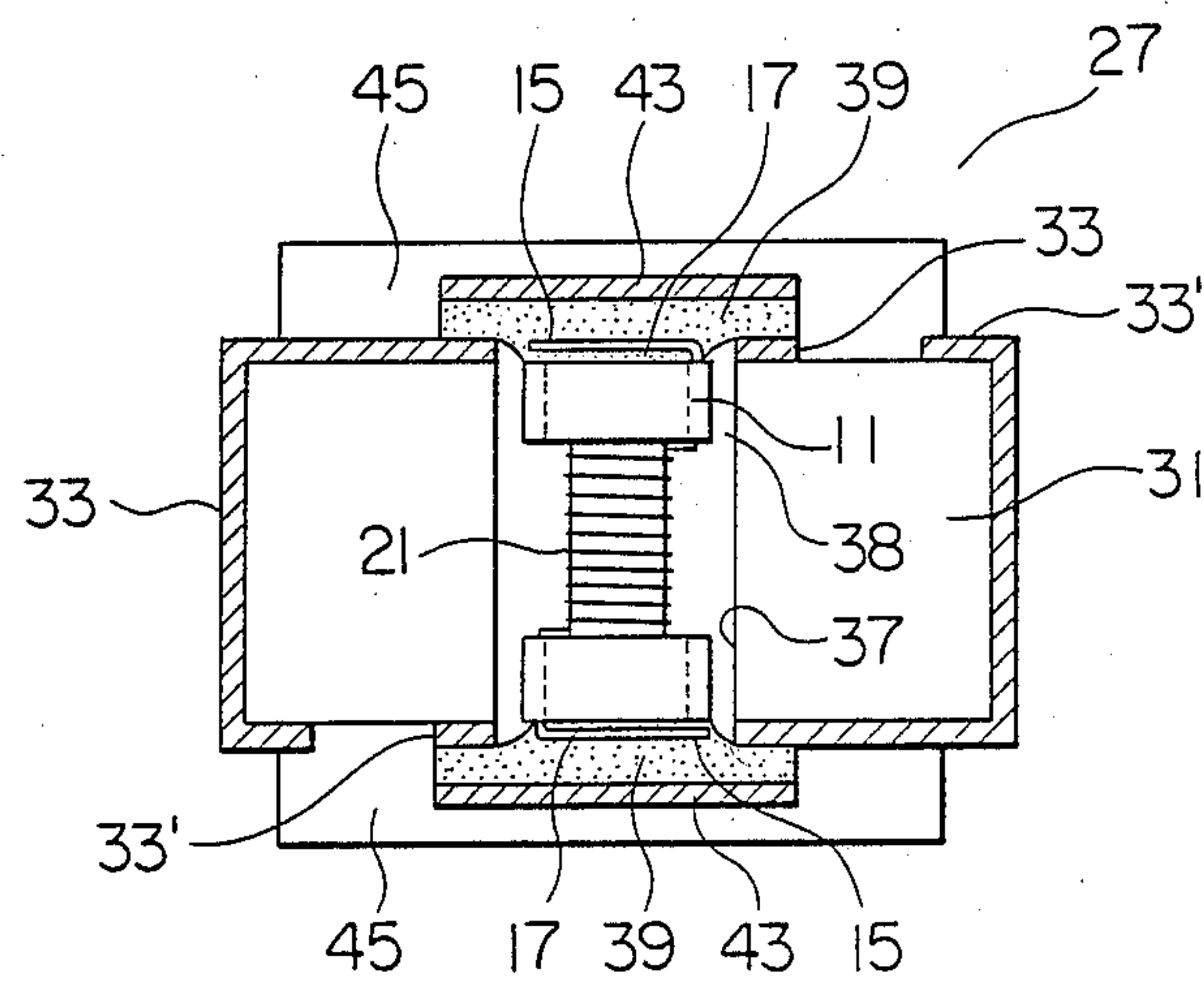
FIG. 8 Prior Art
