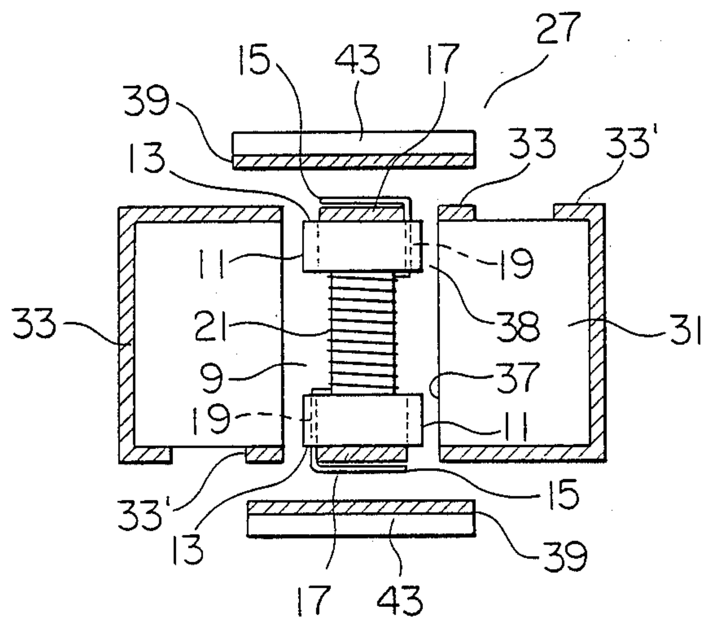
FIG. 7 Prior Art
