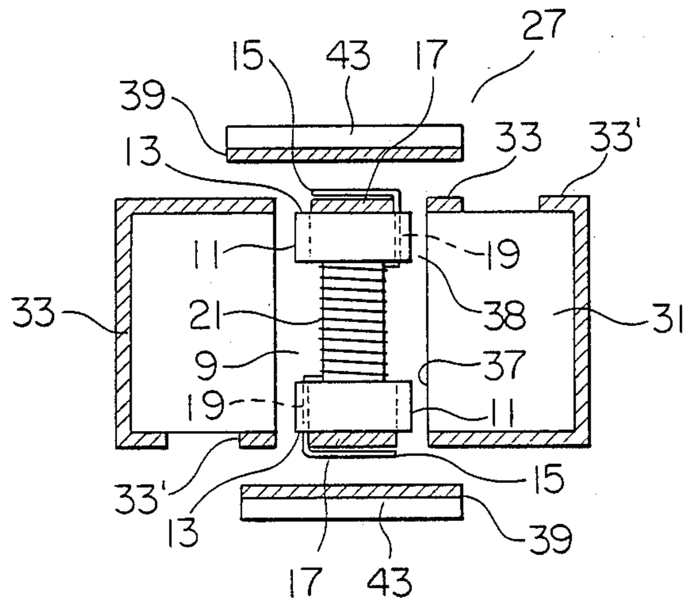
FIG. 7 Prior Art
