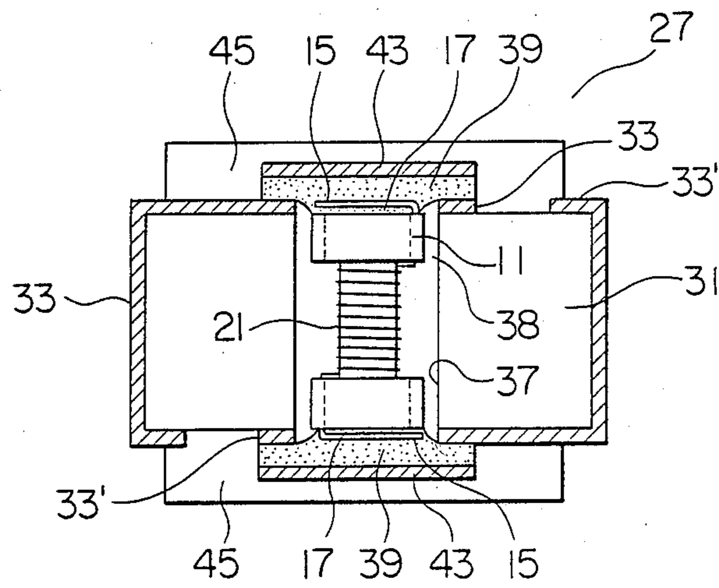
FIG. 8 Prior Art
