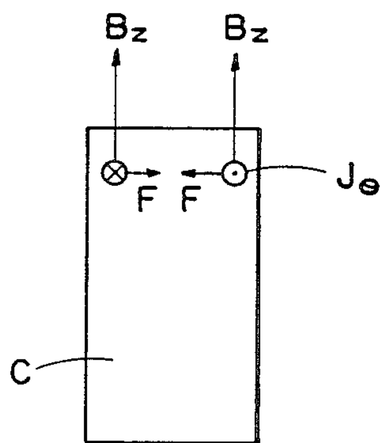
FIG. 5 (PRIOR ART)
