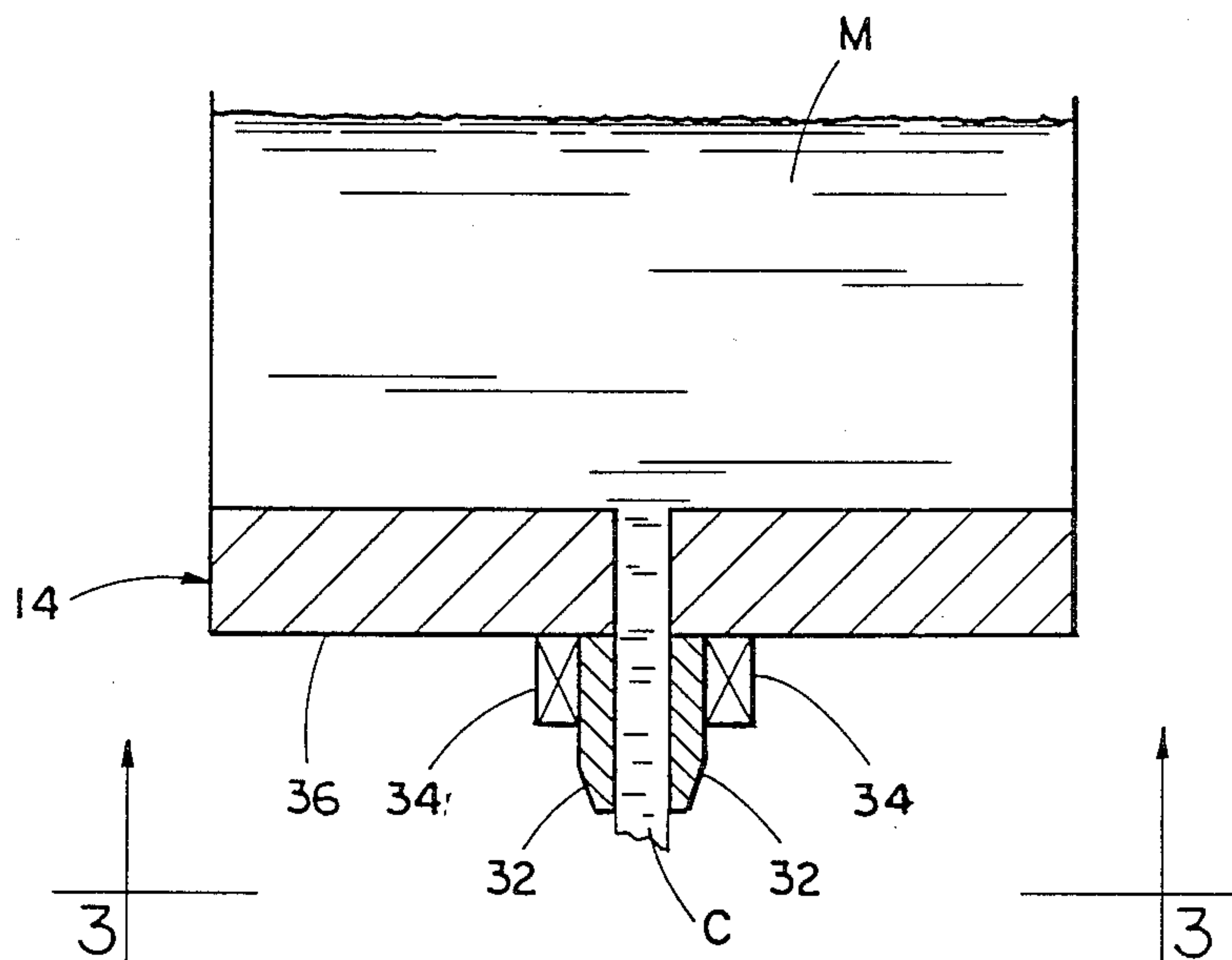
FIG 2 (PRIOR ART)
