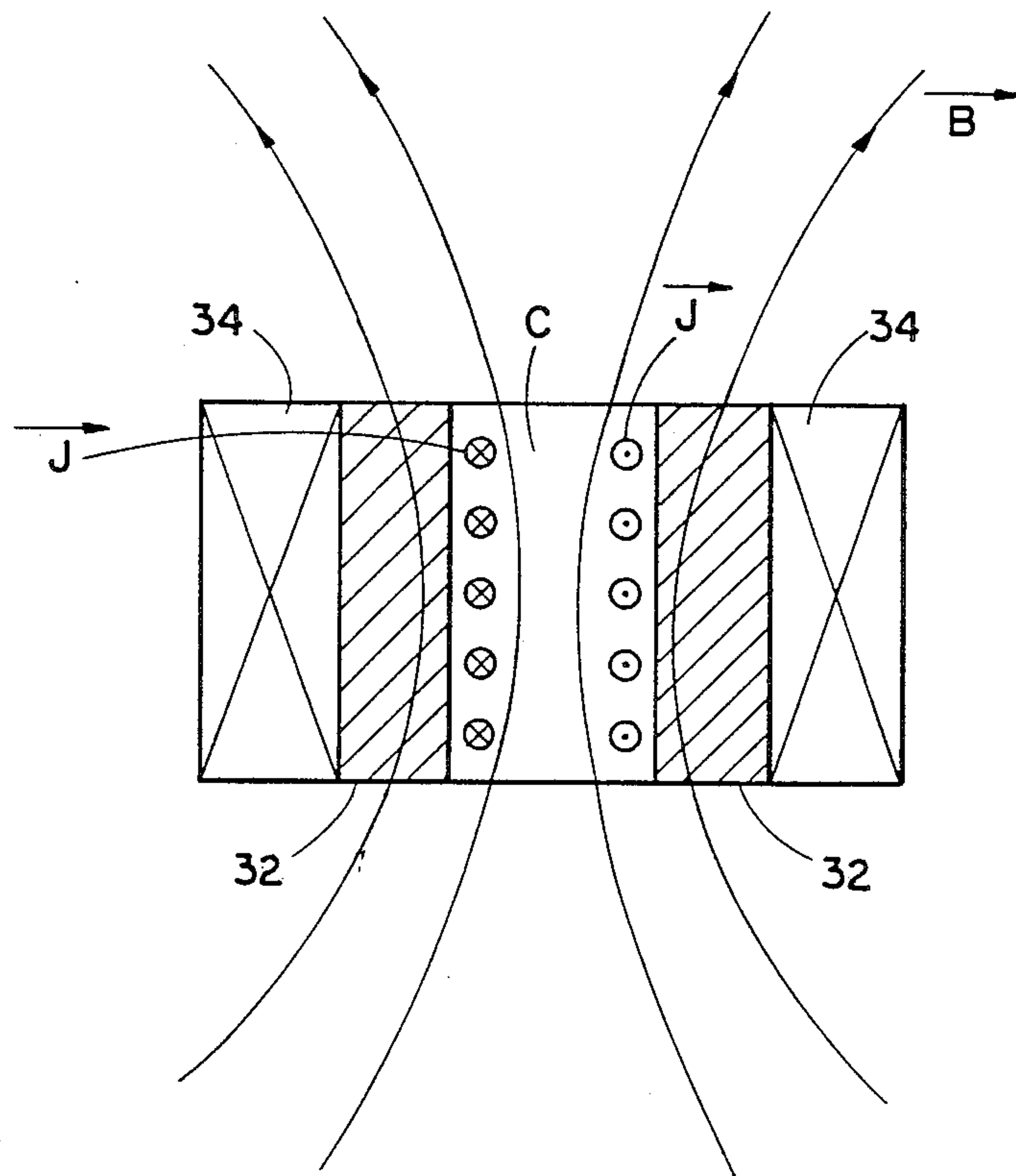
FIG. 4 (PRIOR ART)
