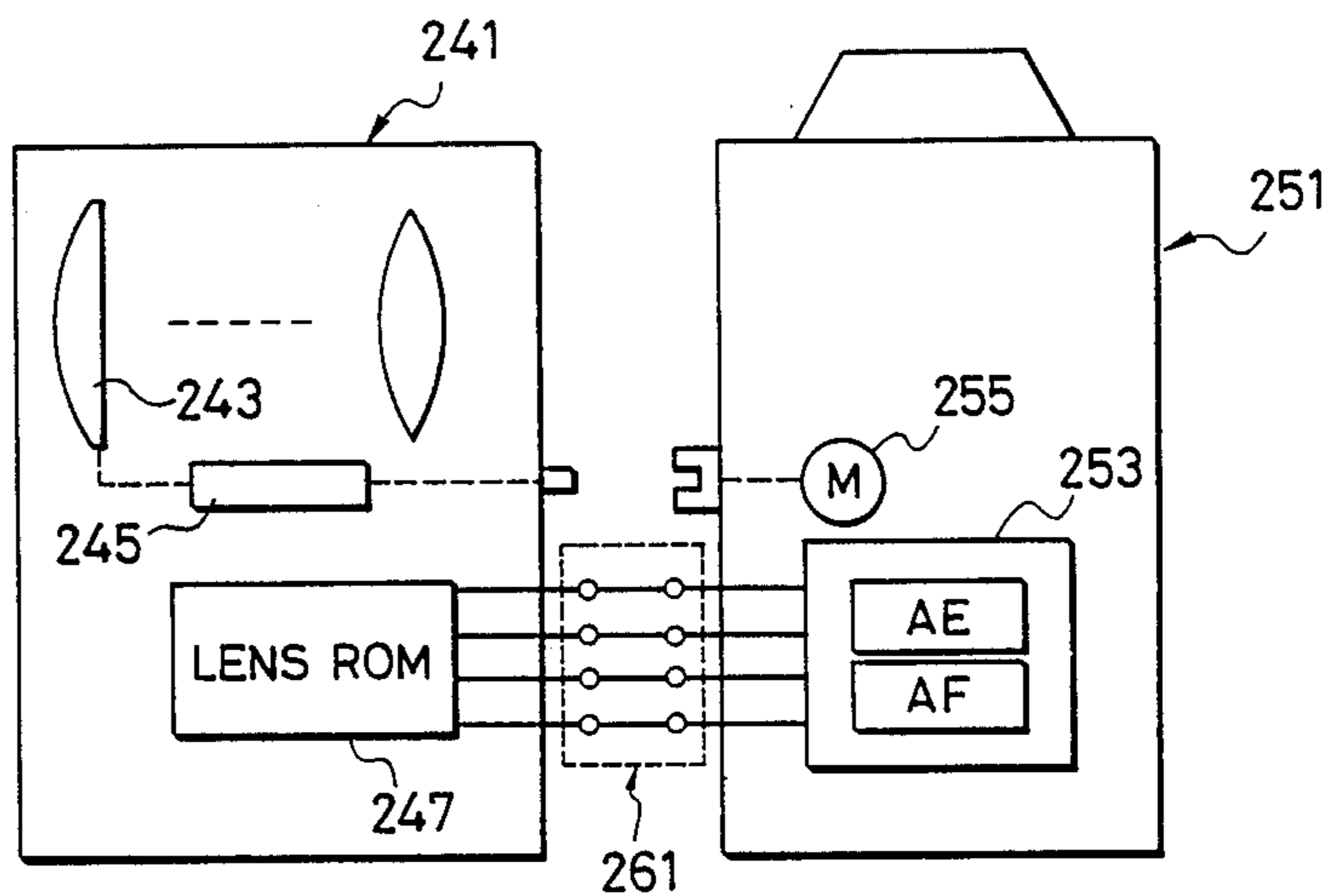
FIG. 5 PRIOR ART
