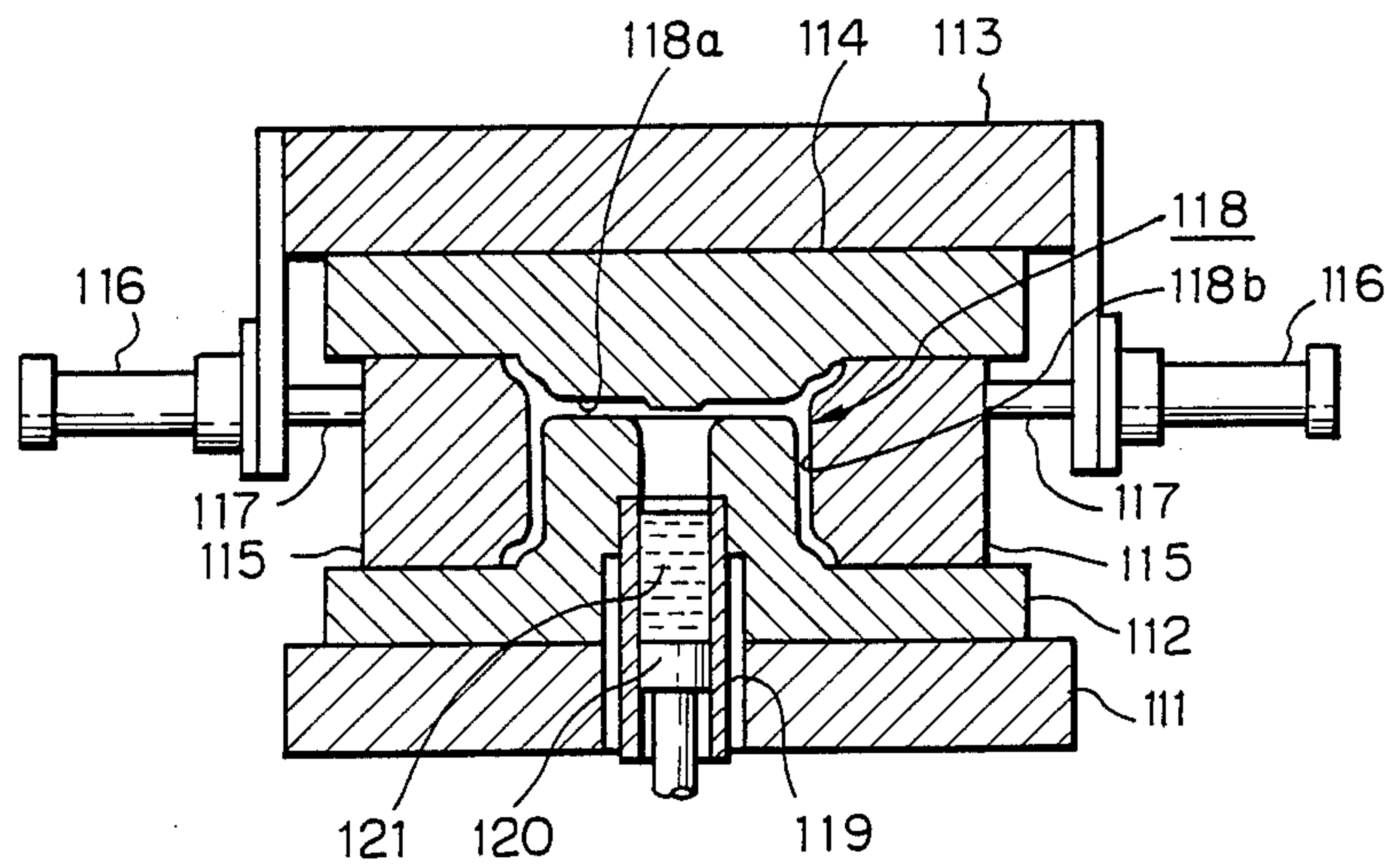
Fig. 6 PRIOR ART
