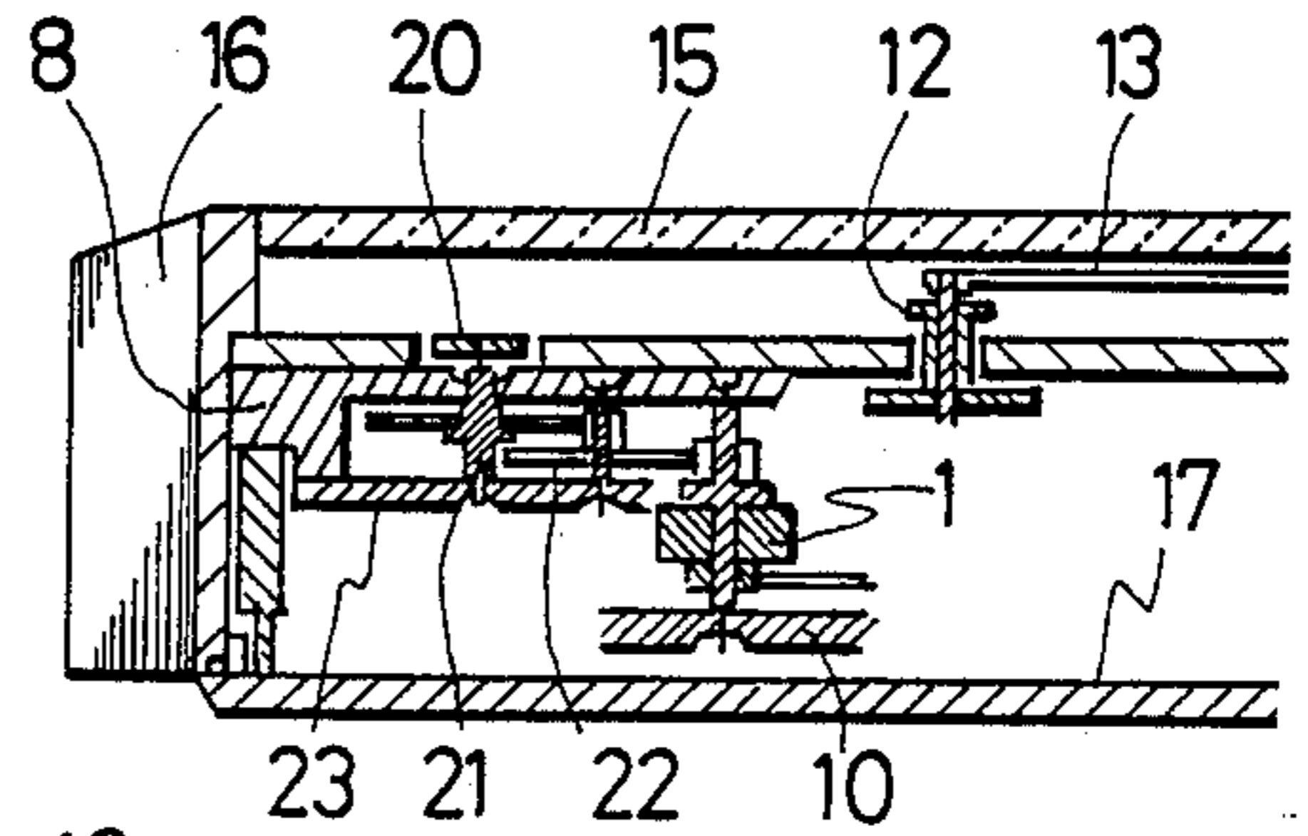
FIG. 24 PRIOR ART
