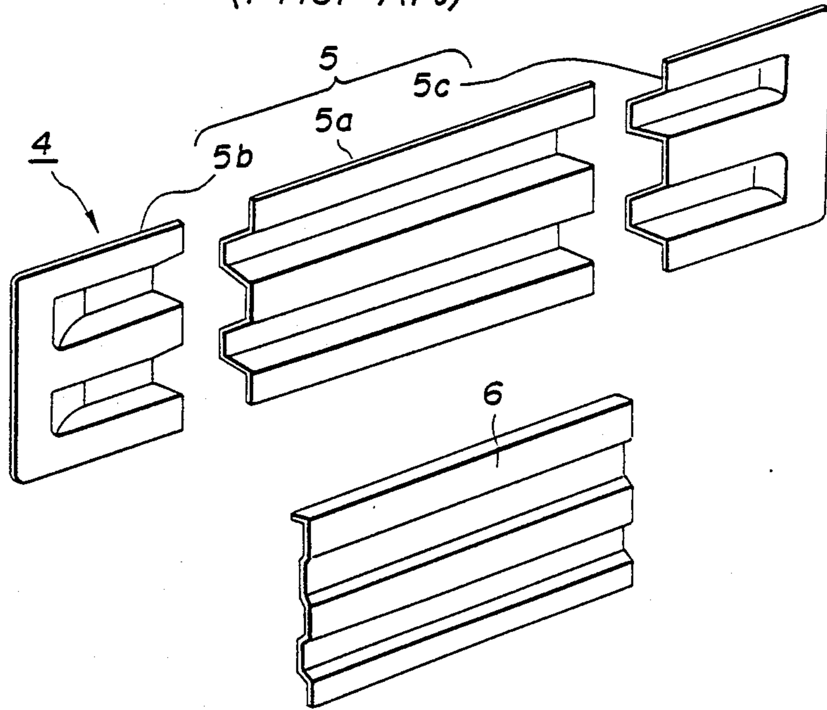
FIG. 16 (Prior Art)
