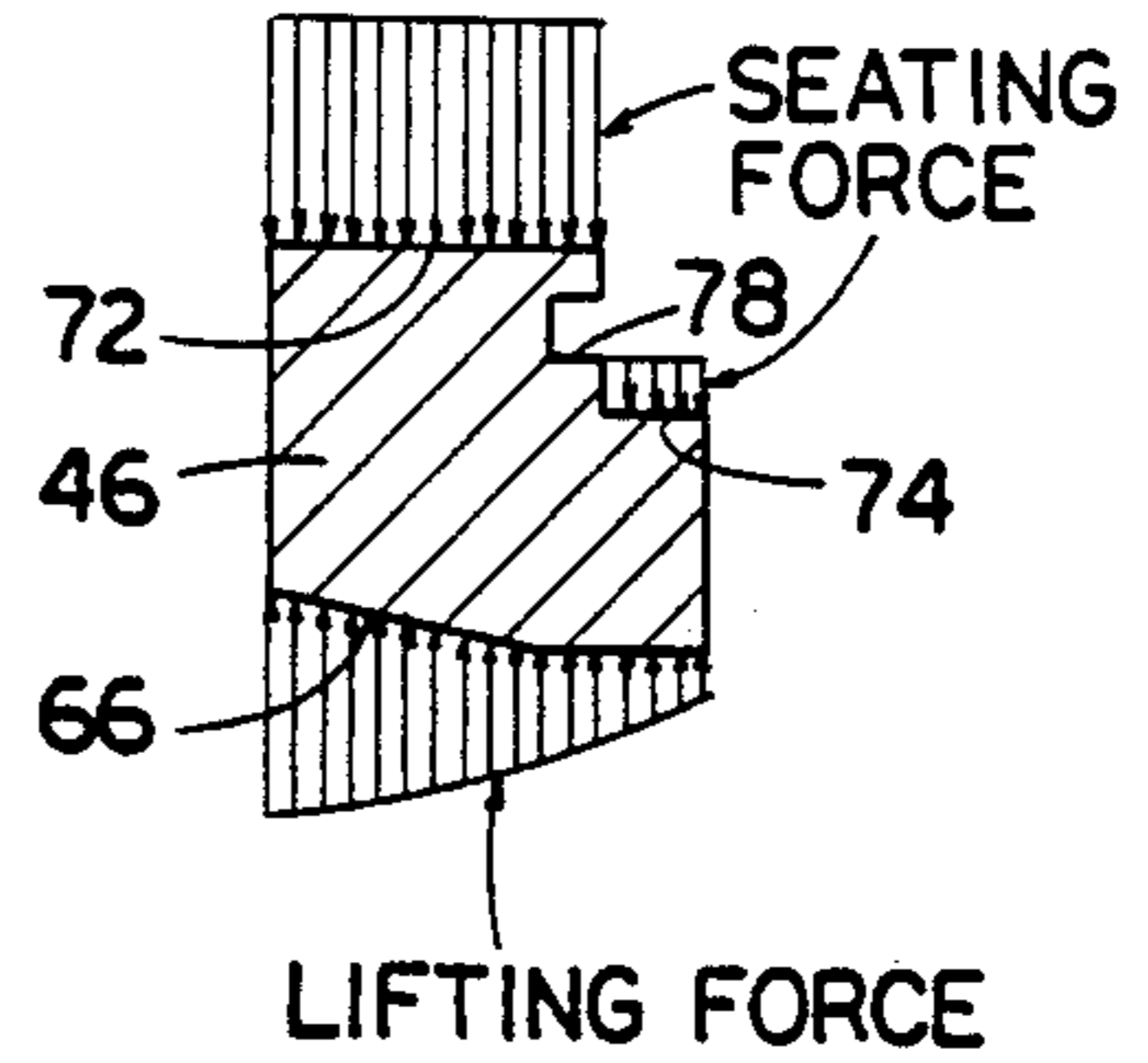
FIG. 9 (PRIOR ART)
