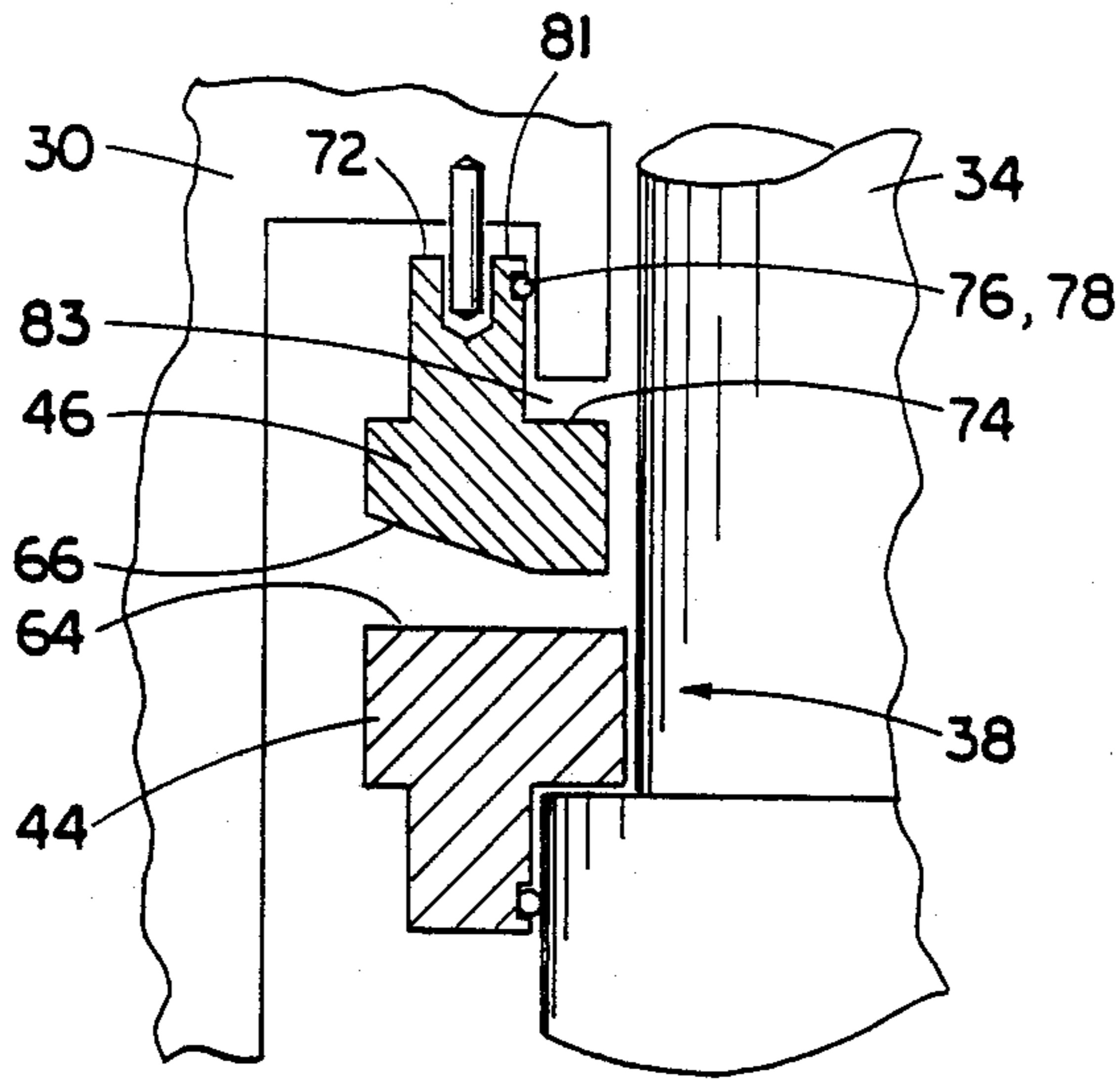
FIG. 8 (PRIOR ART)
