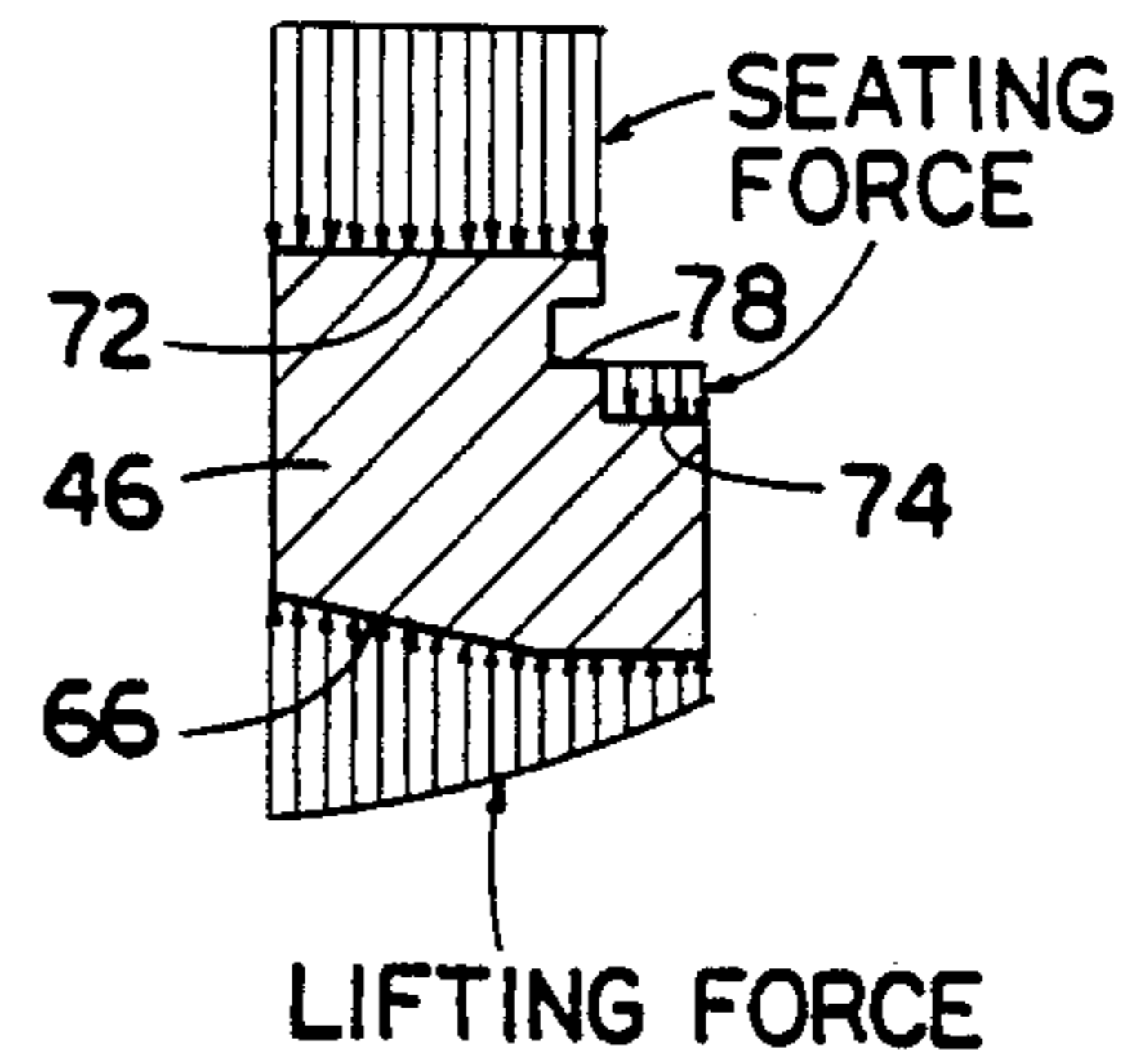
FIG. 9 (PRIOR ART)
