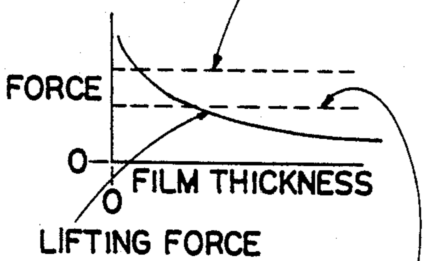
SEATING FORCE WITH LOW PRESSURE IN SECOND BALANCE CHAMBER
