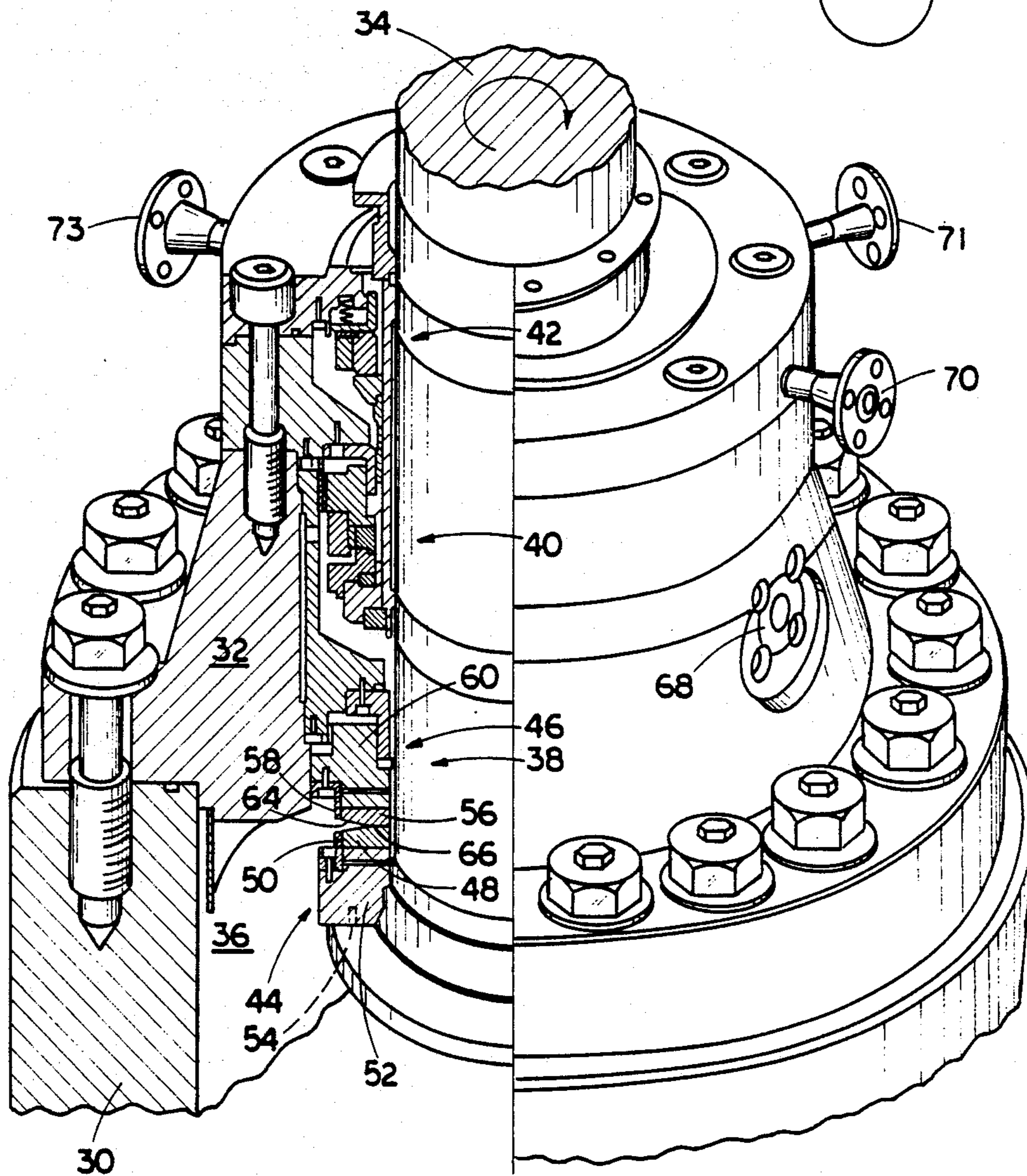
FIG 2 (PRIOR ART)
