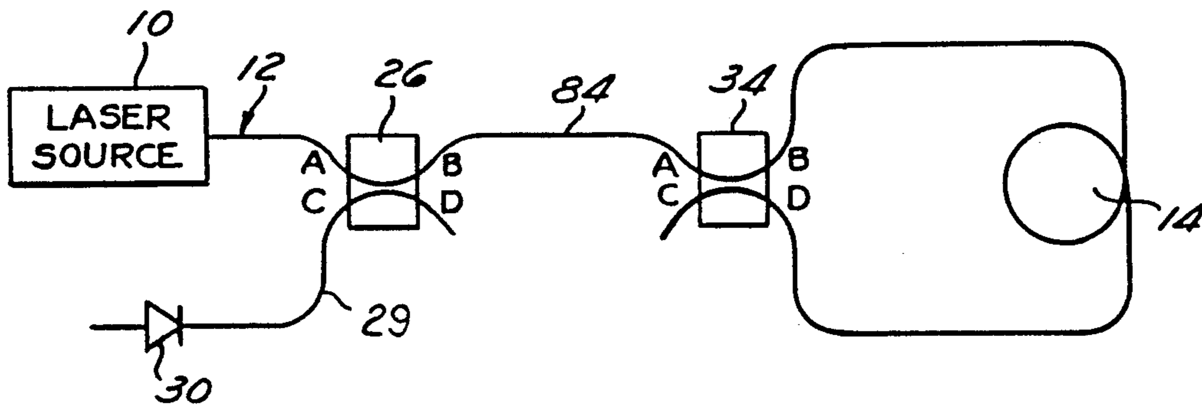
Fig. 5 (PRIOR ART)
