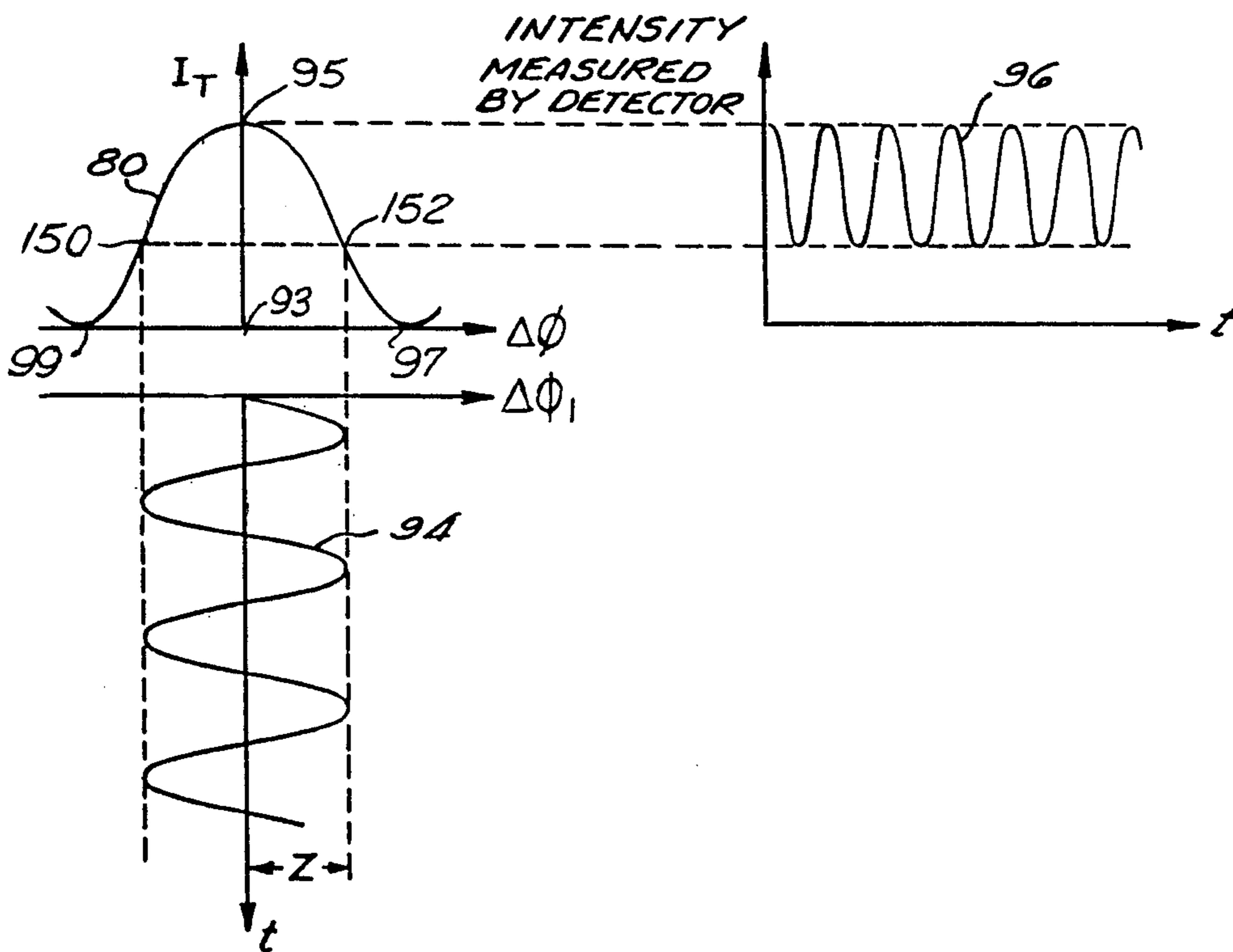
Fig. 8 (PRIOR ART)
