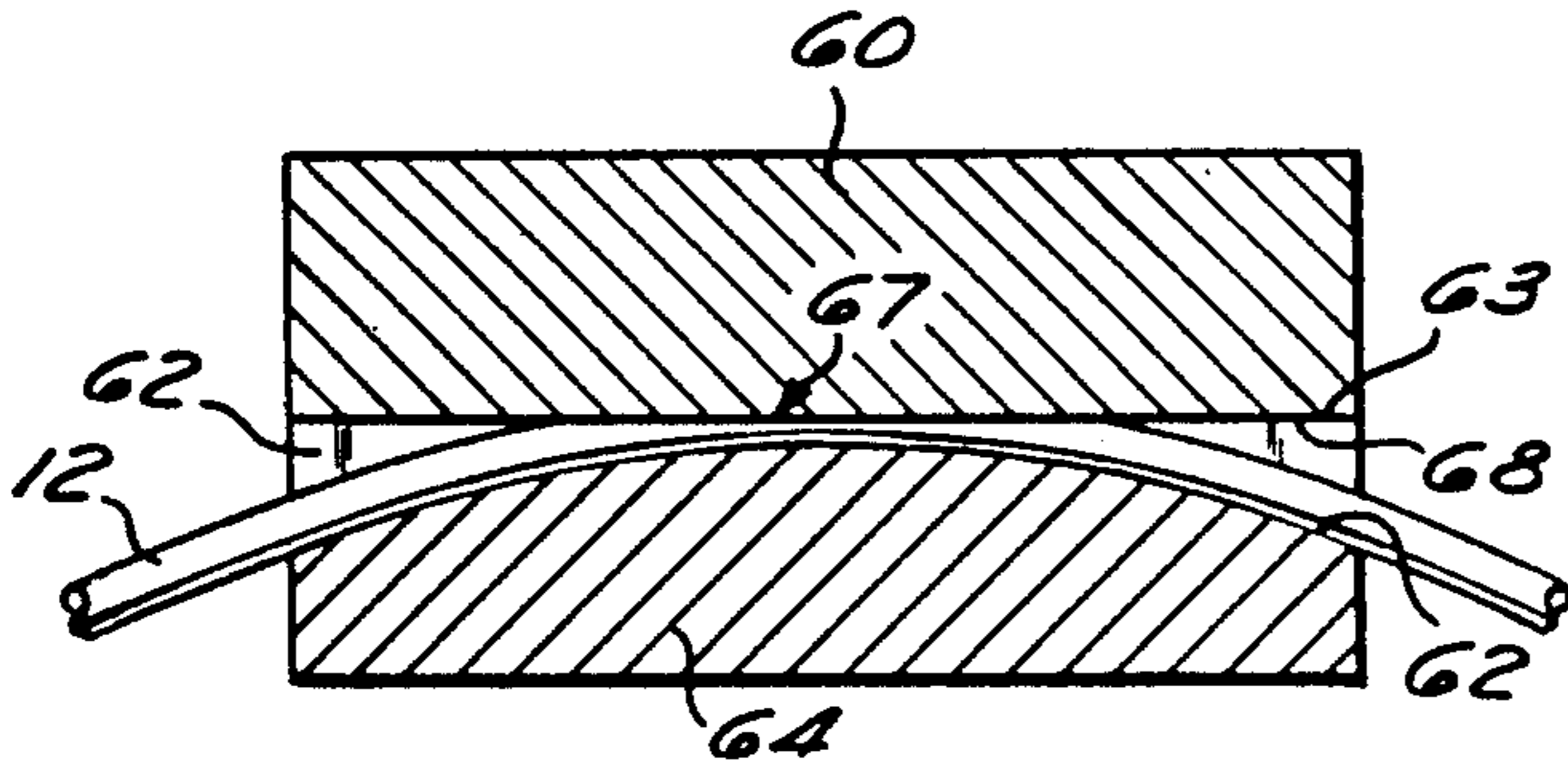
Fig. 3 (PRIOR ART)
