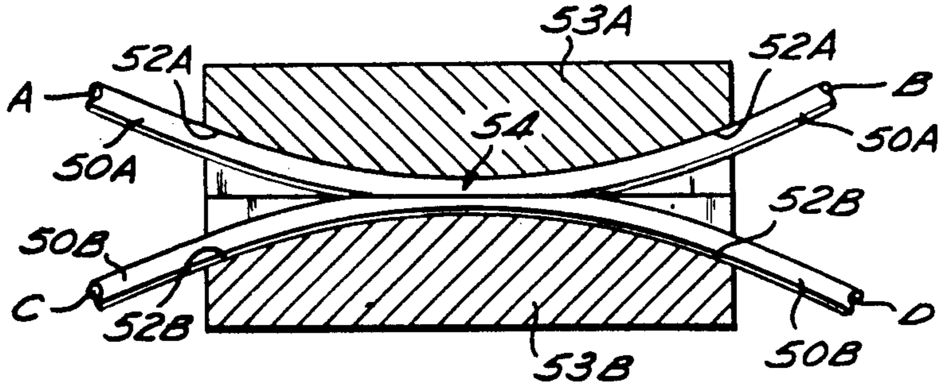
Fig. 2 (PRIOR ART)
