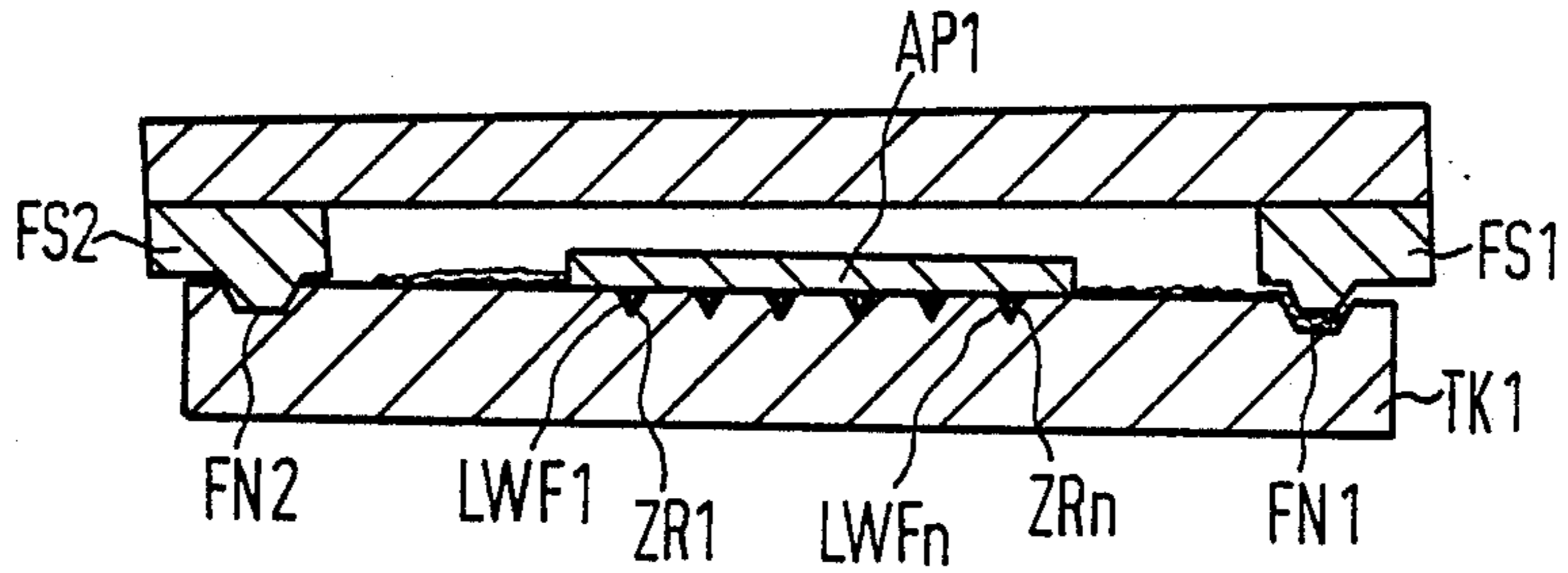
FIG2 (PRIOR ART)
