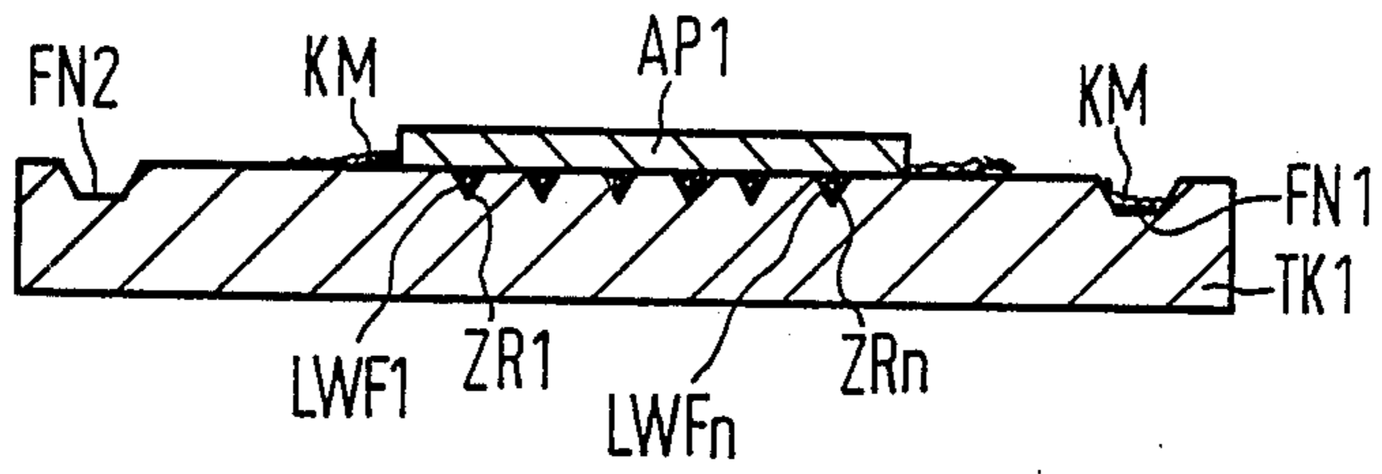
FIG1 (PRIOR ART)
