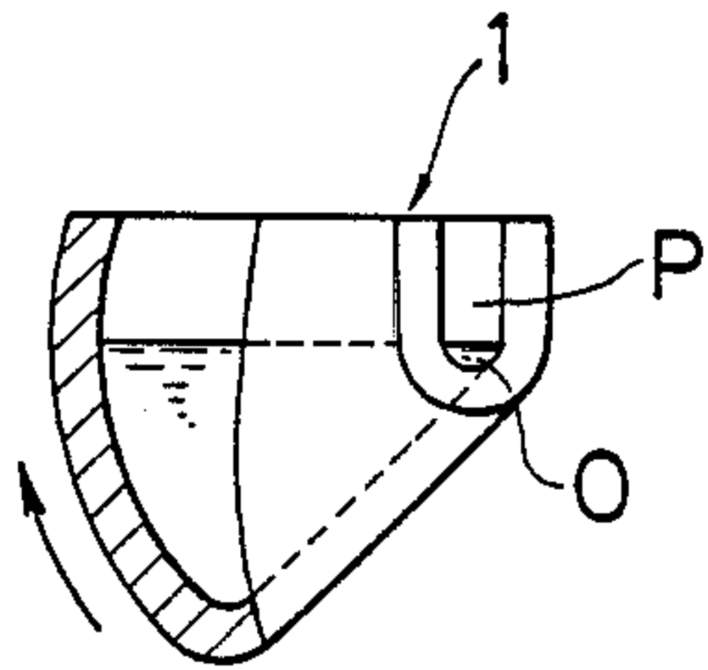
FIG. 10 PRIOR ART
