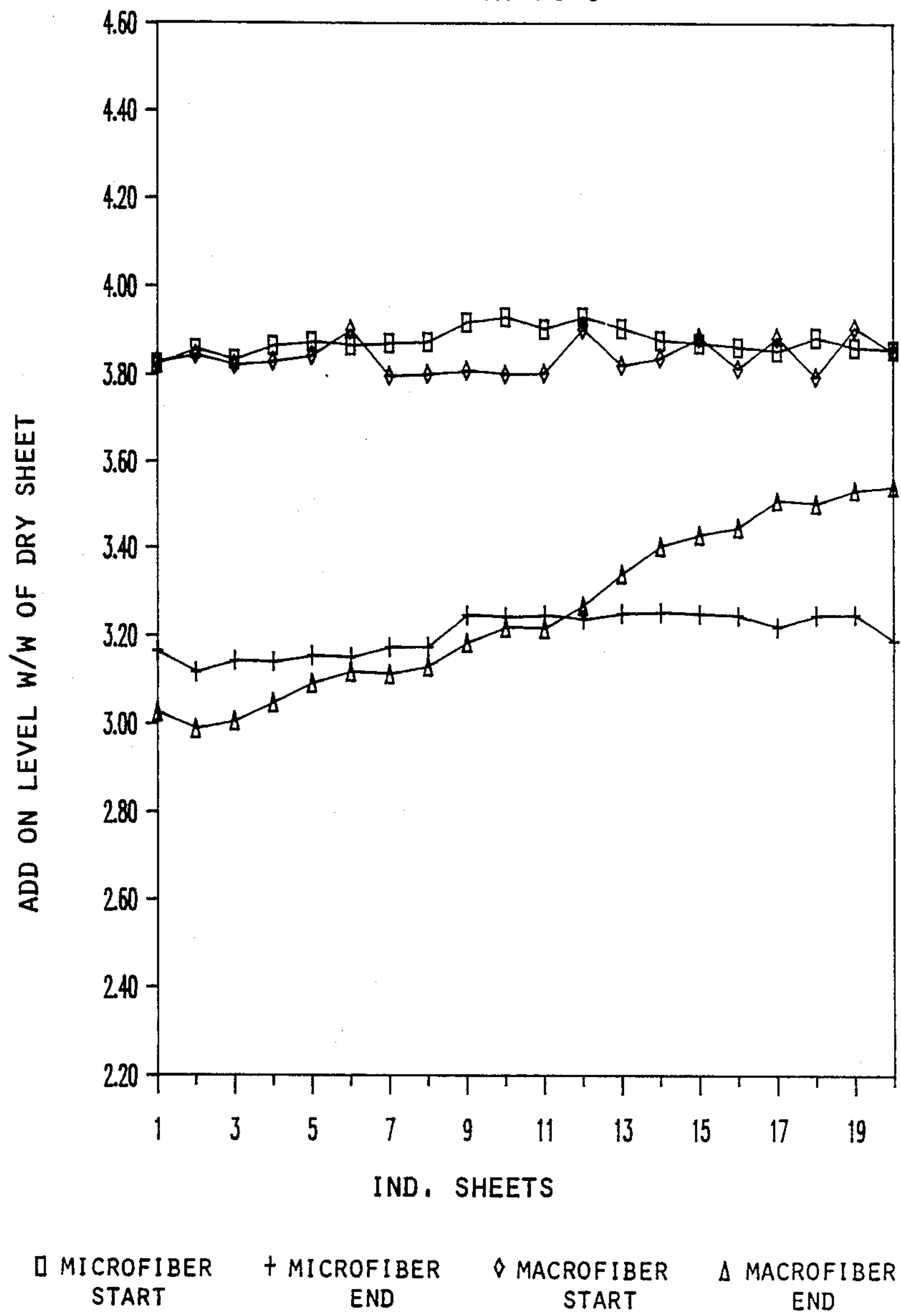
Figure 2F Liquid Retention 1 MONTH AT 50°C
