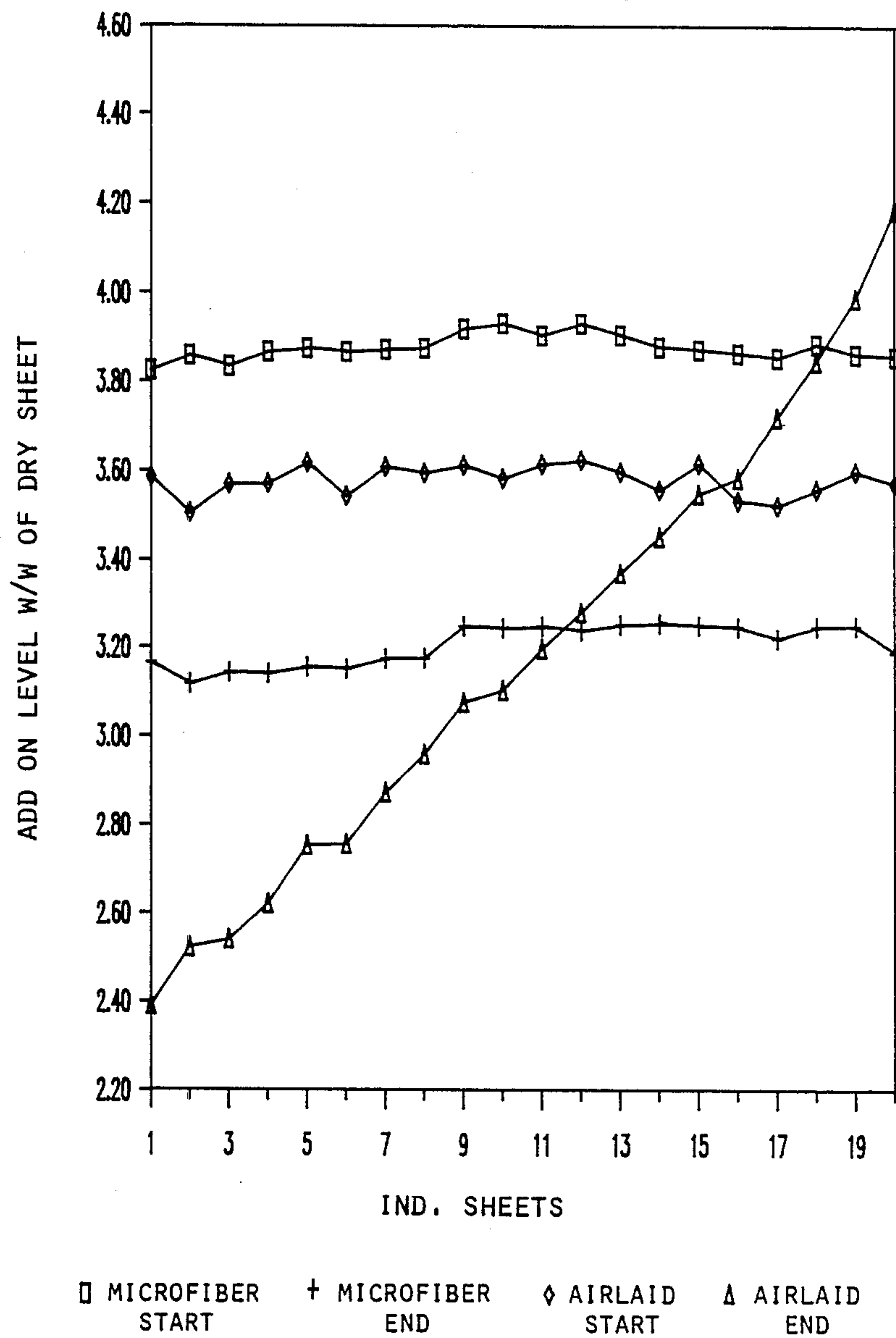
Figure 2E Liquid Retention 1 MONTH AT 50°C
