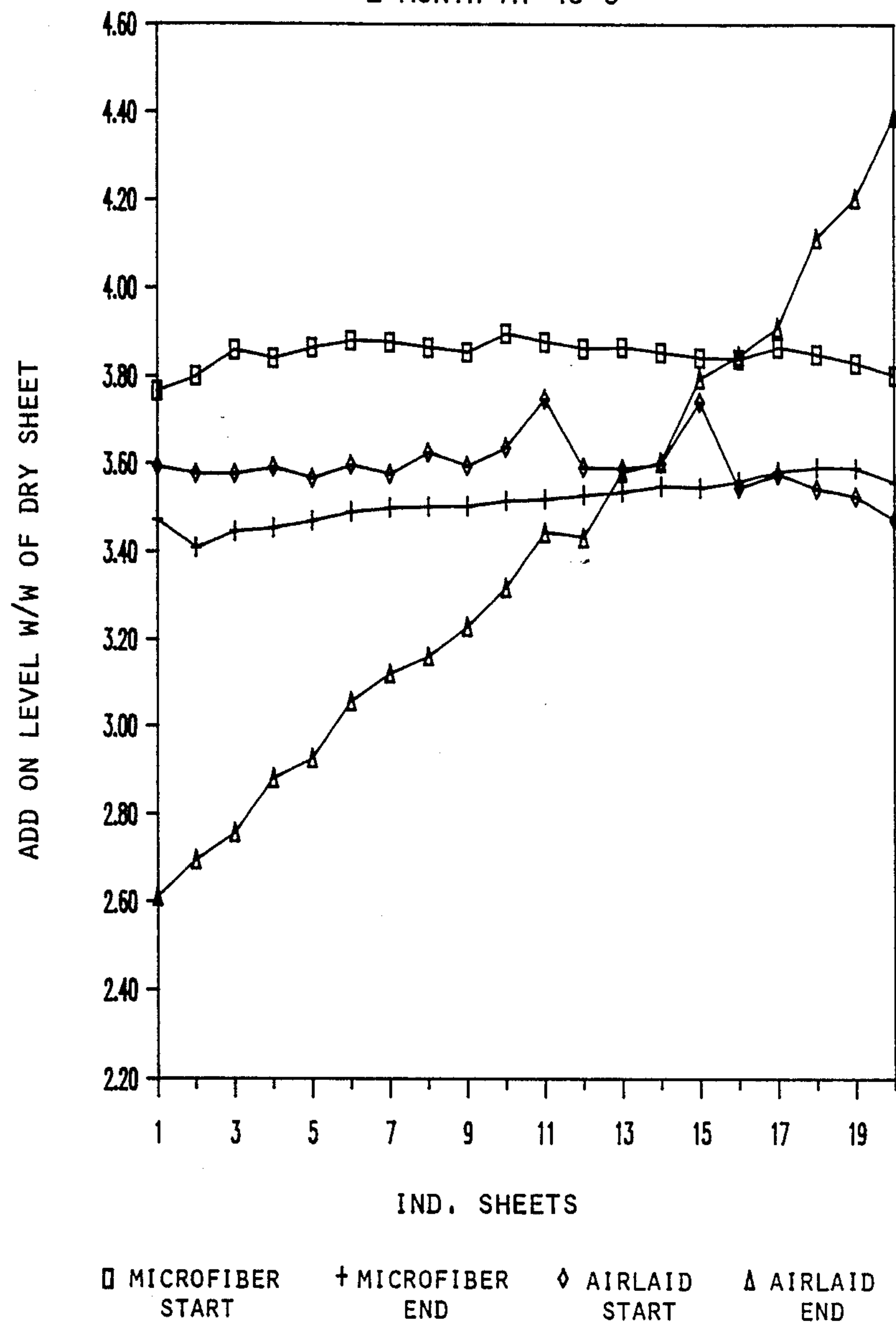
Figure 2C Liquid Retention 1 MONTH AT 40°C
