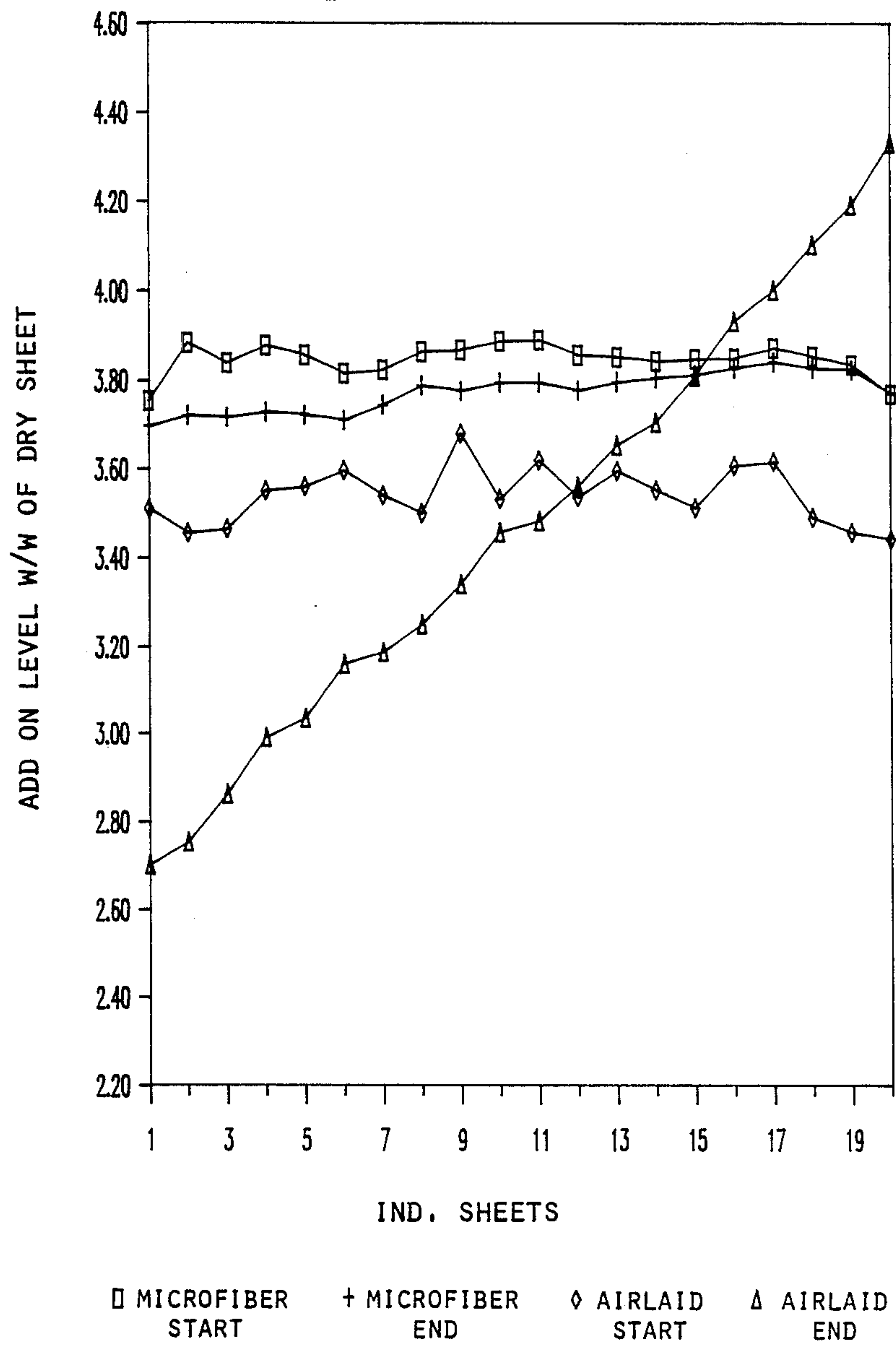
Figure 2A Liquid Retention 1 MONTH AT ROOM TEMP.
