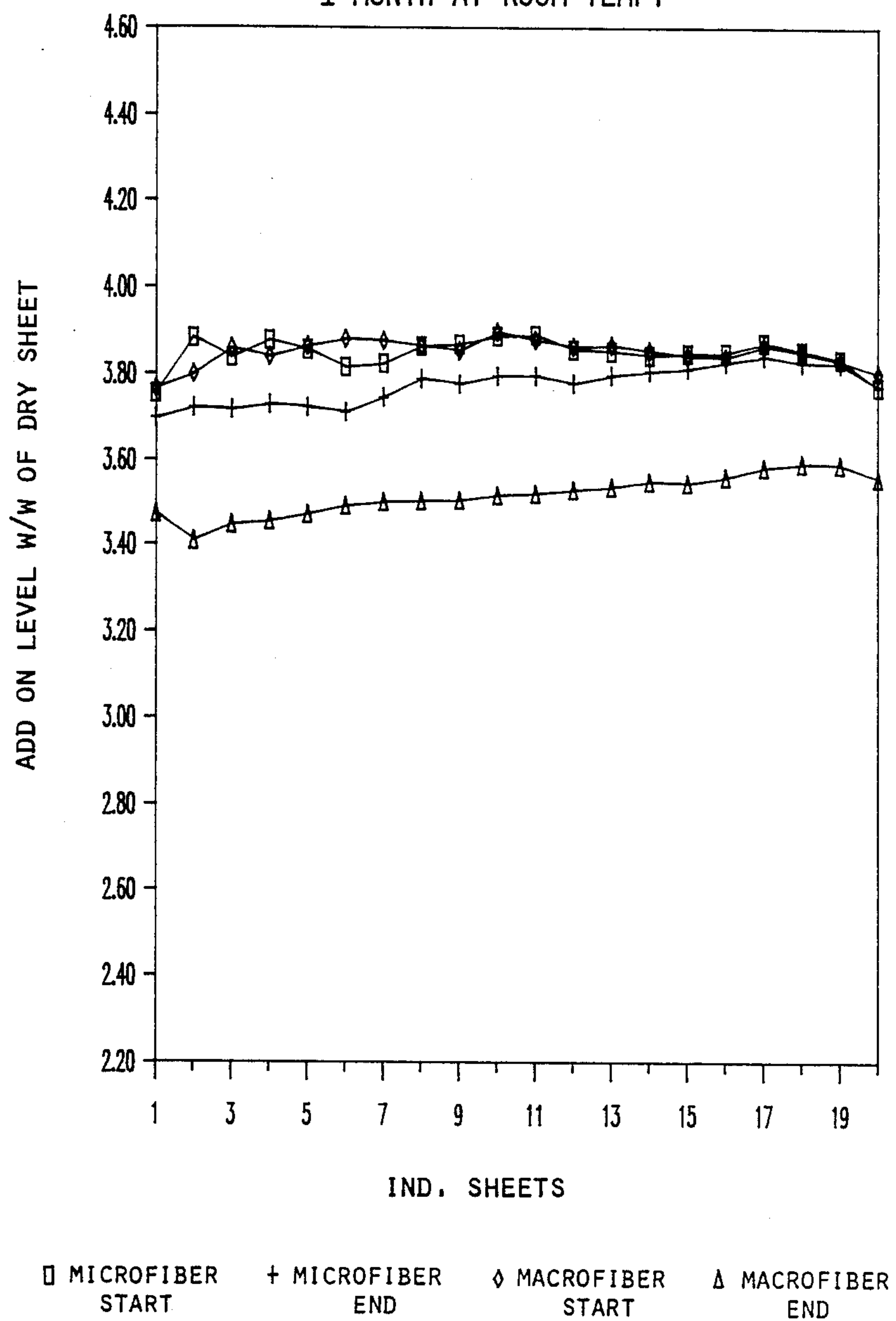
Figure 2B Liquid Retention 1 MONTH AT ROOM TEMP.
