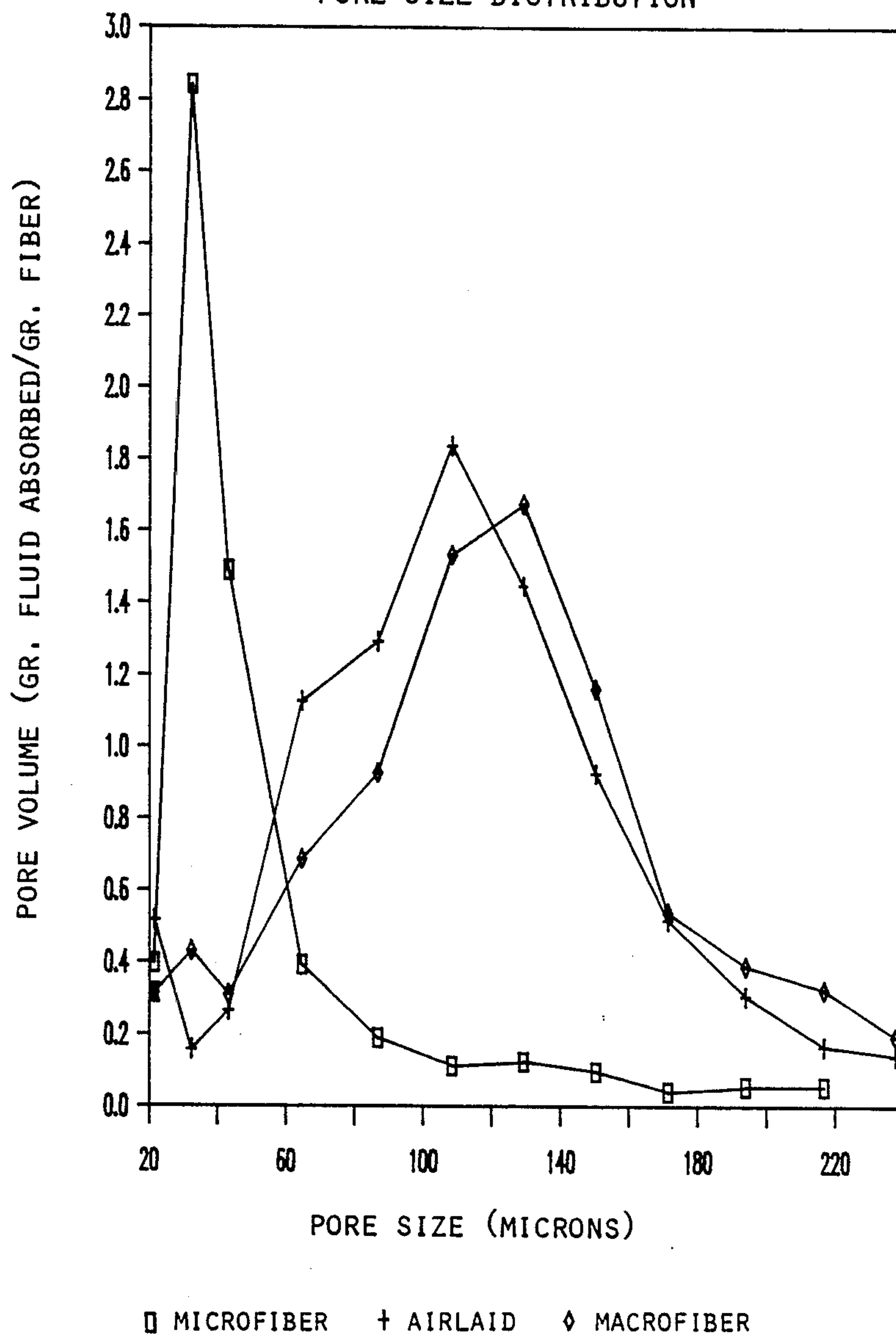
Figure 1 PORE SIZE DISTRIBUTION
