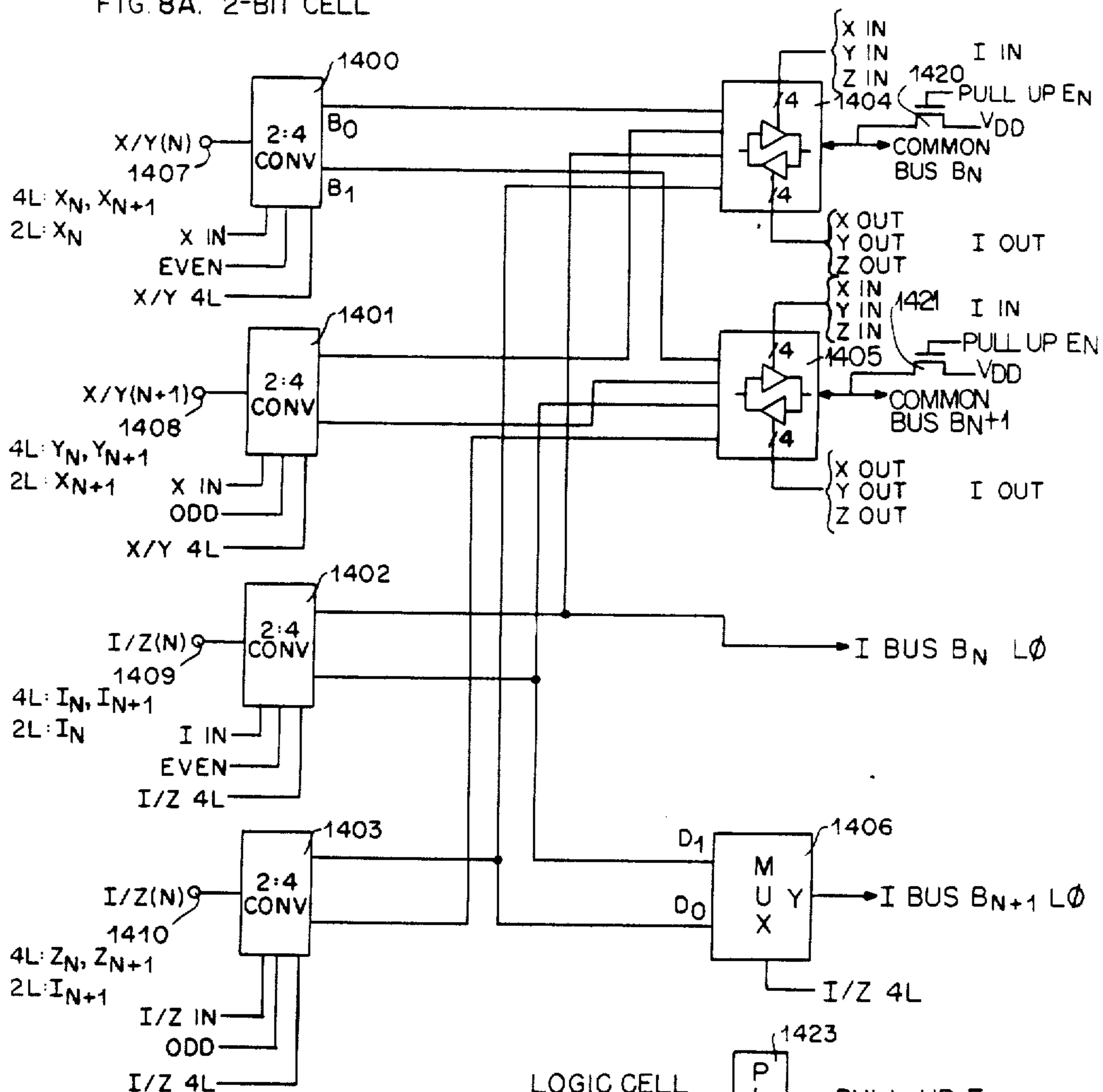
FIG. 8B. COMMON CONTROL LOGIC
