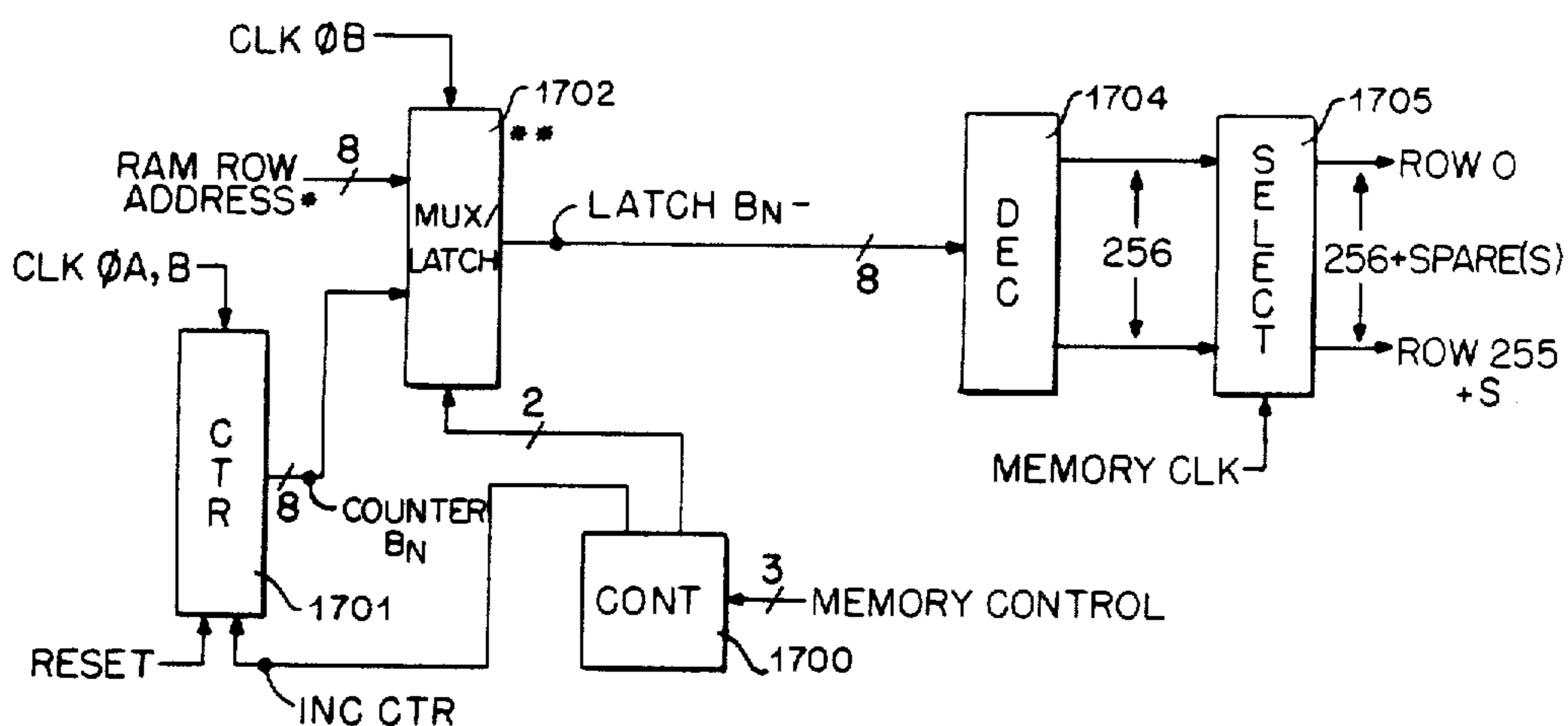
FIG. 10A. BLOCK DIAGRAM
