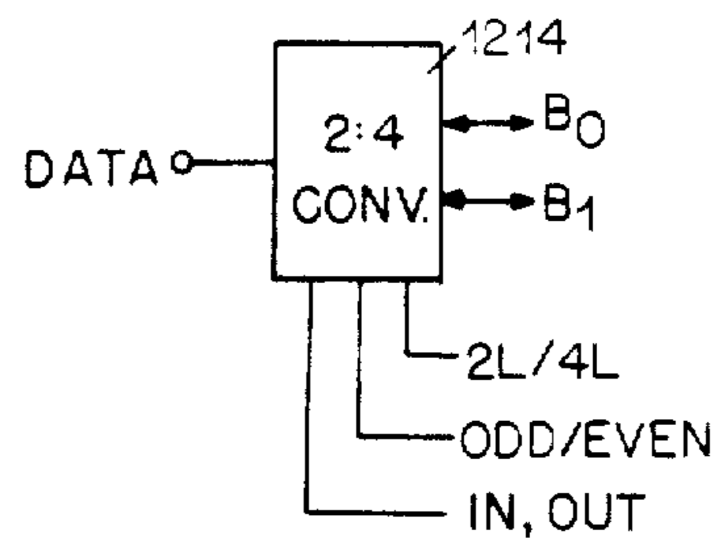
FIG. 7C. 2:4 LEVEL CONVERTER SYMBOL
