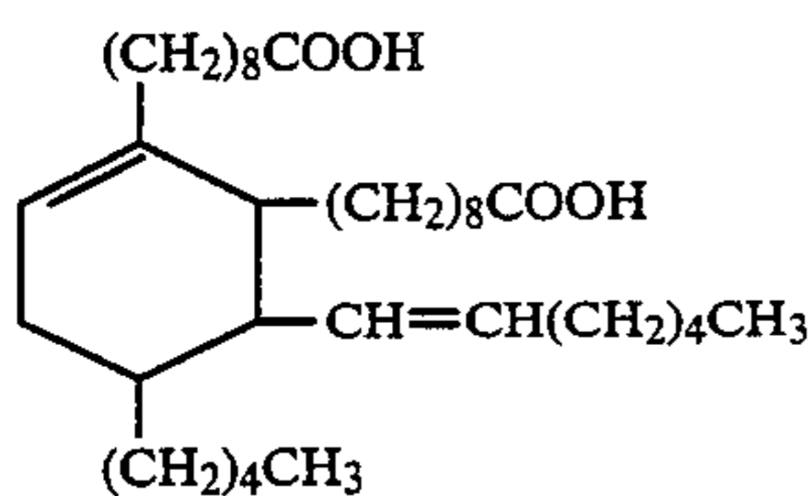
6-(hept-1-enyl)-5-pentyl-3-cyclohexene-1,2-dinonanoic acid
