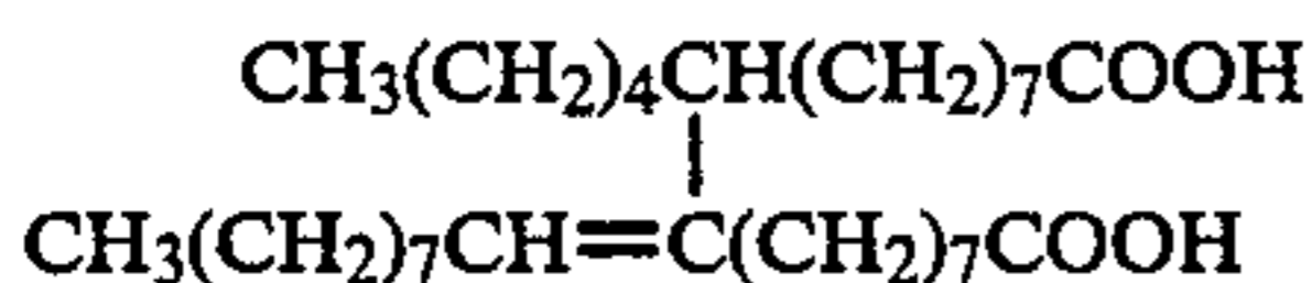
9-nonylidene-10-pentyl-1,18-octadecanedioic acid.
