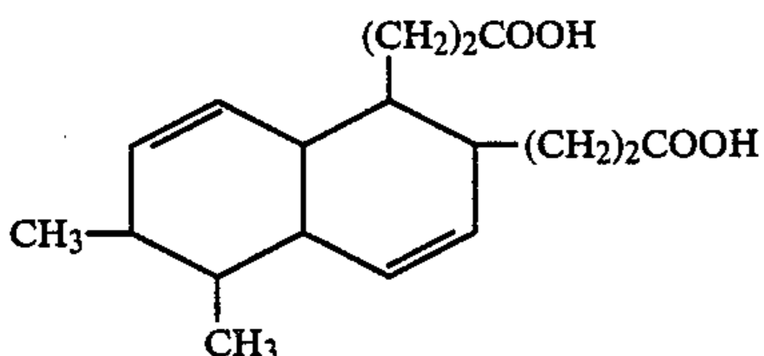
1,2,3,4,4a,5,6,8a-octahydro-5,6-dimethyl-1,2-naphthalene-dipropionic acid. Reactions forming these cyclic compounds from propenyl alcohols usually result in mixtures of acyclic, monocyclic and bicyclic compounds. Thus the reaction of linoleic and oleic acids in the presence of a clay catalyst results in a mixture of compounds L, M and
