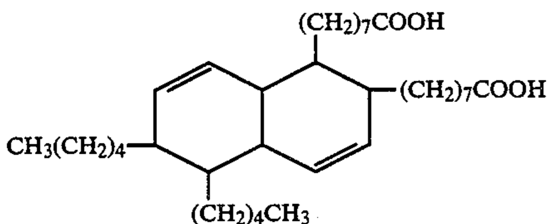
5,6-dibutyl-1,2,4a,5,6,8a-hexahydro-1,2-naphthalene-dioctanoic acid
