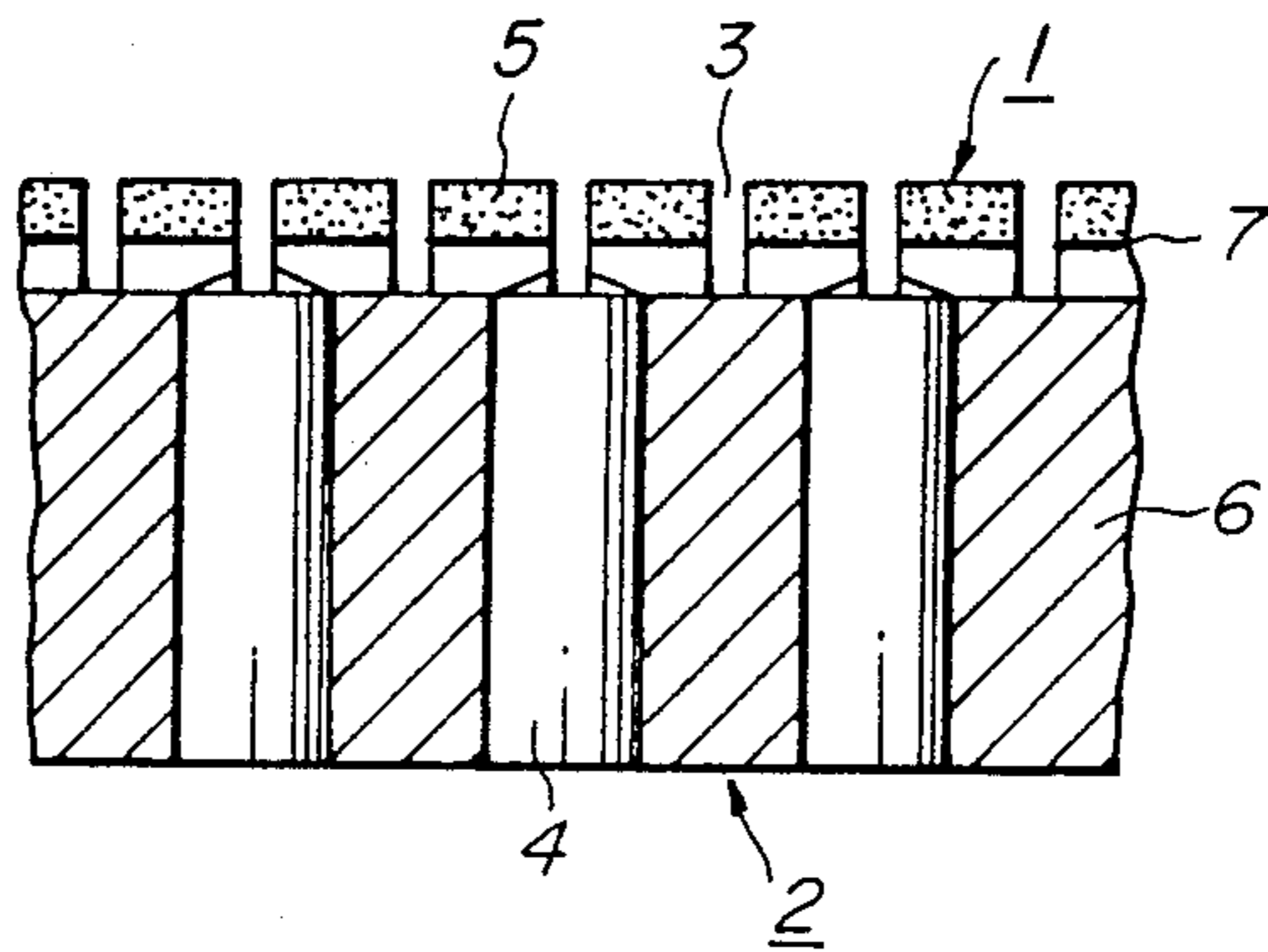
FIG. 2 PRIOR ART
