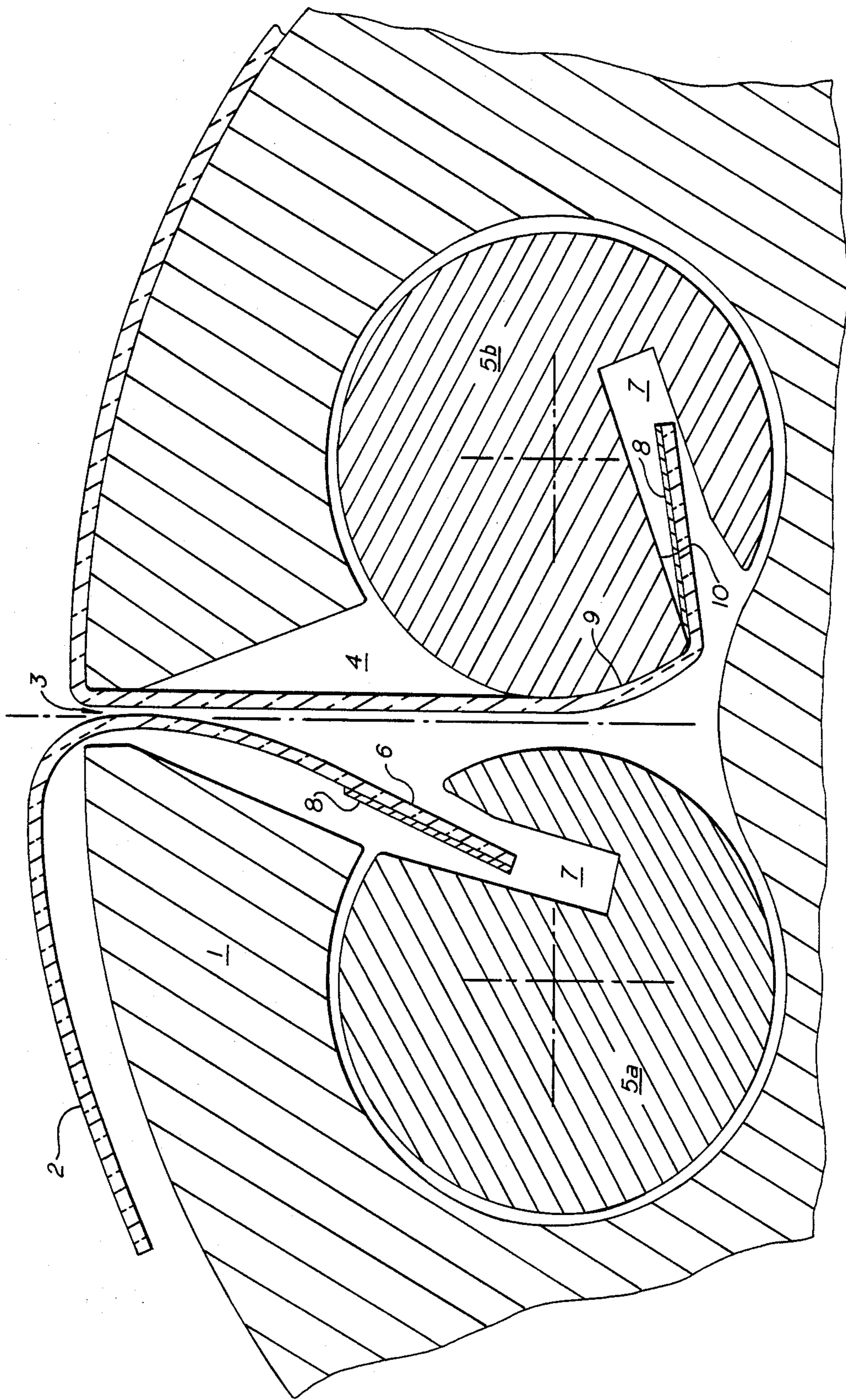
FIG. 1 PRIOR ART
