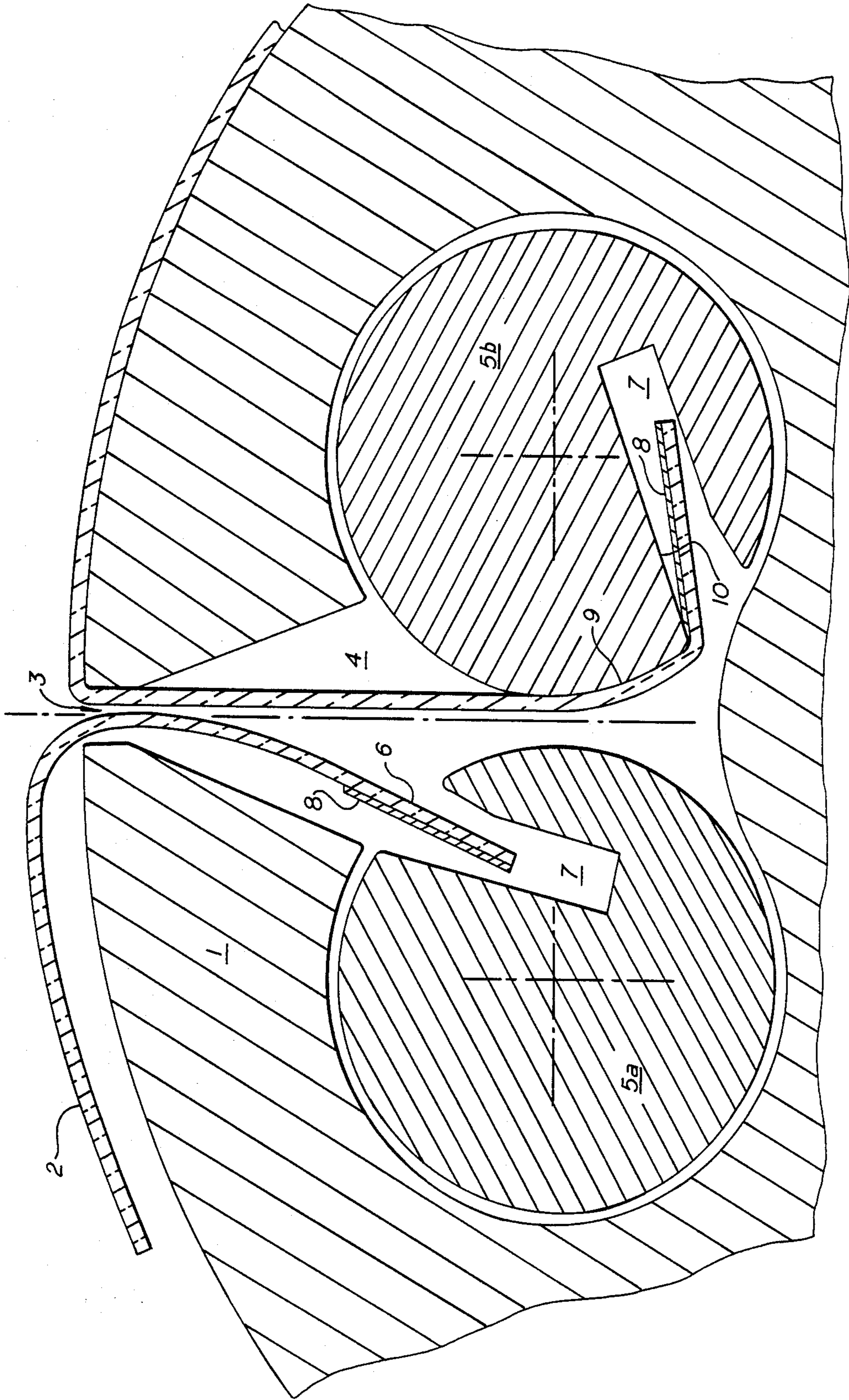
FIG. 1 PRIOR ART
