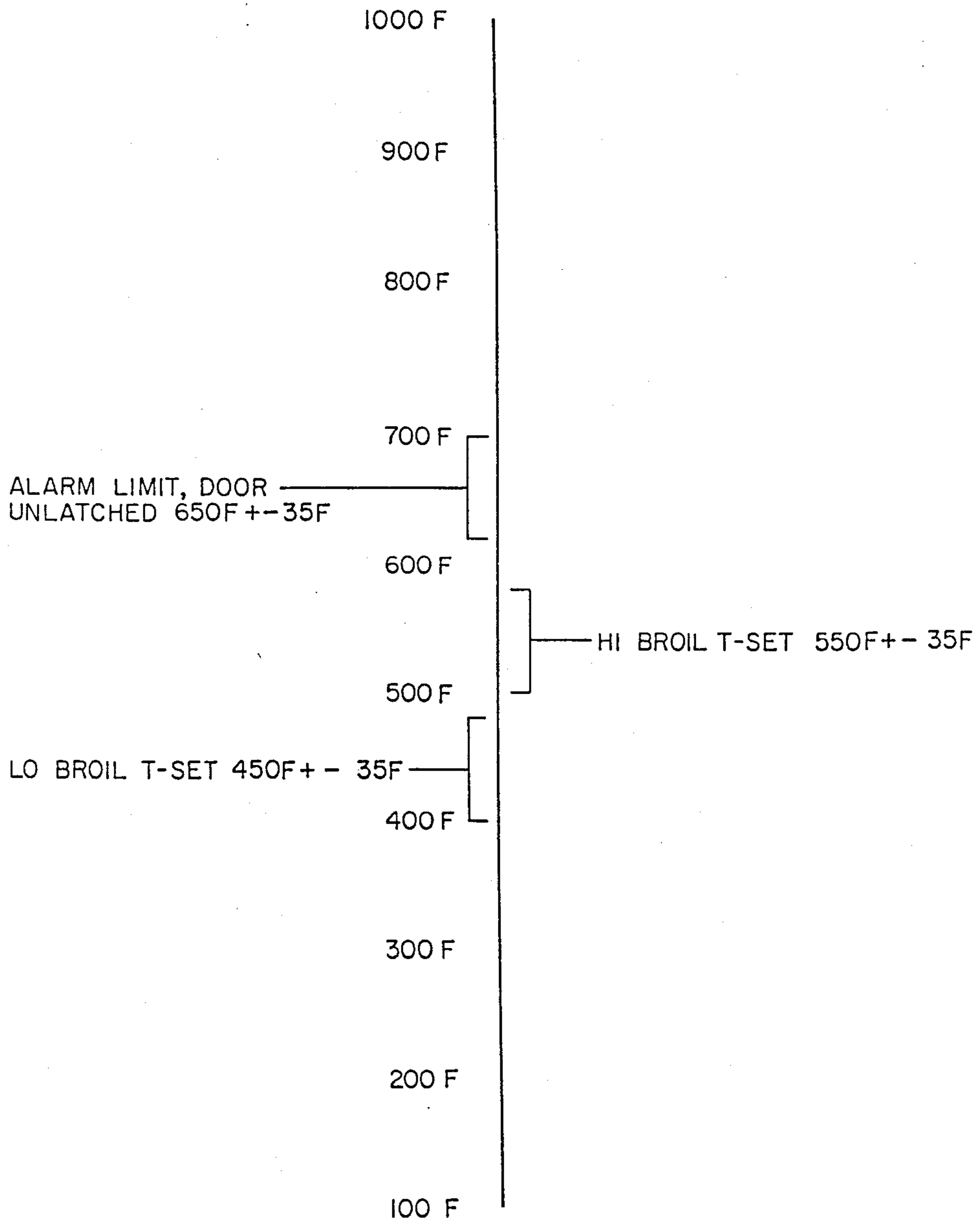
BROIL MODE TEMPERATURE ACTION POINTS.
