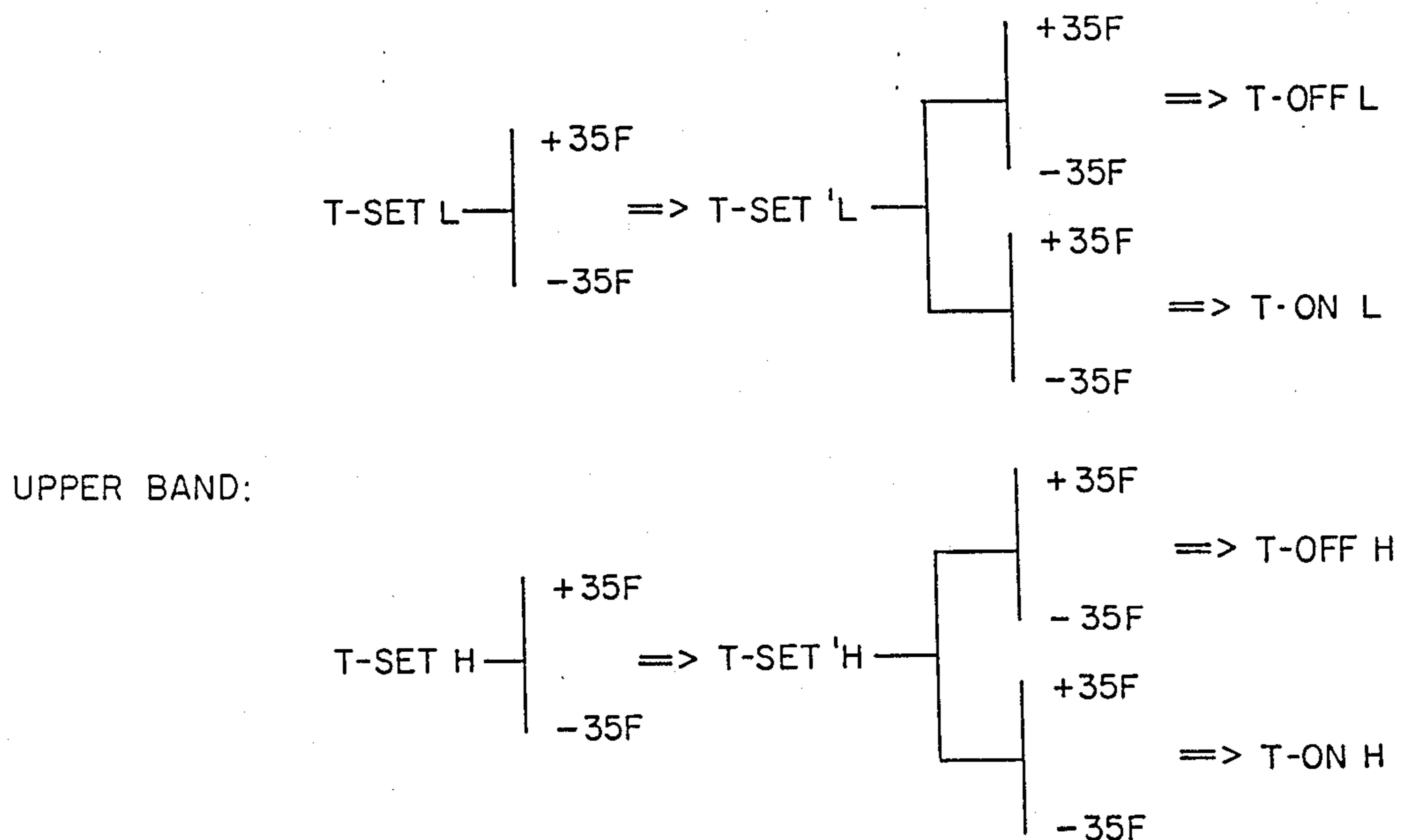
FORMATION OF ELEMENT RELAY T-ON AND T-OFF TEMPERATURES.
