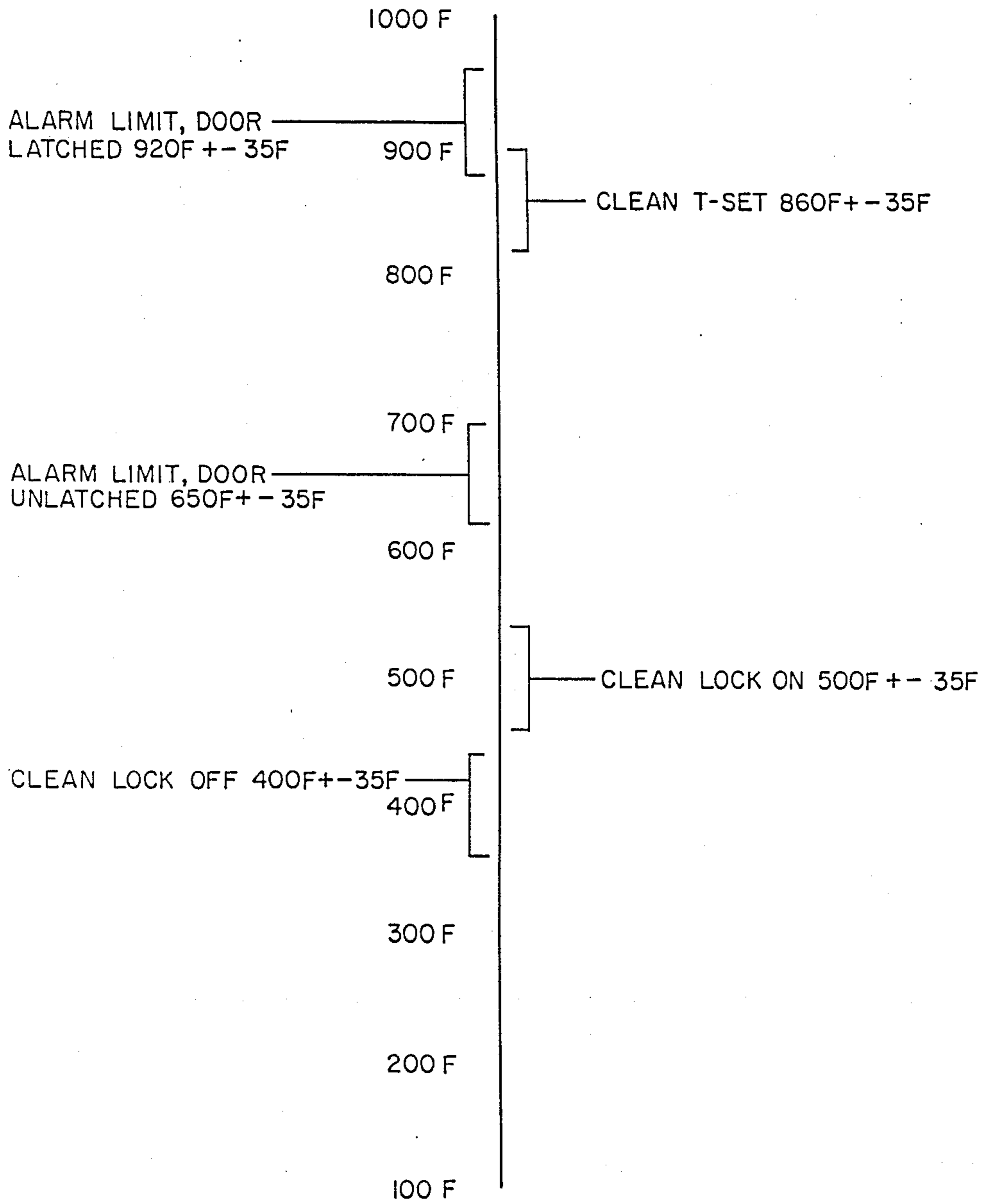
CLEAN MODE TEMPERATURE ACTION POINTS.
