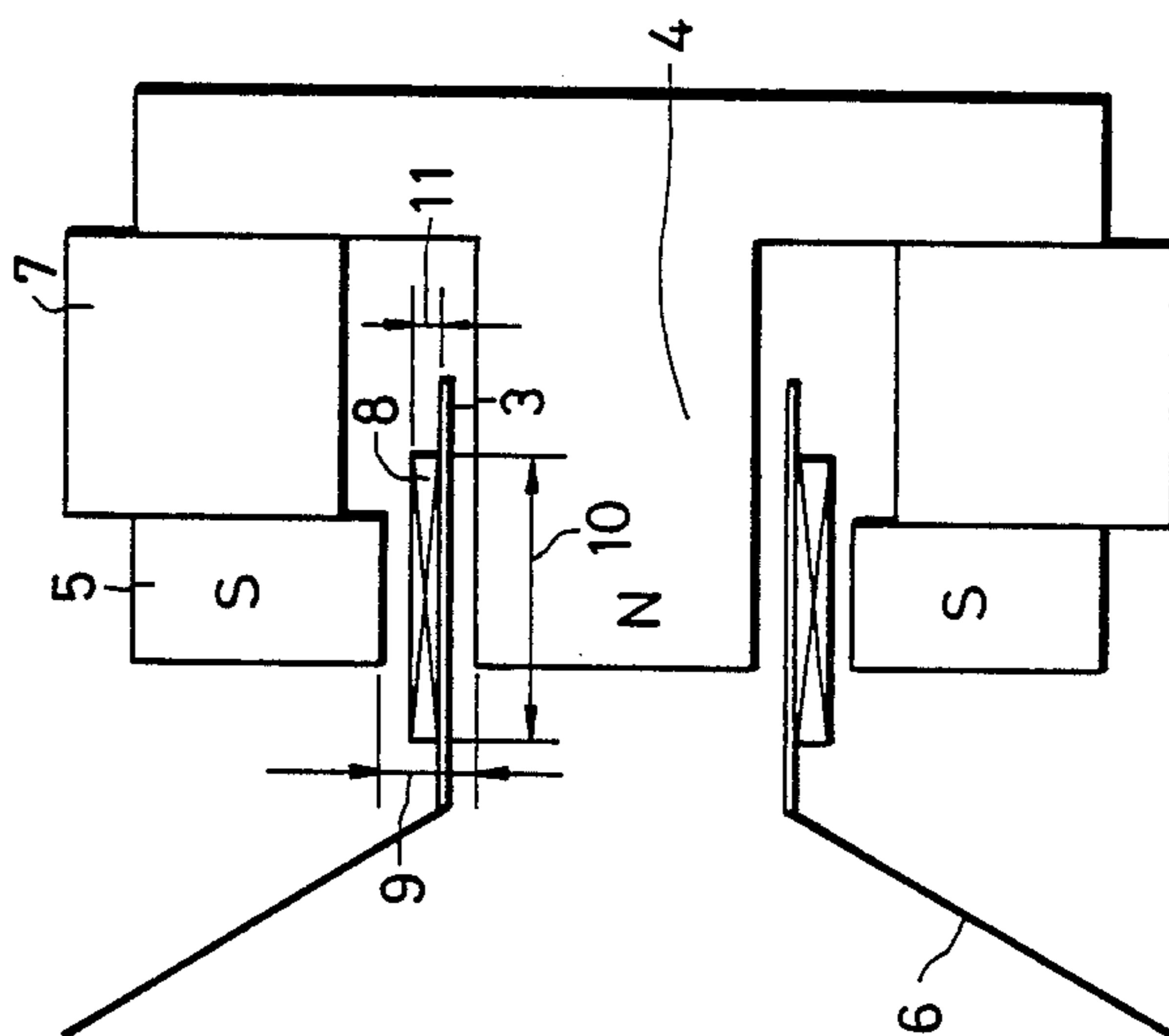
FIG. 1 PRIOR ART
