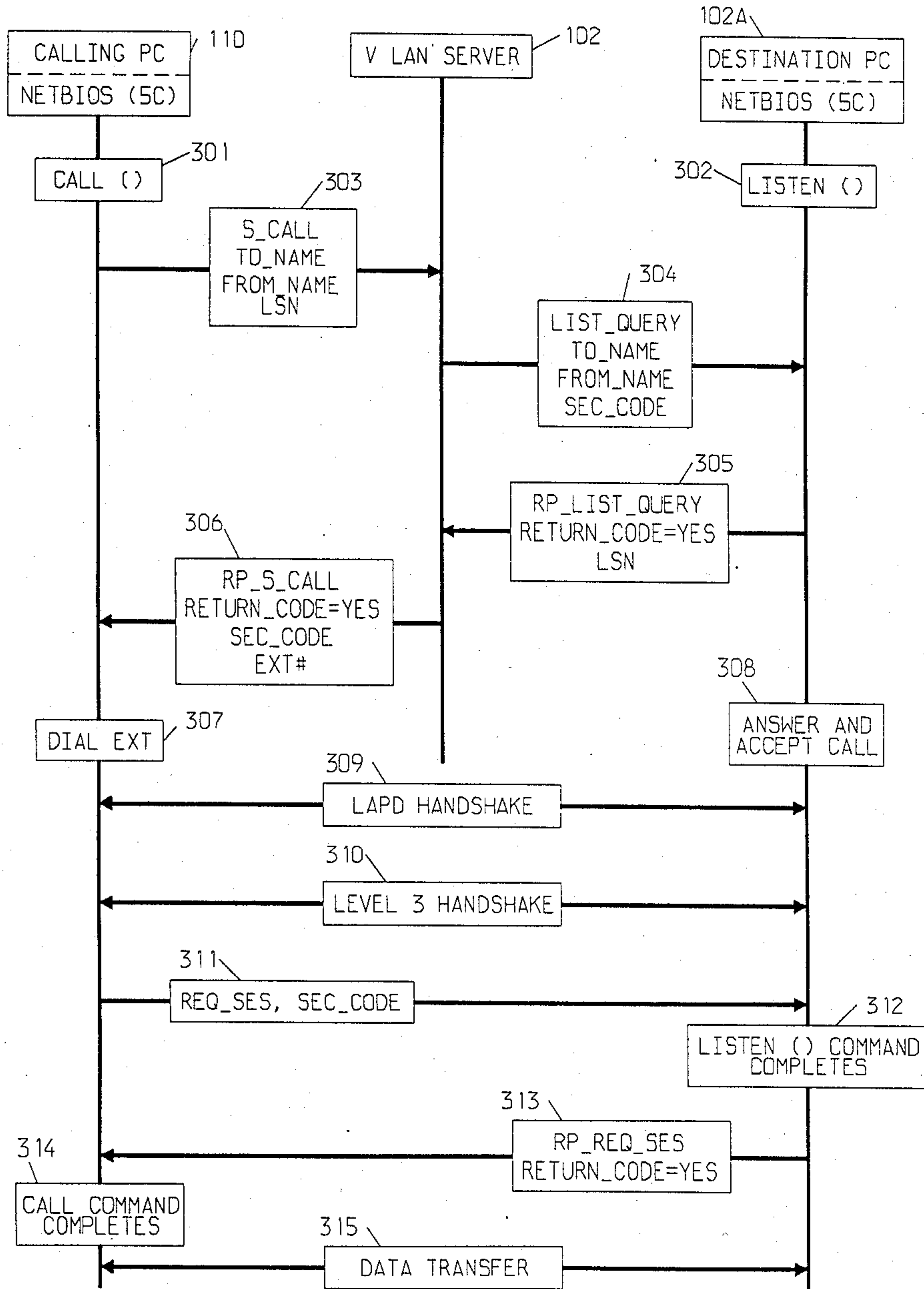
FIG. 3 CALL SET UP SEQUENCE
