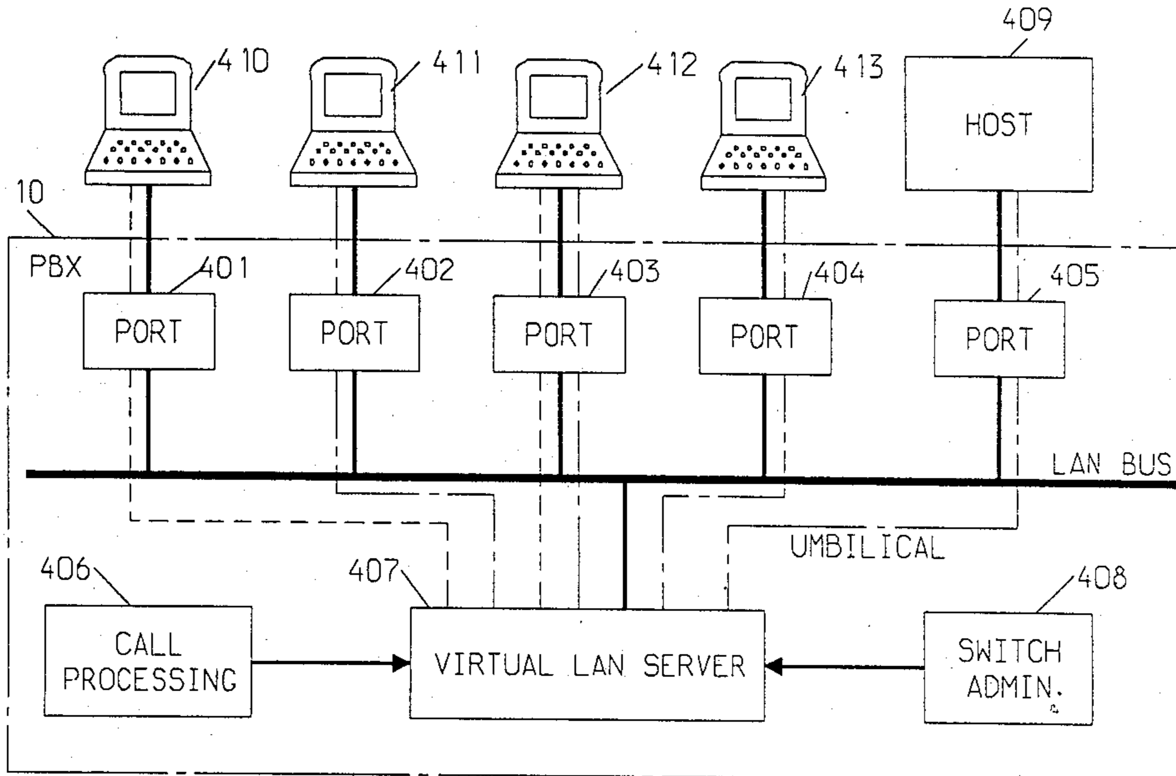
FIG. 4 UMBILICAL CONNECTIONS AND VIRTUAL LANS
