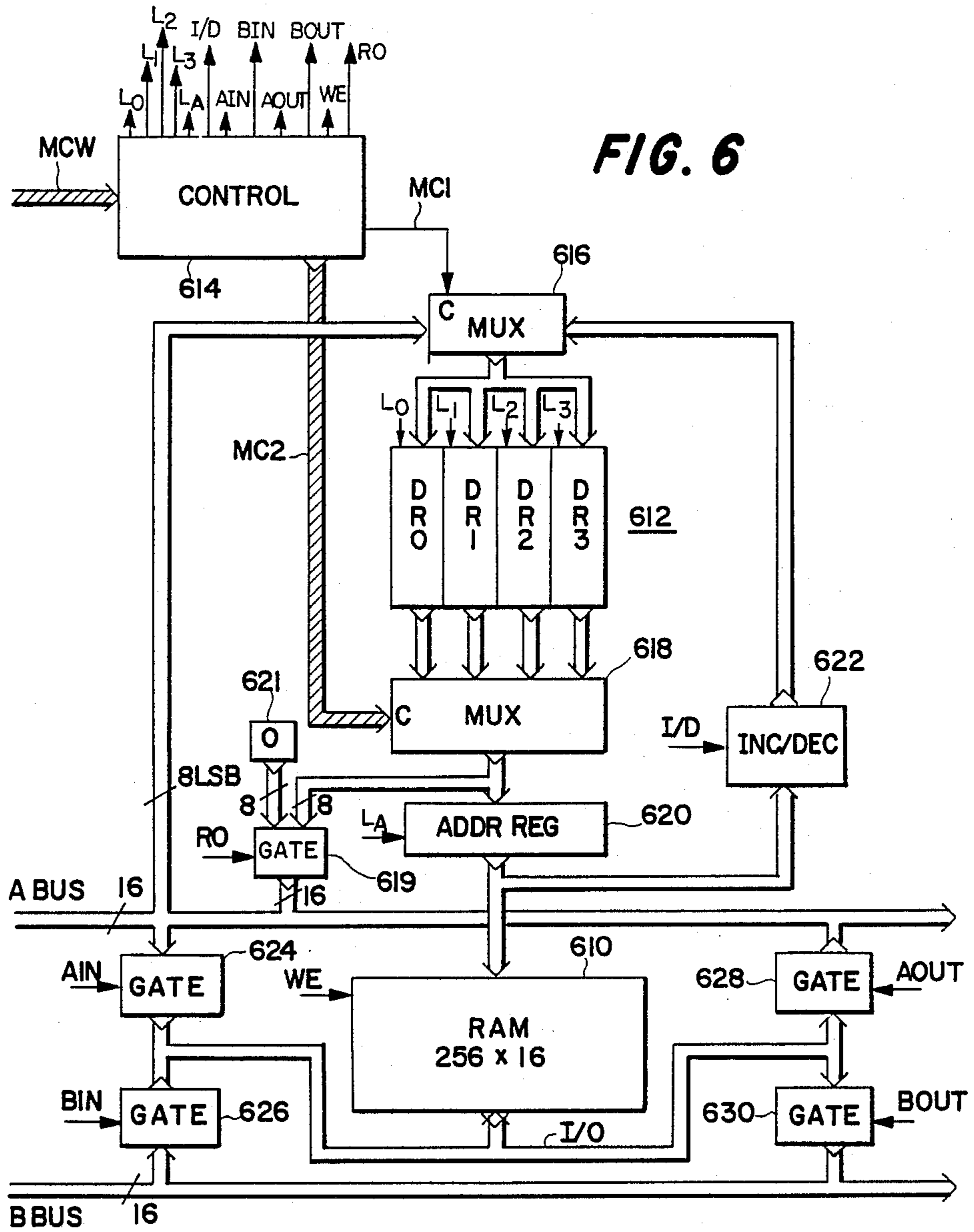
DATA RAM
