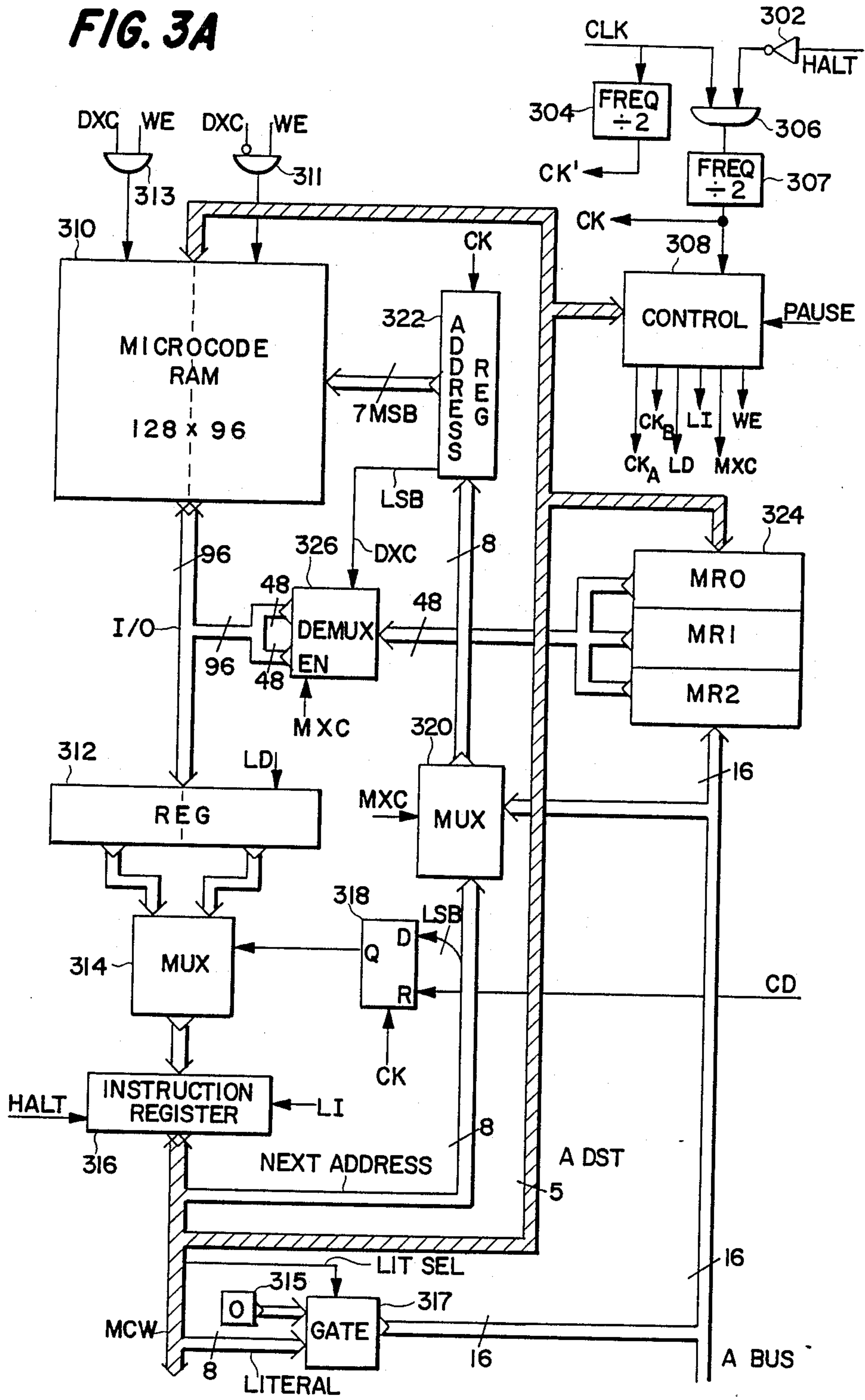
MICROCODE RAM AND SEQUENCER
