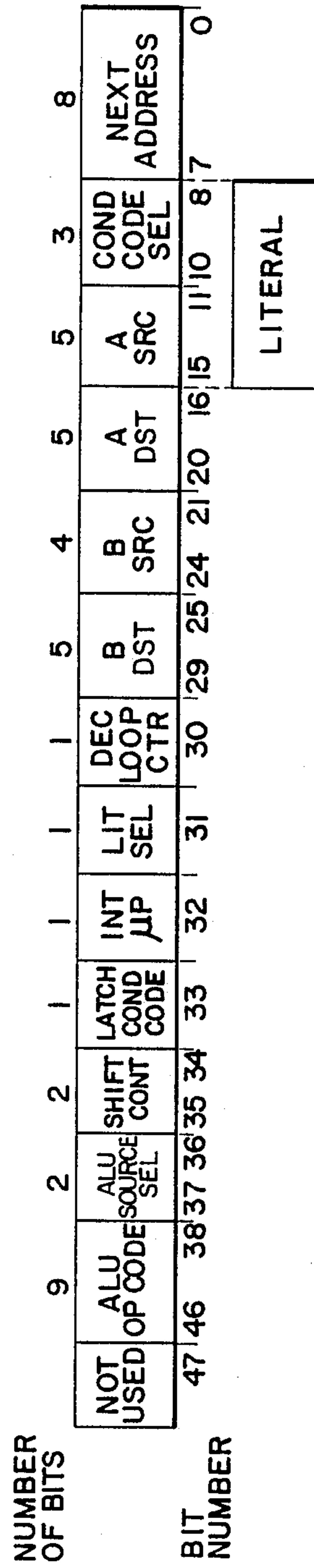
MICROCODE CONTROL WORD
