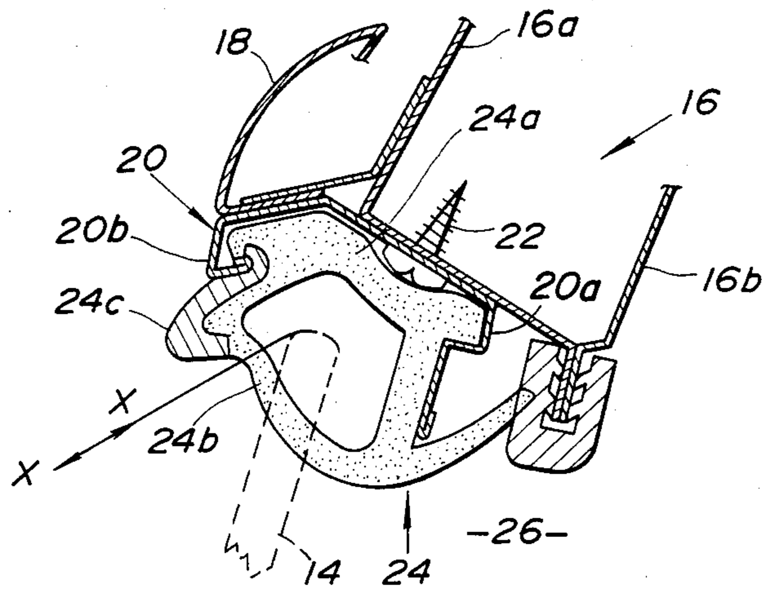
FIG. 5 (PRIOR ART)
