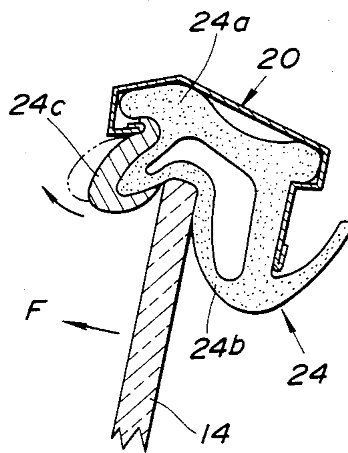
FIG. 6 (PRIOR ART)
