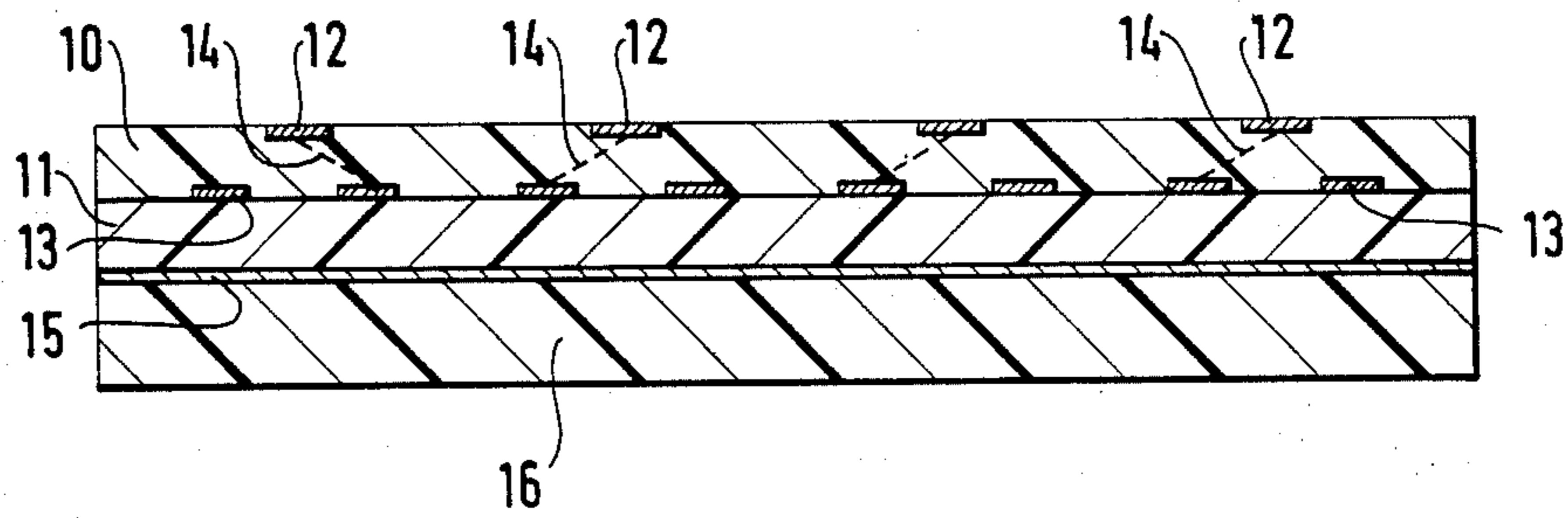
FIG. 1 PRIOR ART
