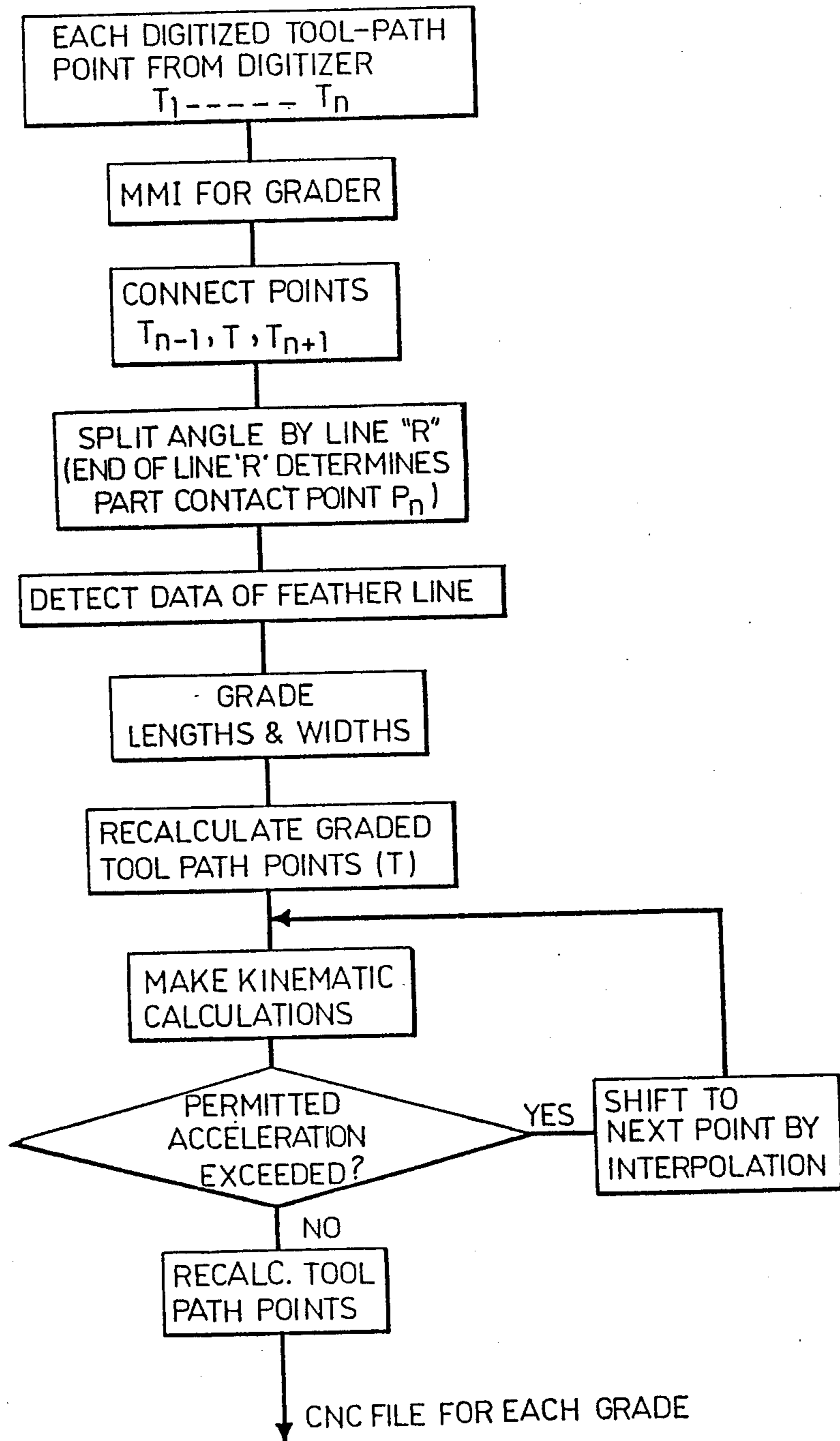
FIG 9 GRADING SOFTWARE
