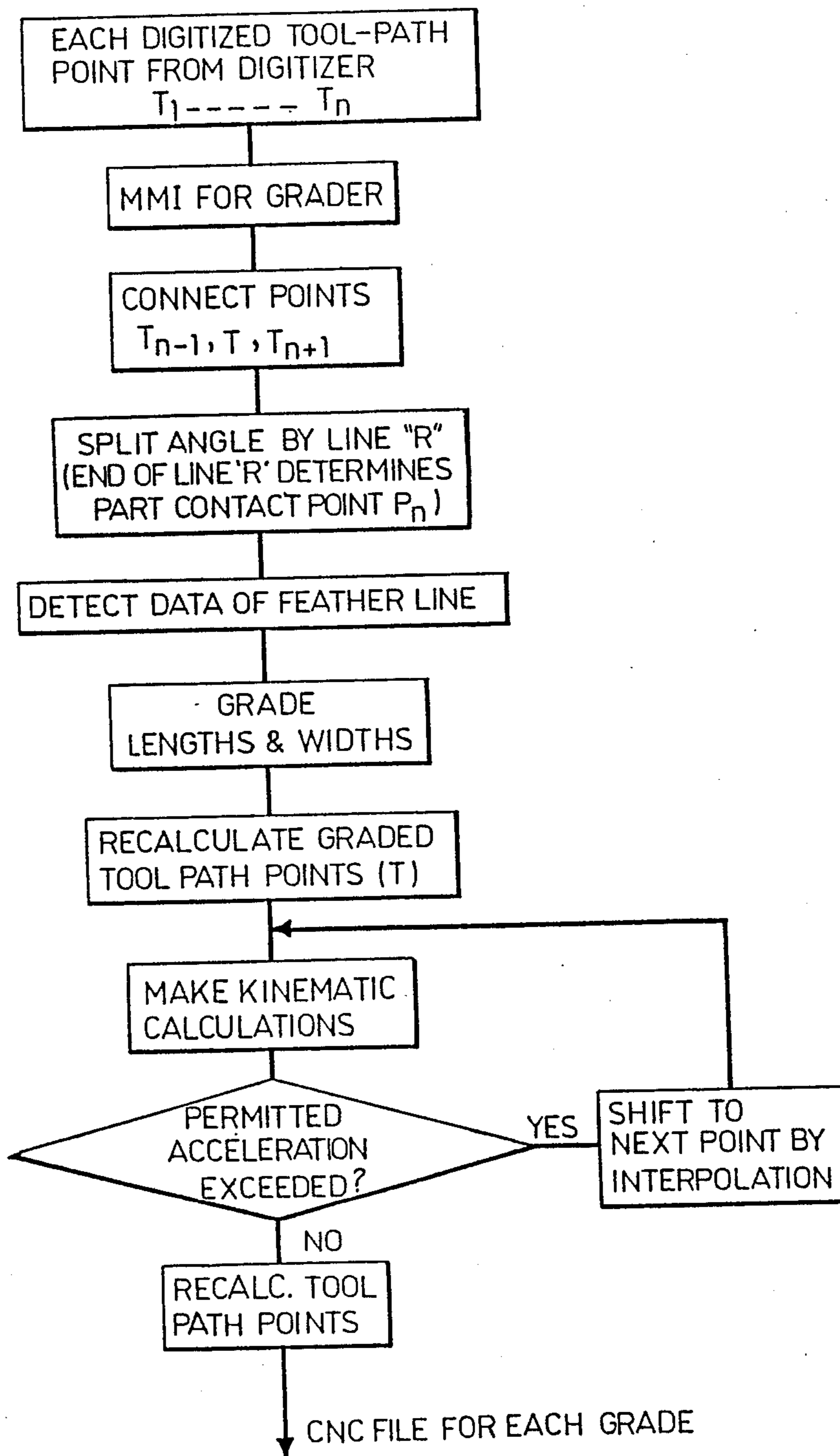
FIG 9 GRADING SOFTWARE
