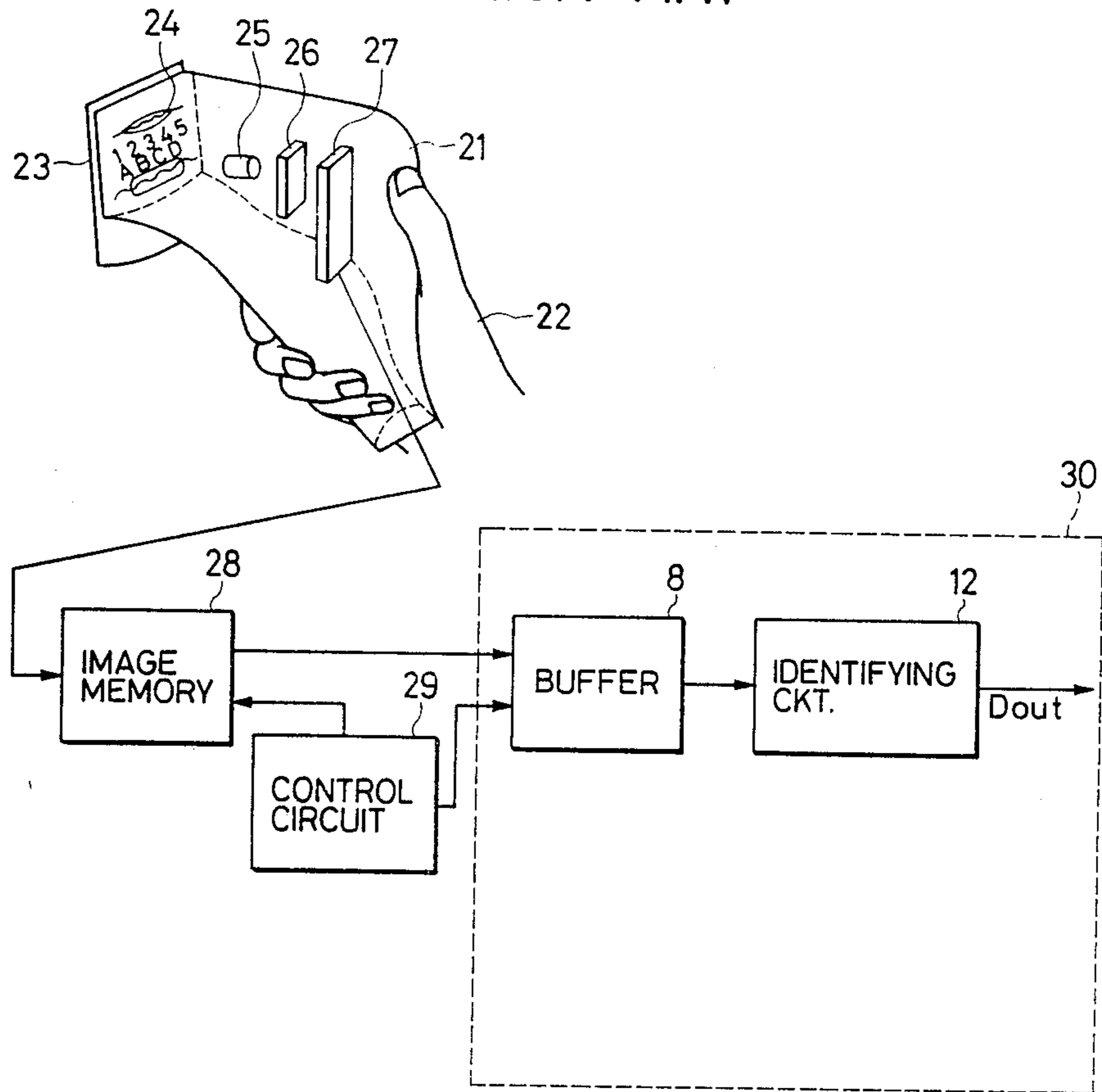
FIG. 2 PRIOR ART
