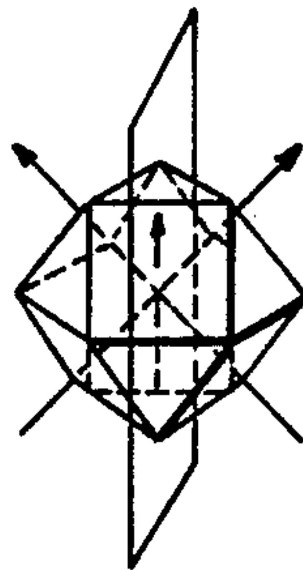
CUBOCTAHEDRON
