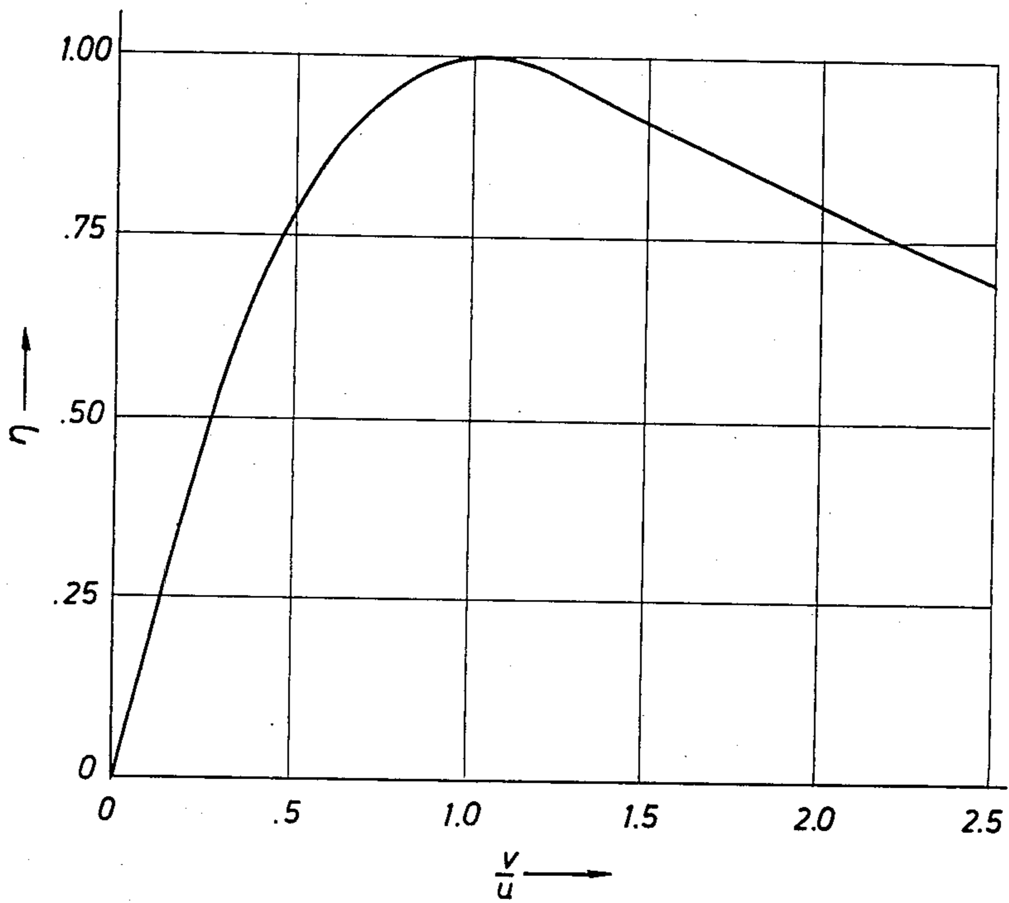
FIG. 7 PROPULSIVE EFFICIENCY \eta AS A FUNCTION OF VELOCITY RATIO
