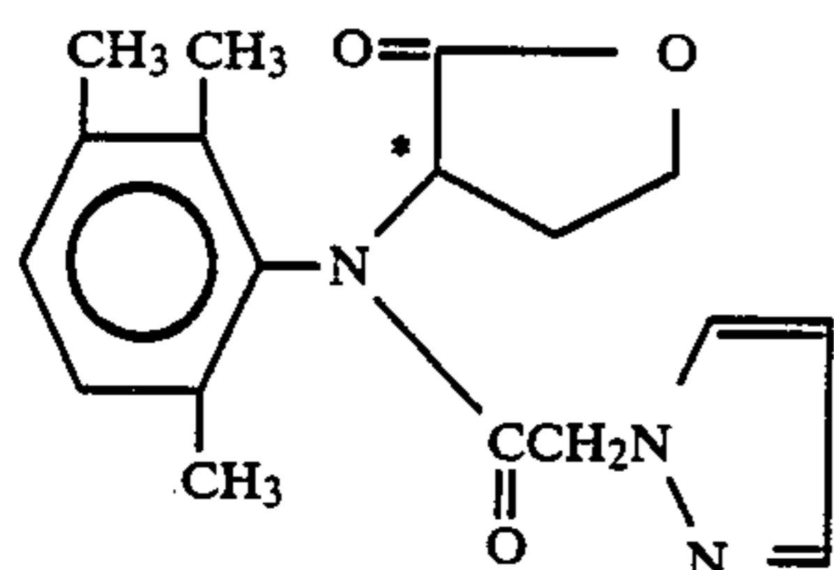
3-[N-(1,2-pyrazol-1-yl-acetyl)-N-(2,3,6-trimethylphenyl)]amino-tetrahydro-2-furanone (compound No. 111)
