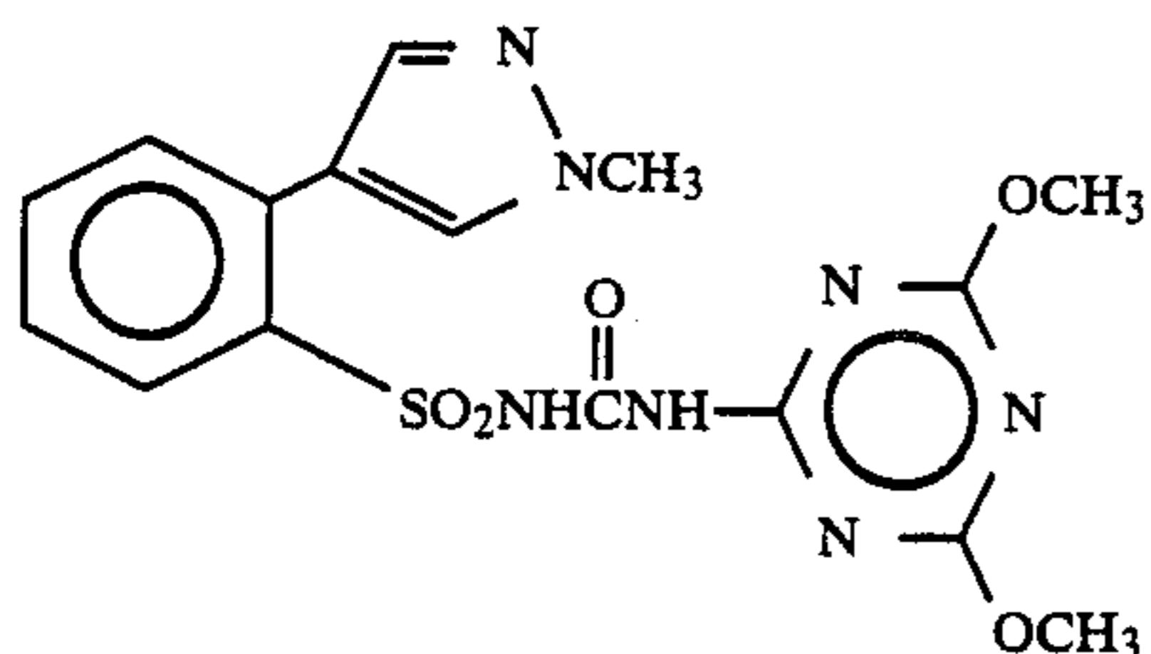
Compound 35
