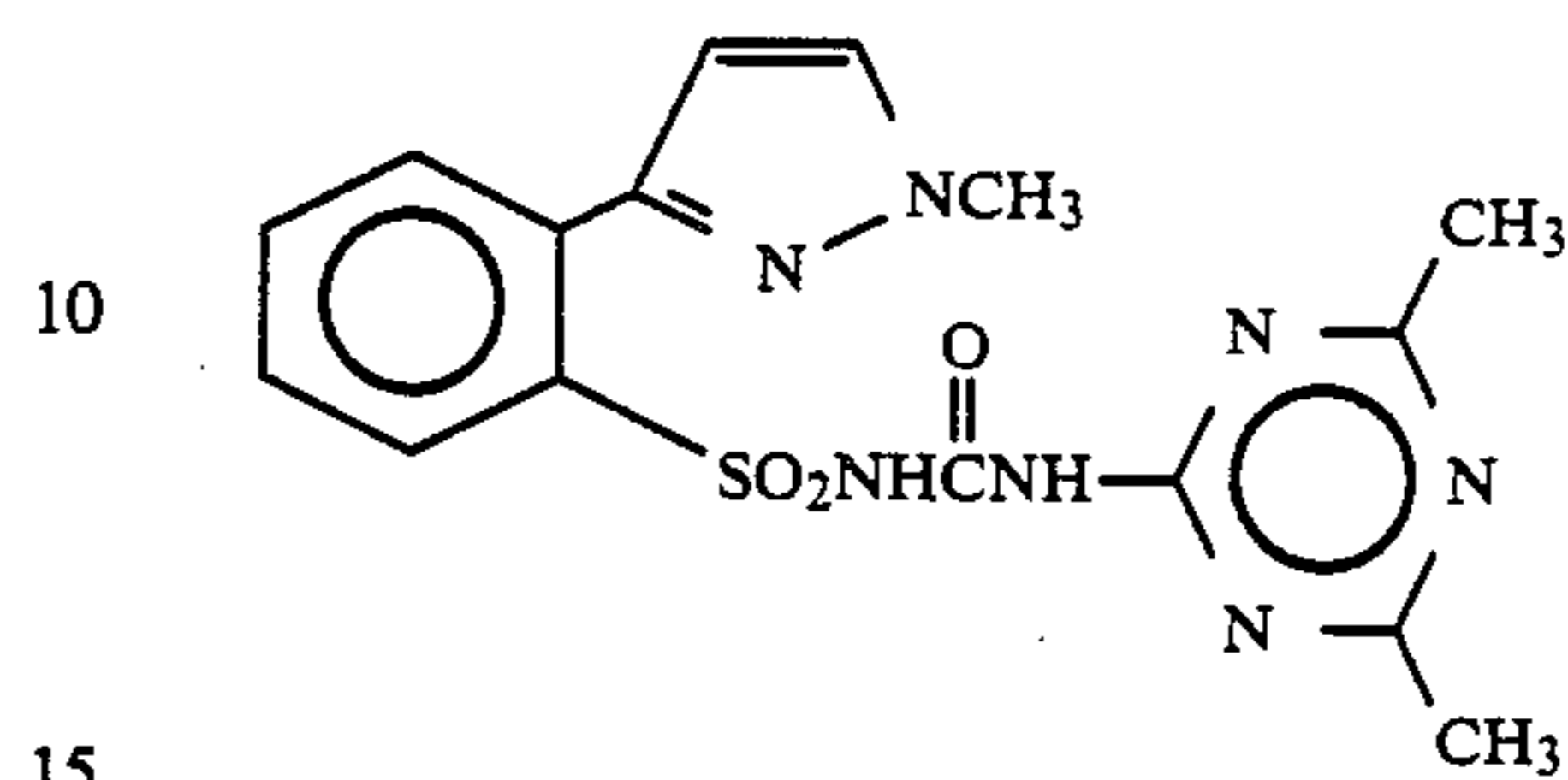
Compound 34
