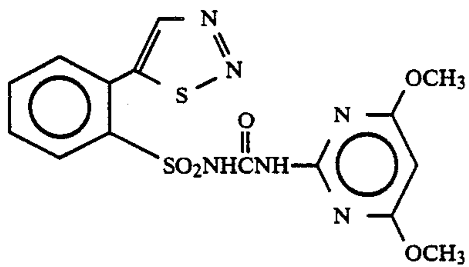
Compound 20
