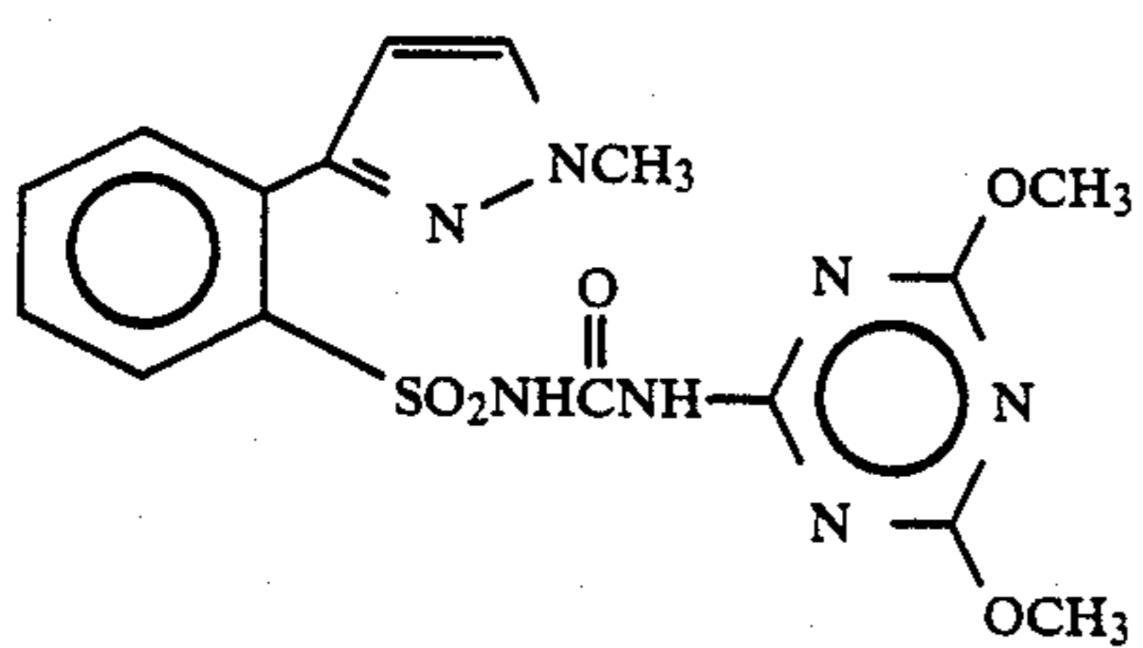
Compound 39
