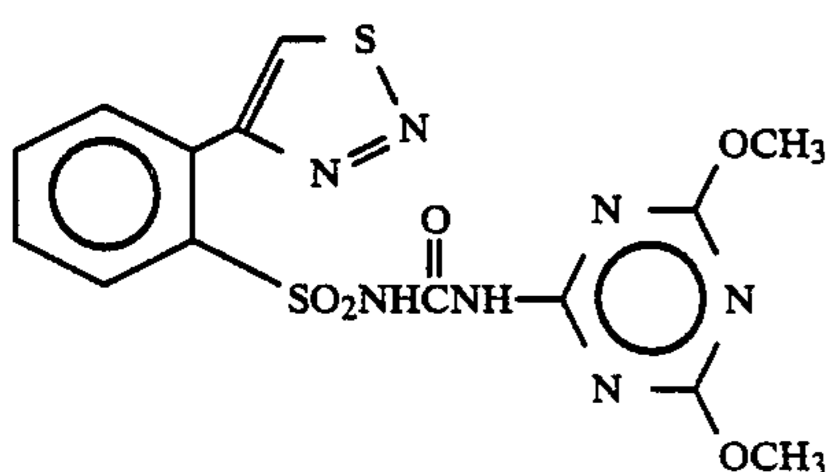
Compound 23
