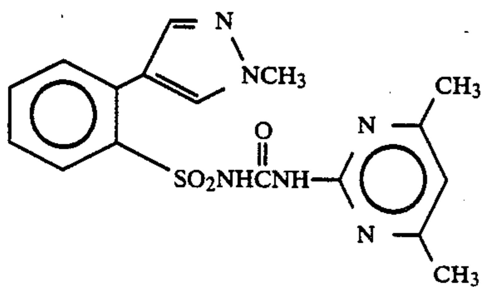
Compound 34
