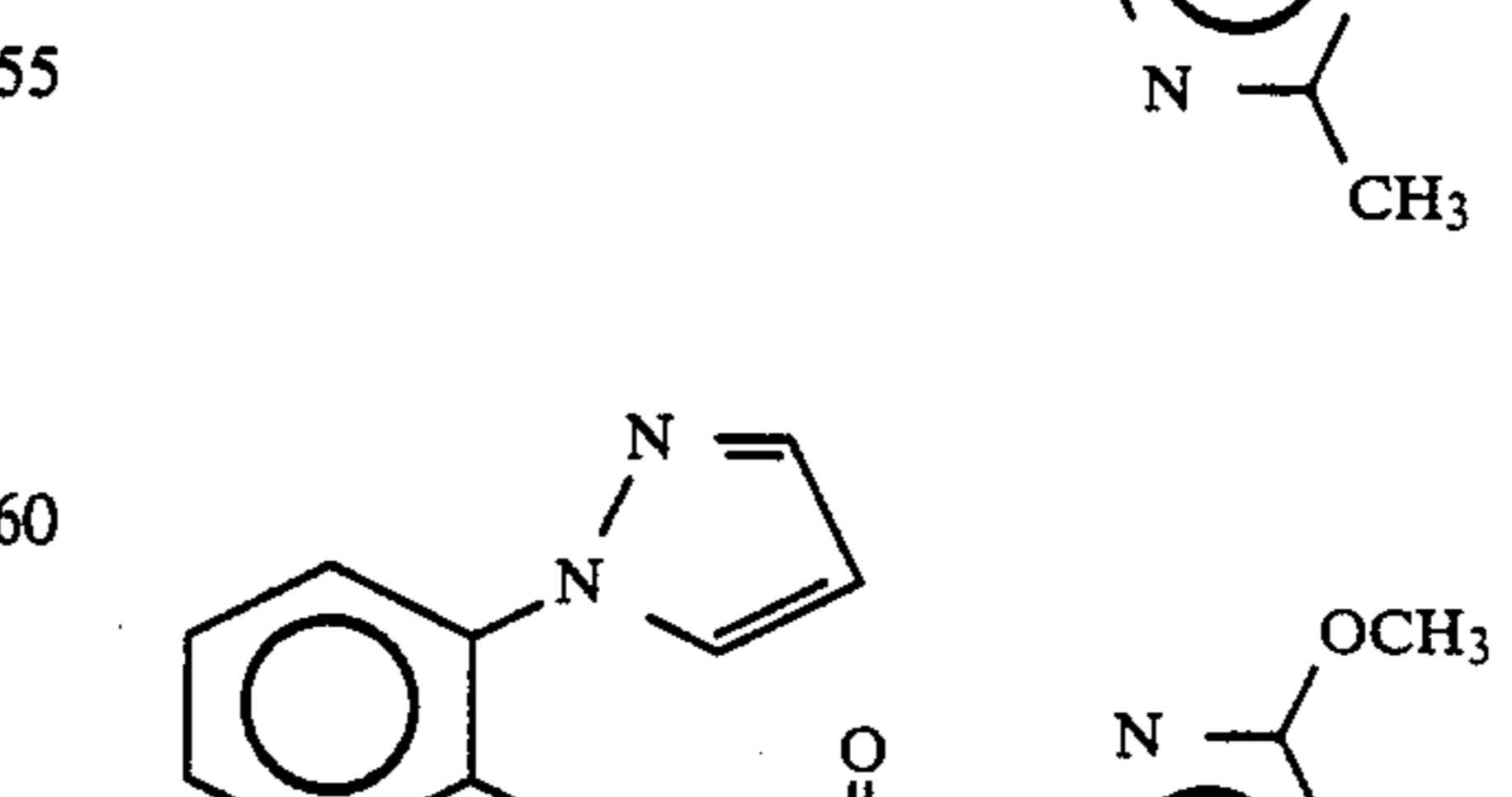
Compound 39
