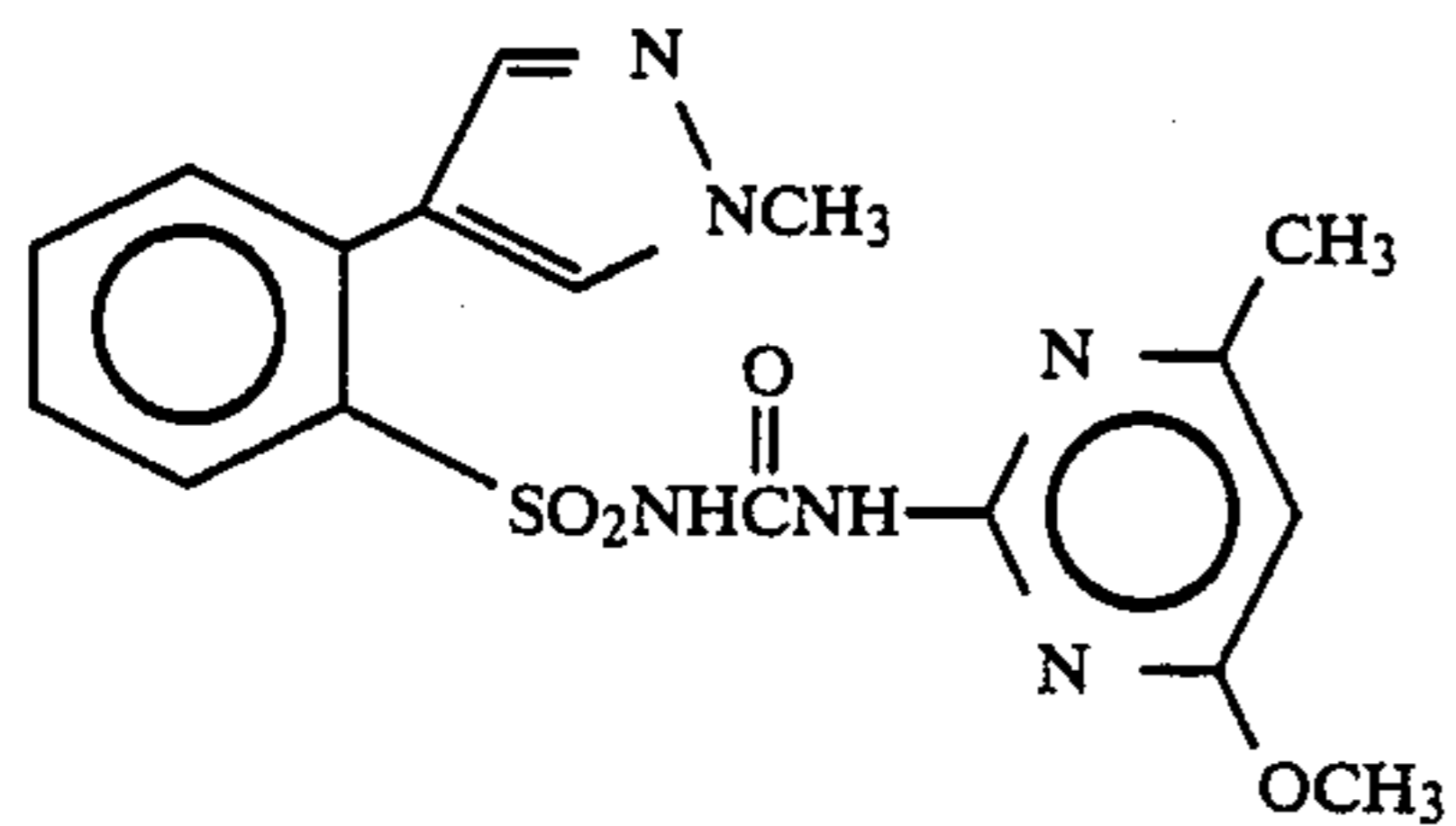
Compound 33
