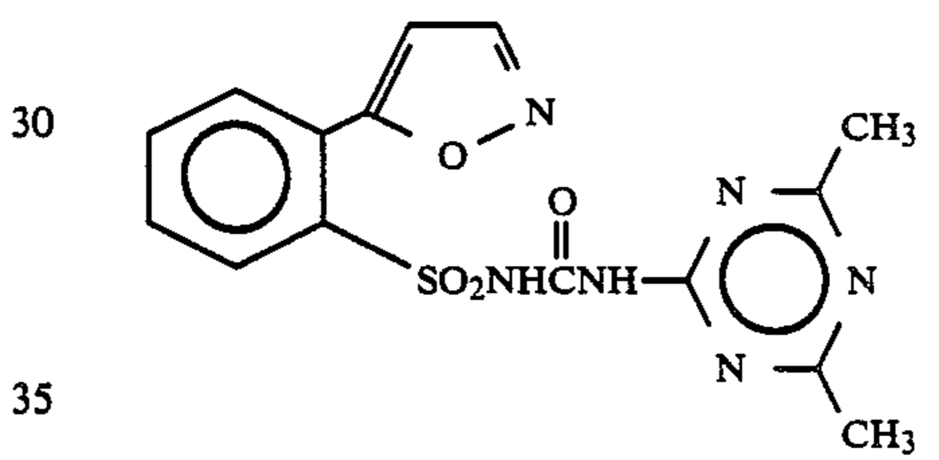
Compound 23
