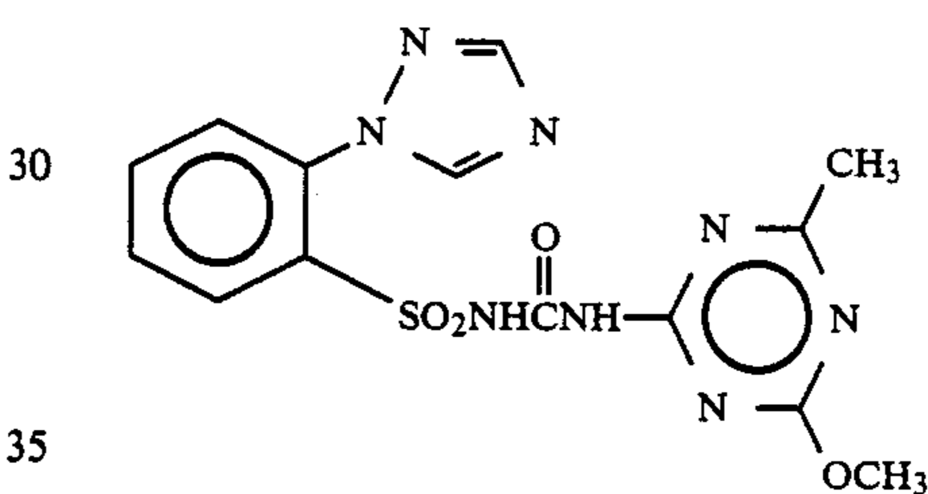
Compound 36
