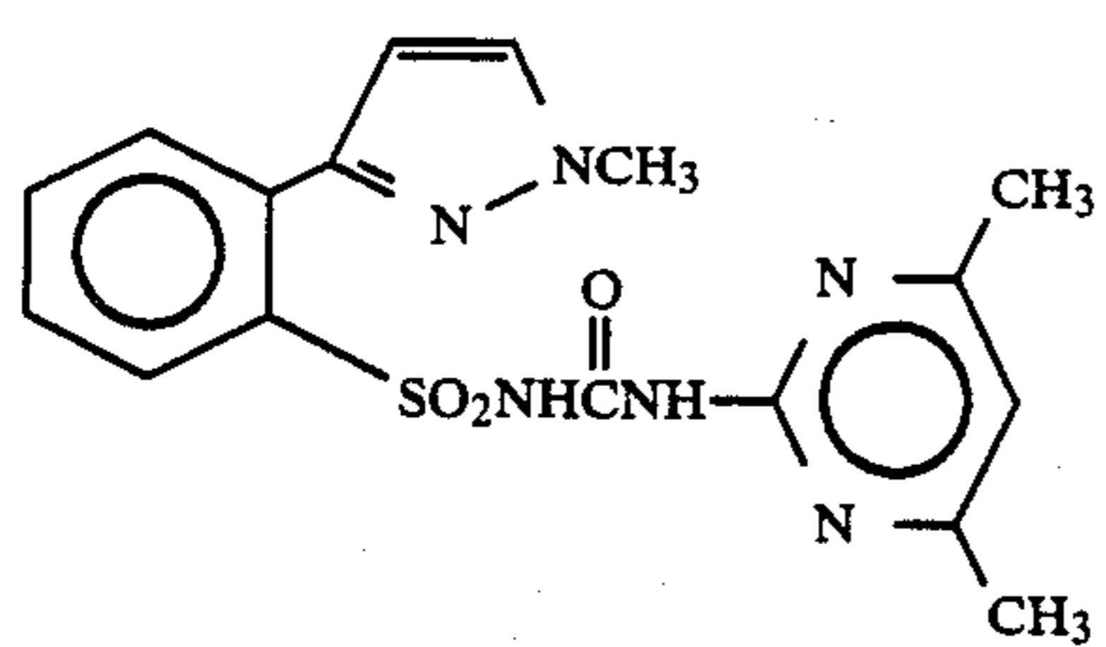
Compound 38
