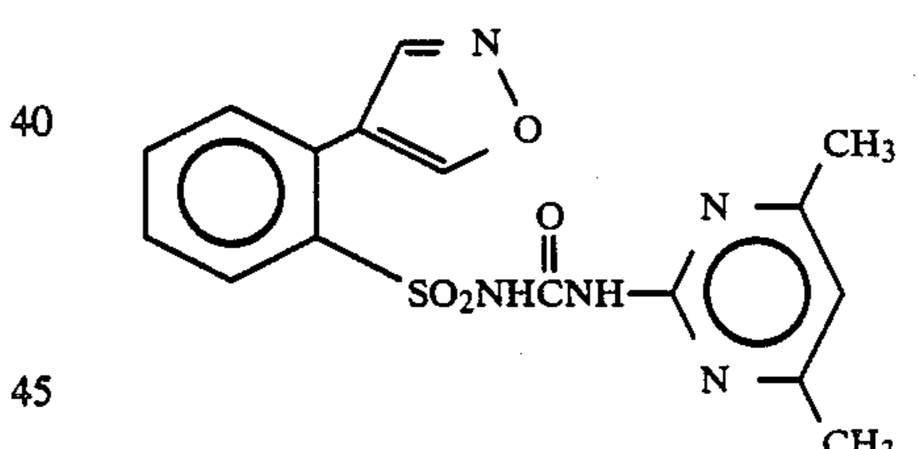
Compound 24
