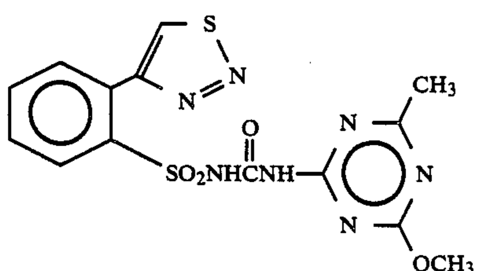
Compound 24
