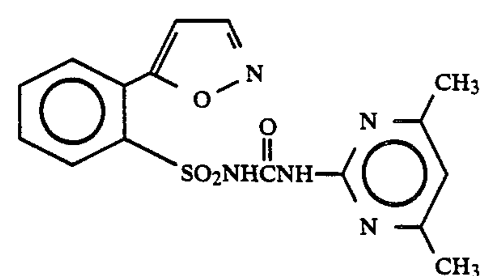
Compound 26
