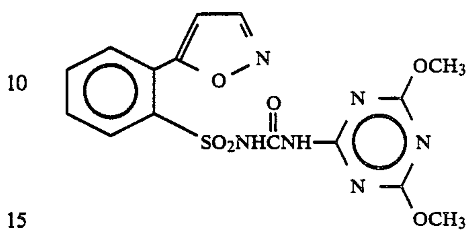
Compound 21
