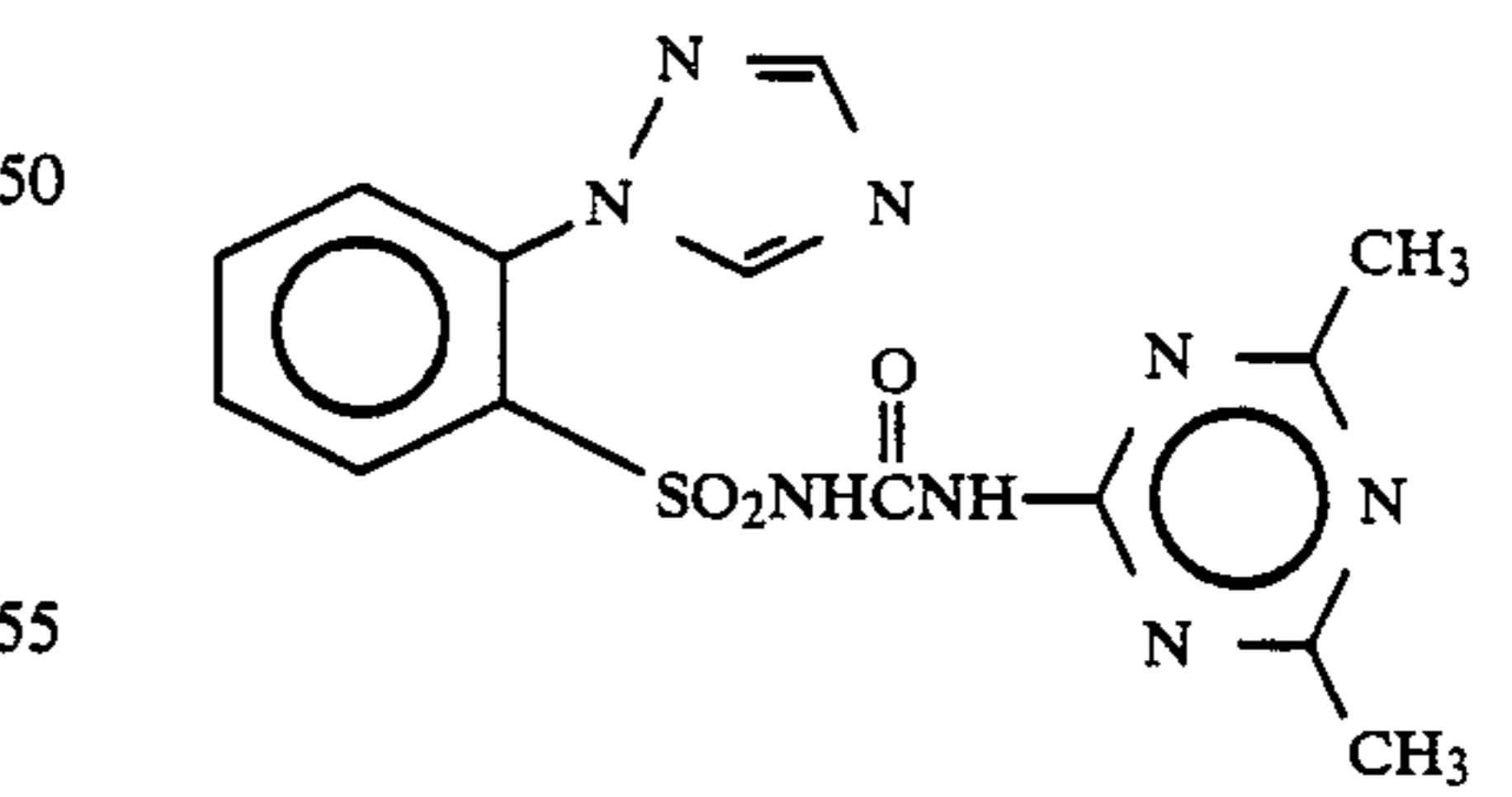
Compound 38
