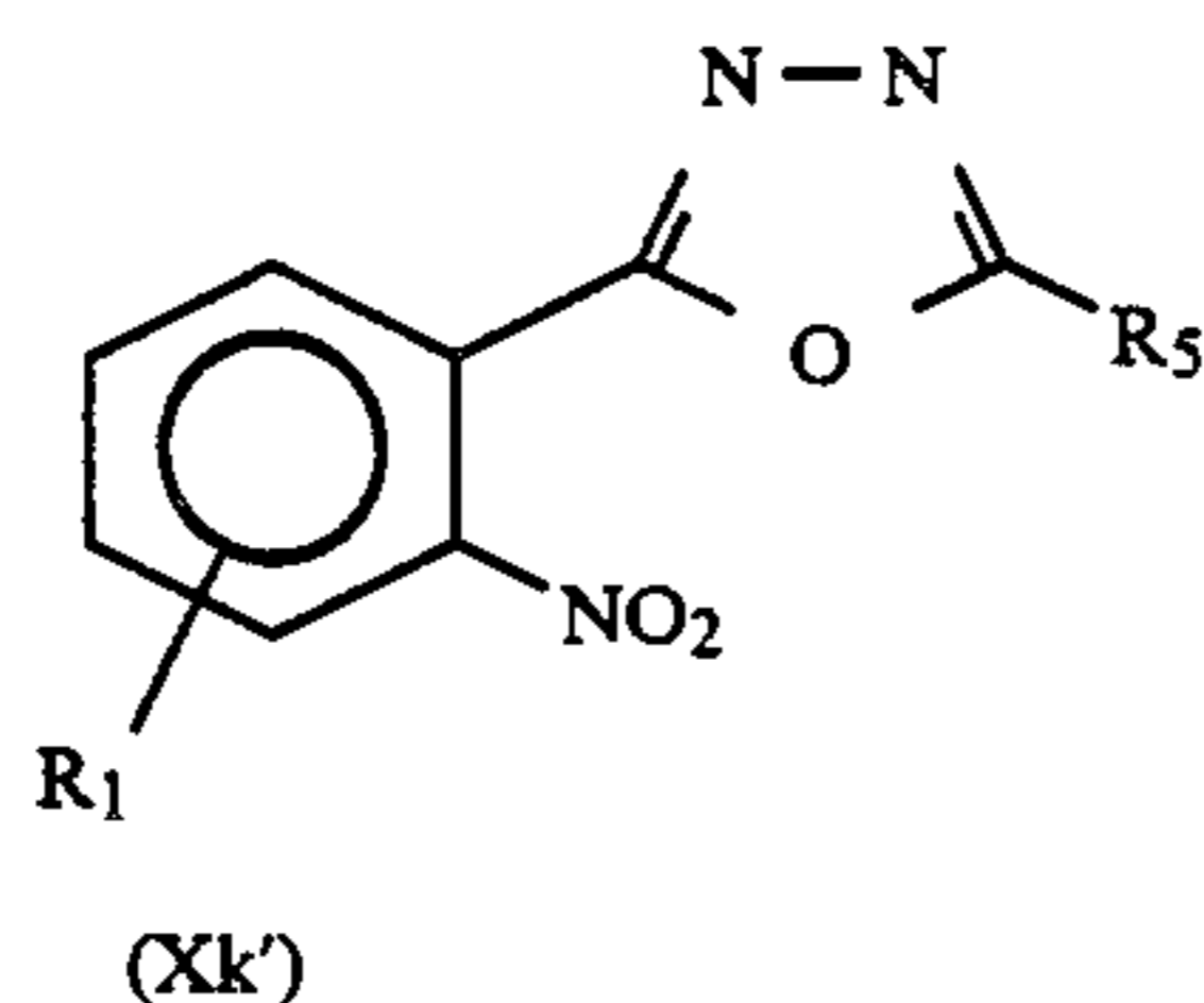
-continued Equation 35
