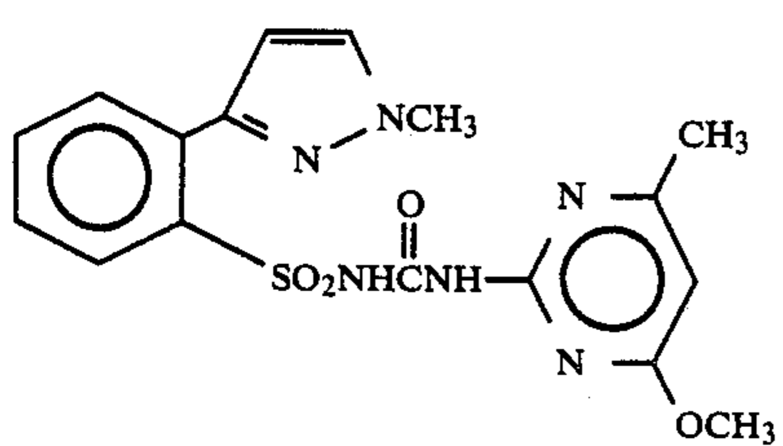
Compound 37
