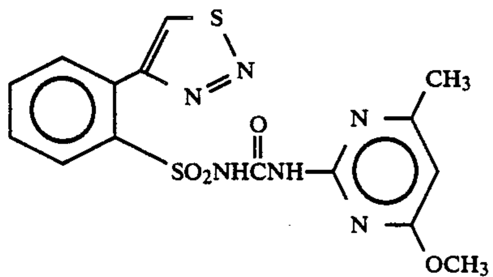
Compound 21
