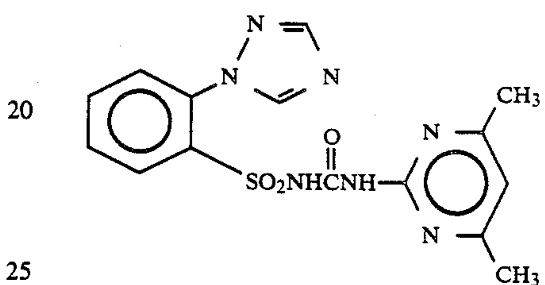
Compound 35
