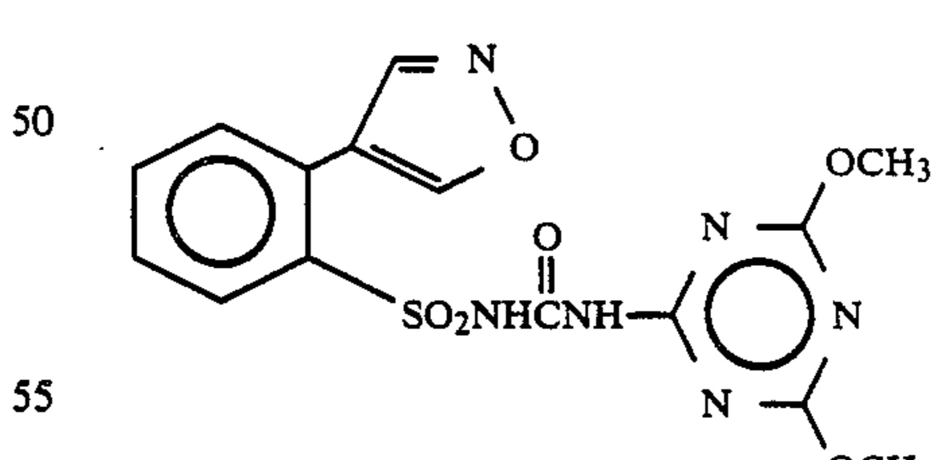
Compound 25
