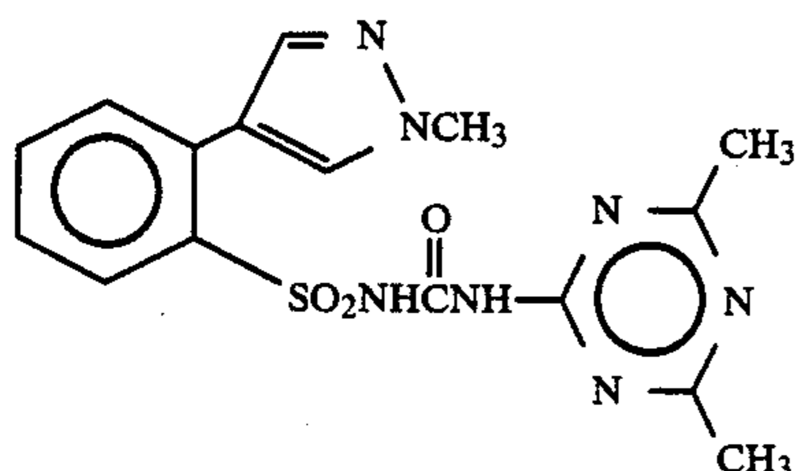
Compound 36
