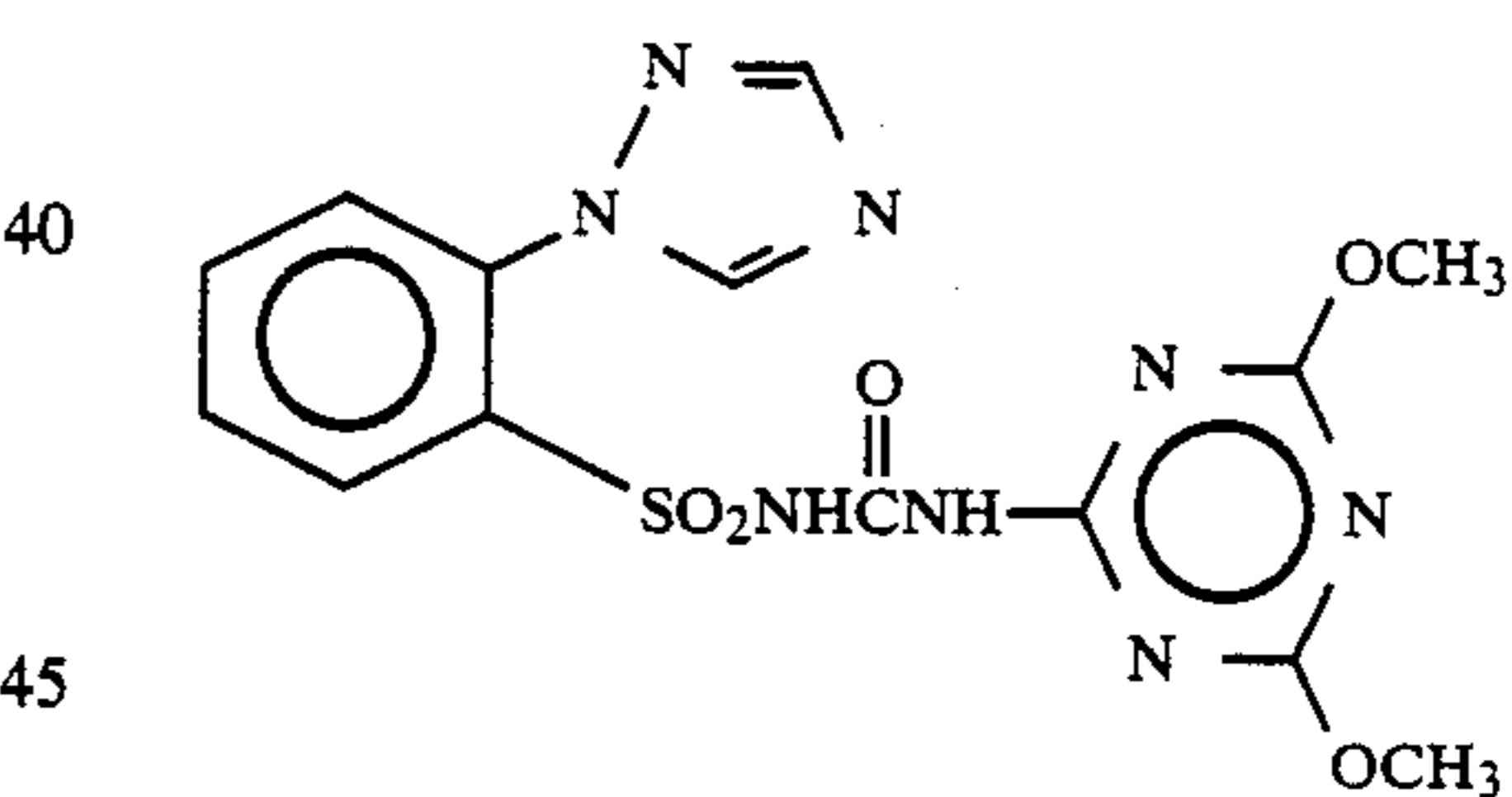
Compound 37
