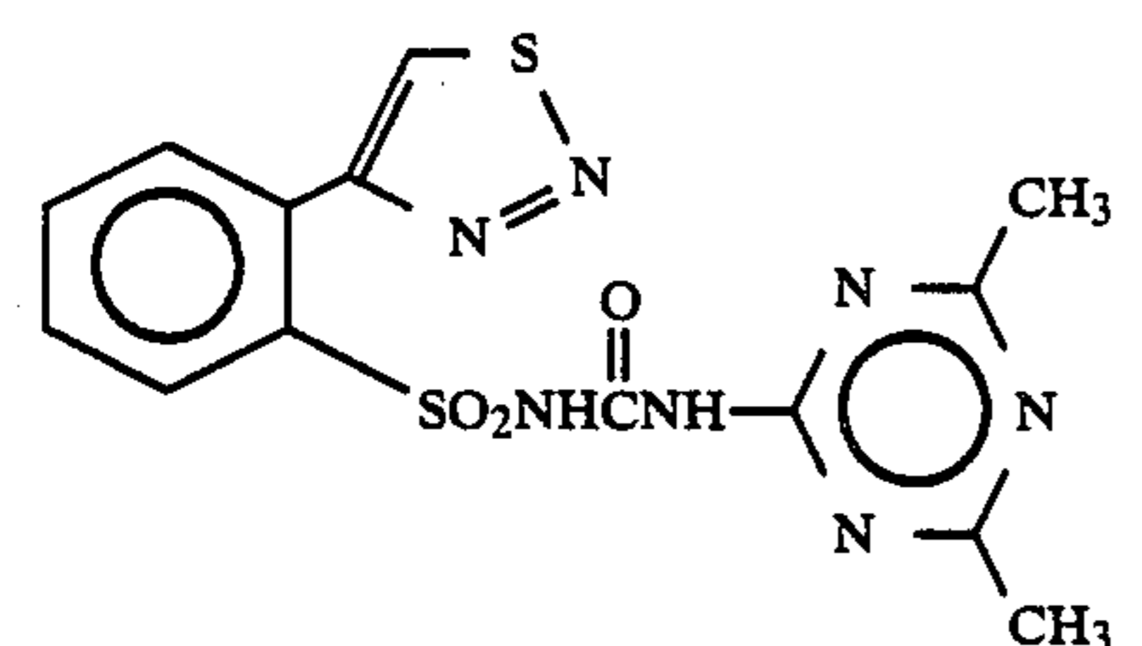
Compound 25
