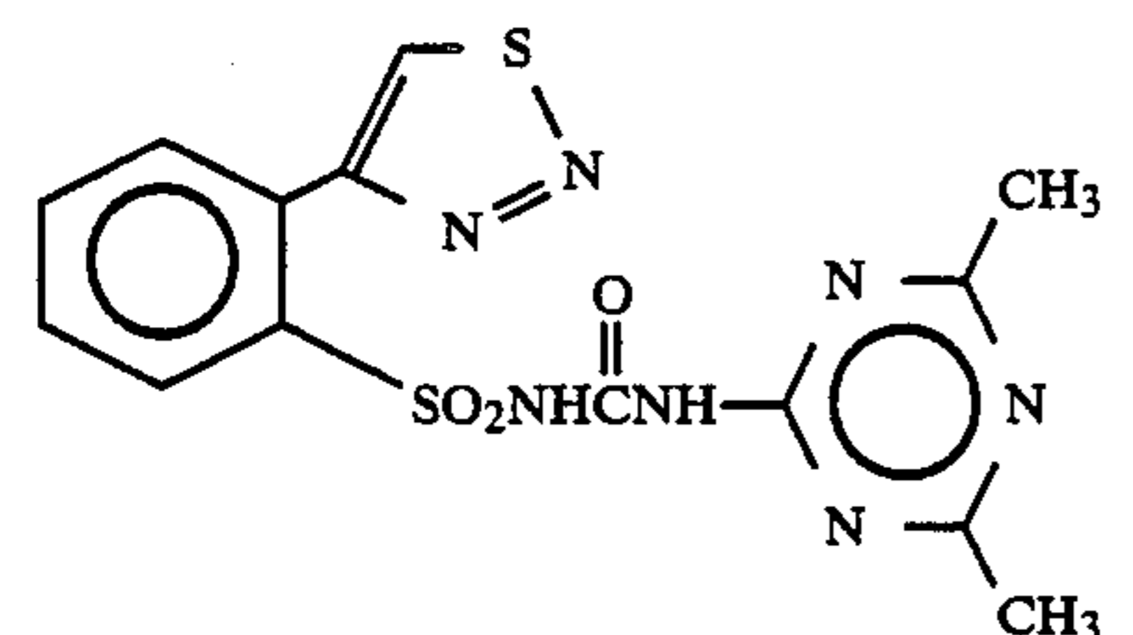
Compound 22
