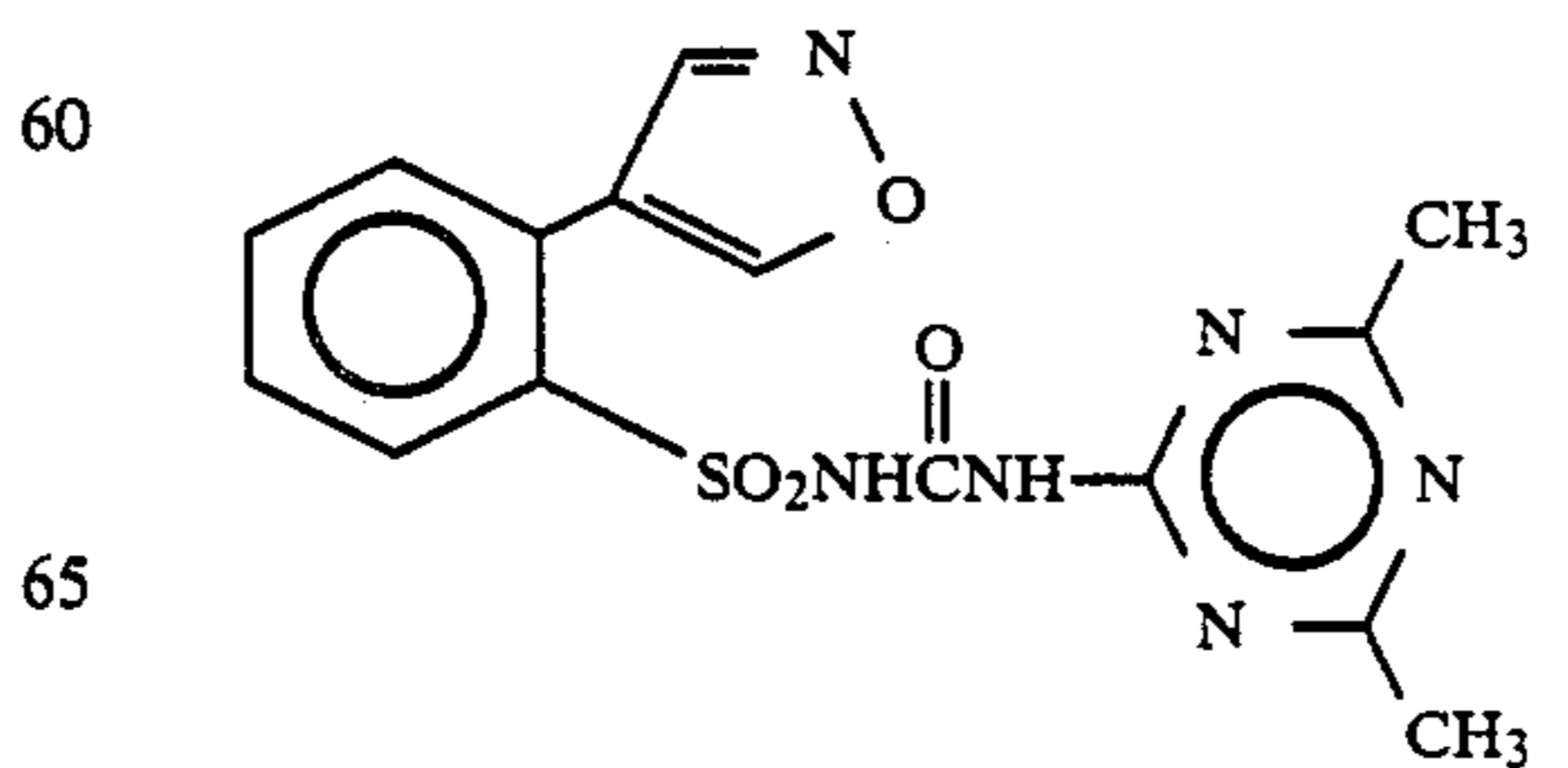
Compound 26
