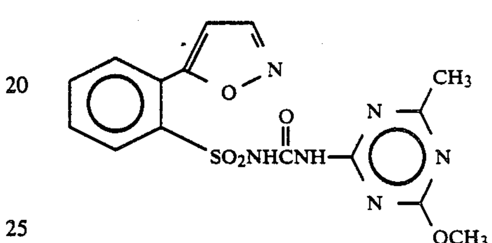
Compound 22
