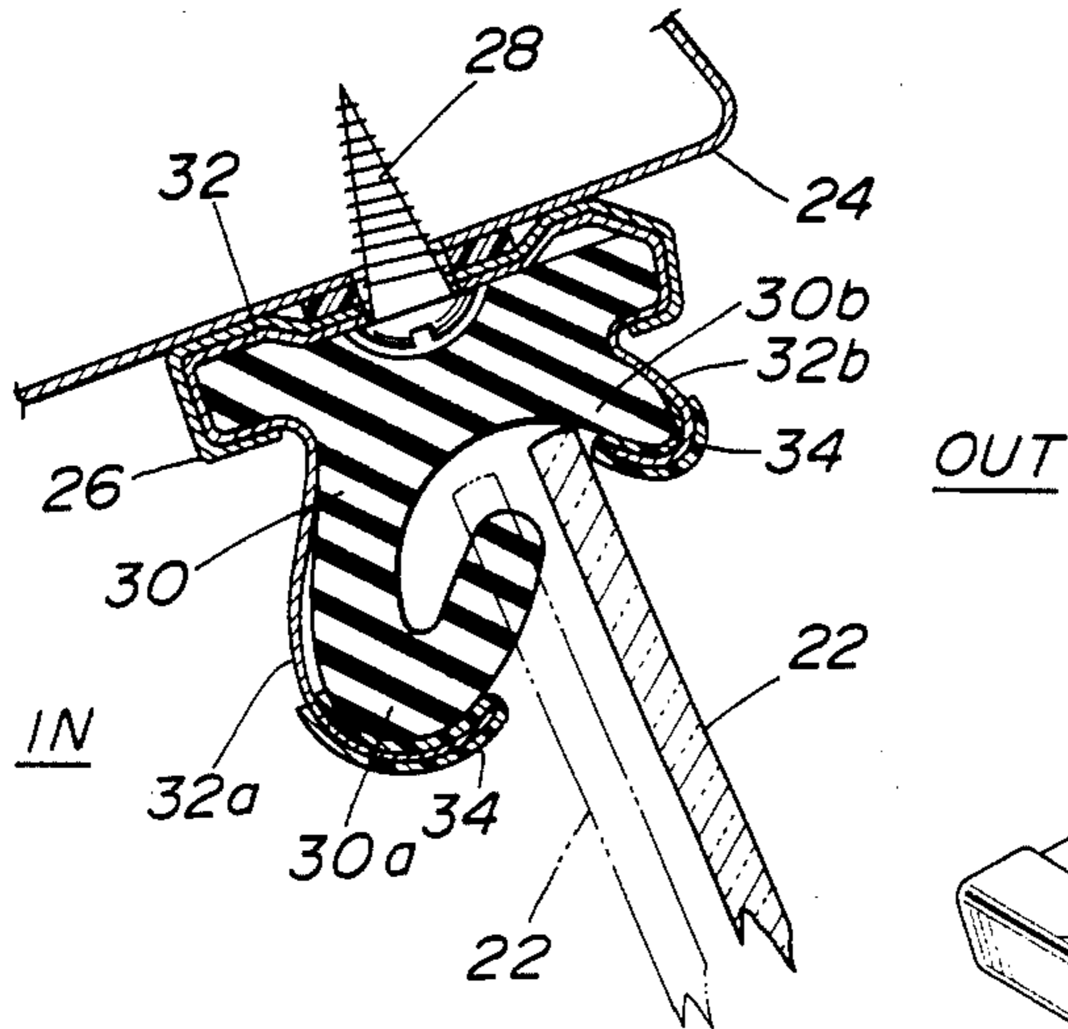
FIG. 2 (PRIOR ART)
