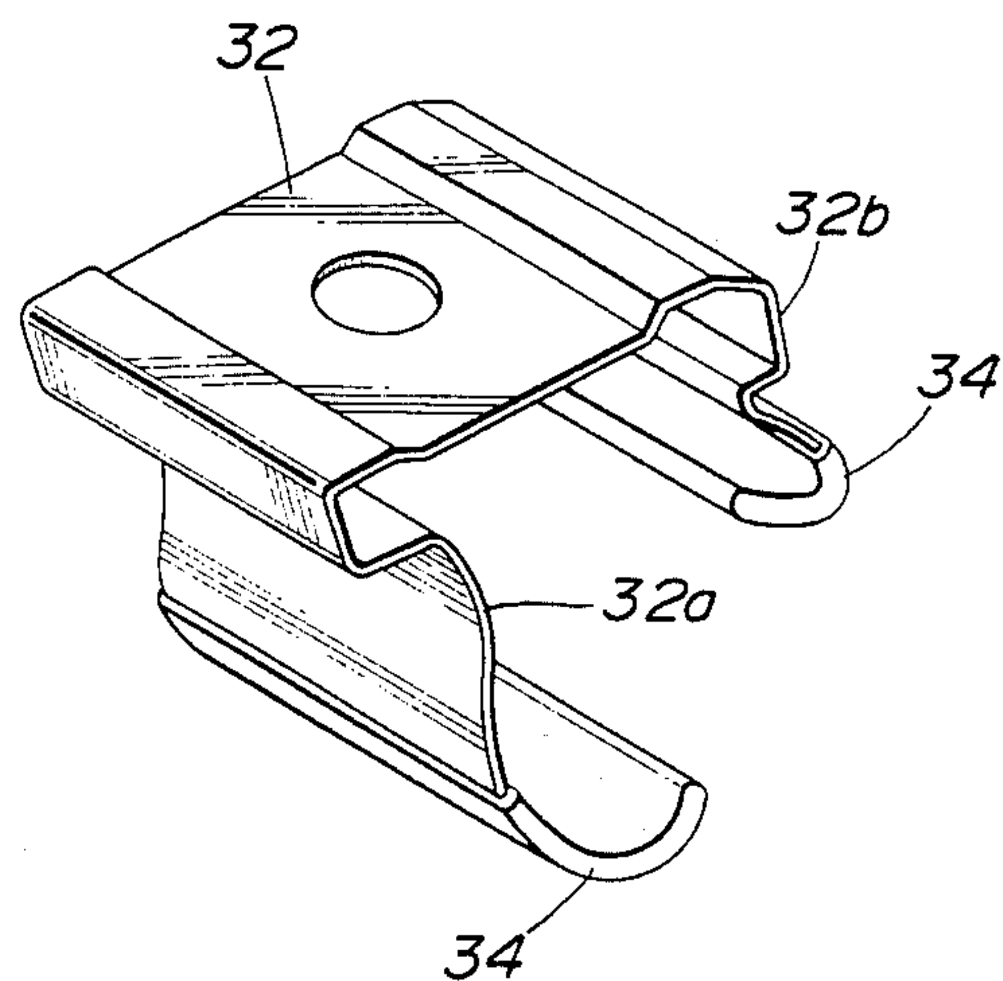
FIG. 3 (PRIOR ART)
