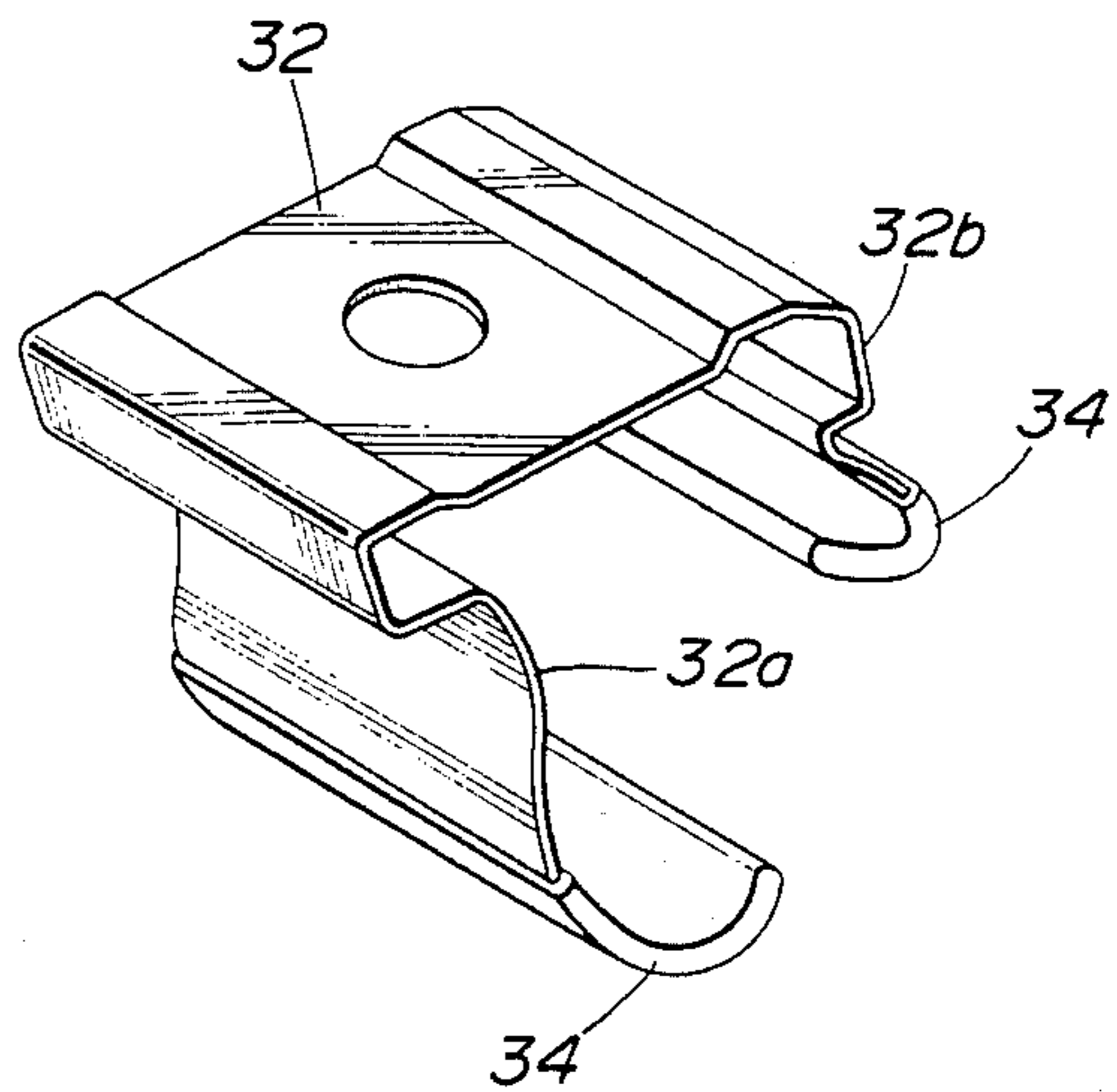
FIG. 3 (PRIOR ART)
