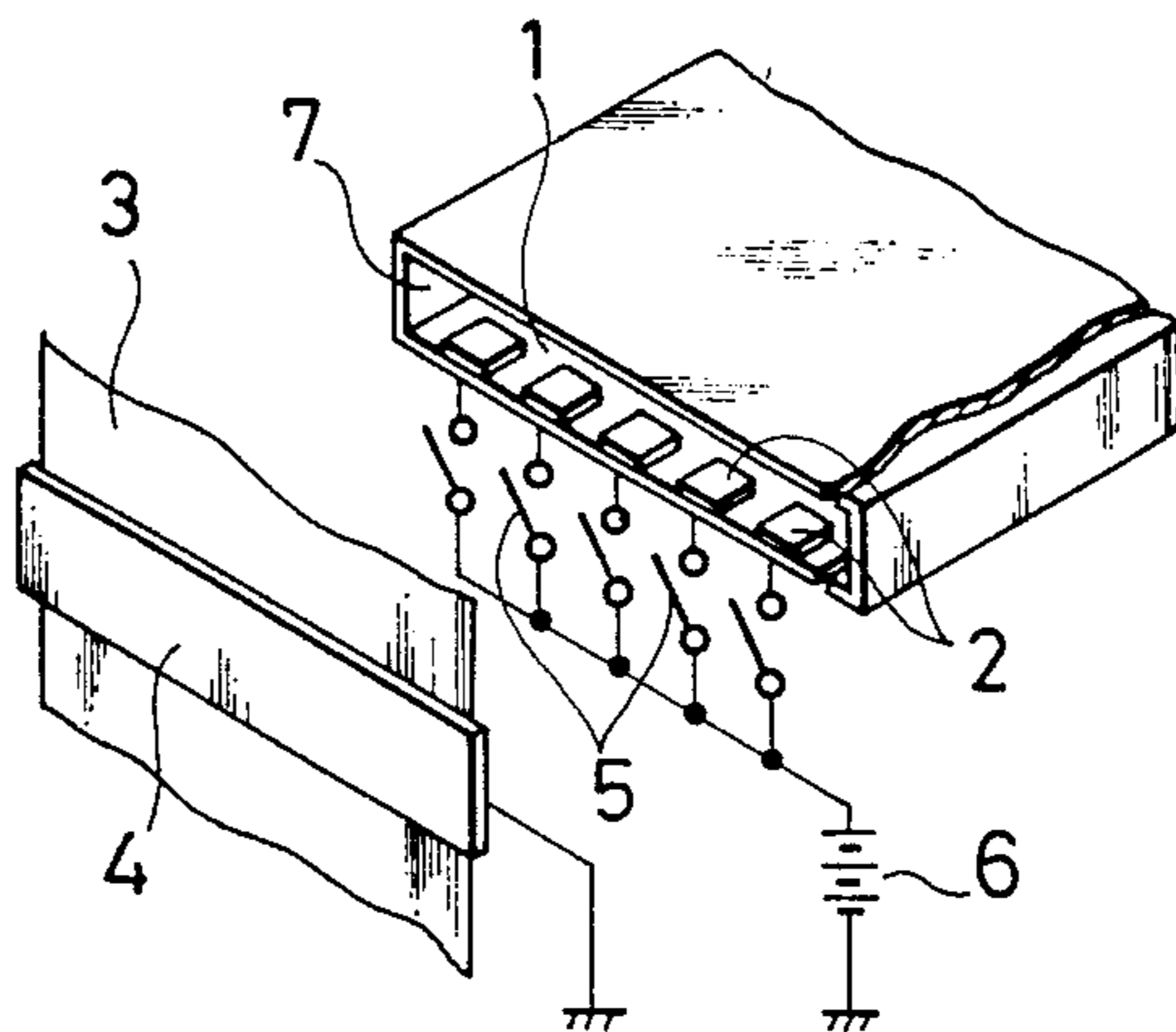
FIG. 27 PRIOR ART
