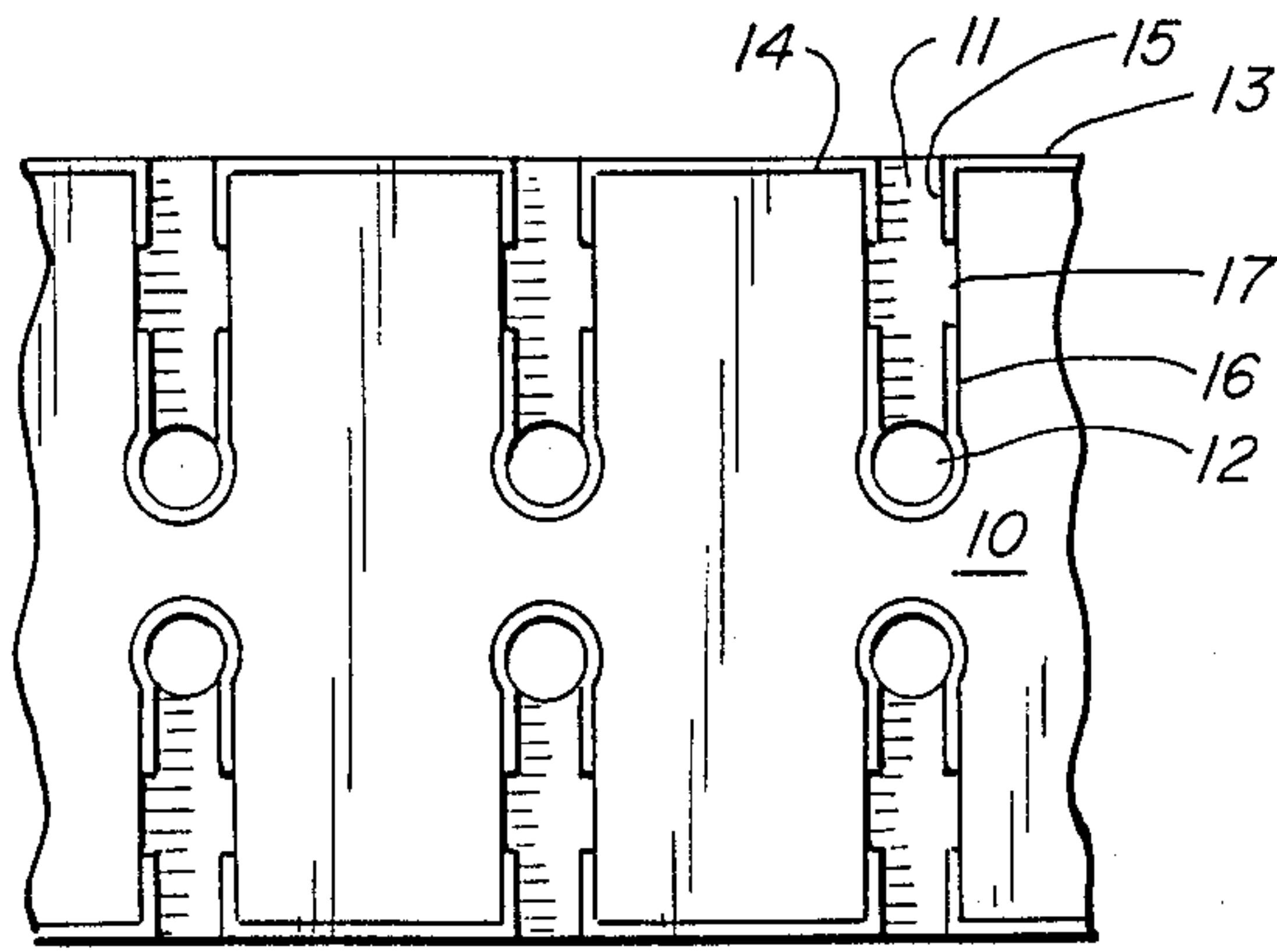
FIG. 1 prior art
