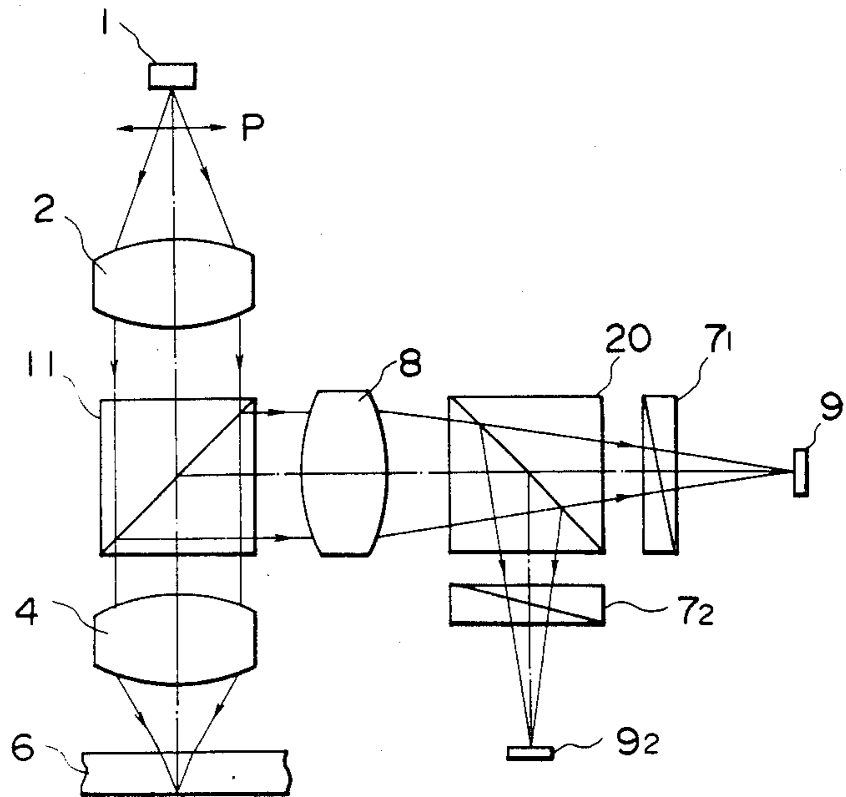
FIG. 1 PRIOR ART
