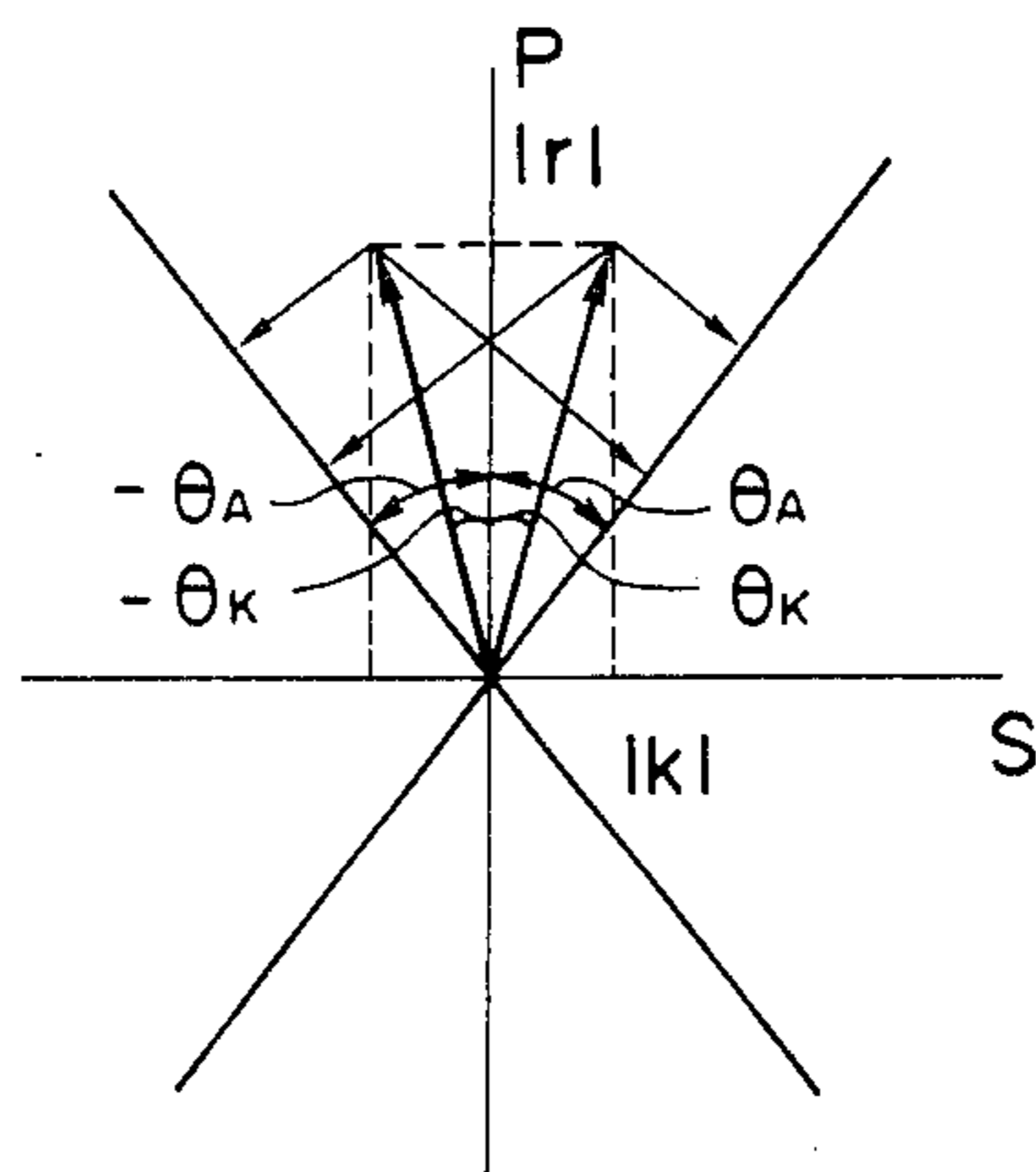
FIG. 2 PRIOR ART
