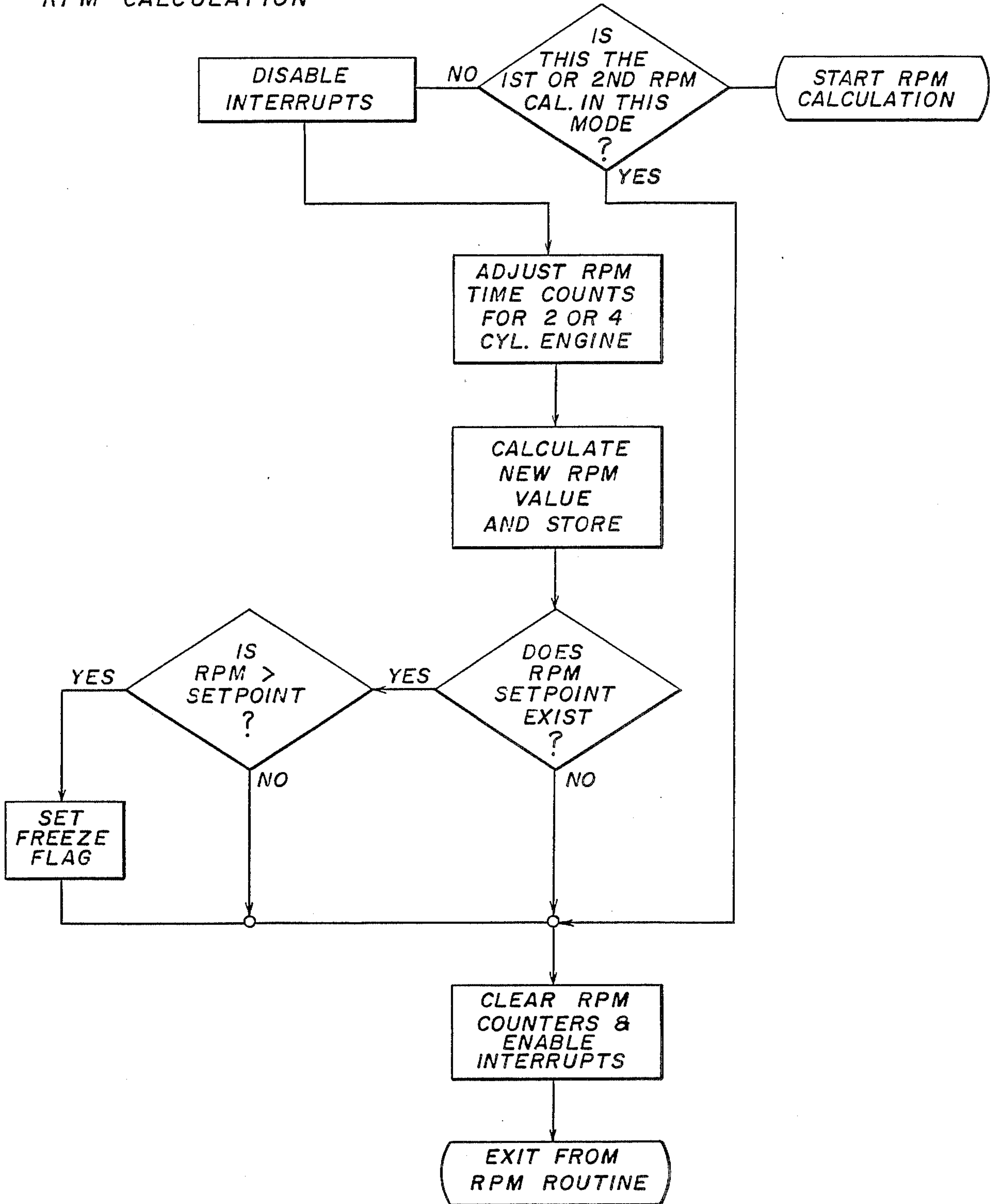
RPM CALCULATION
