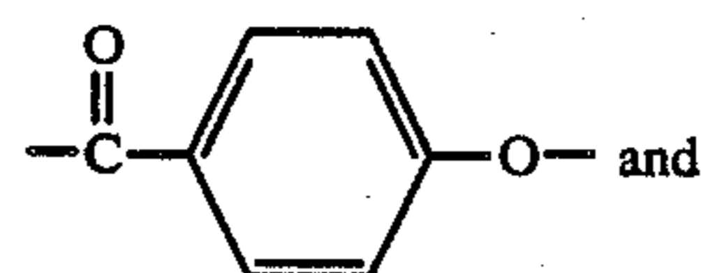
(1,4-benzoate unit)
