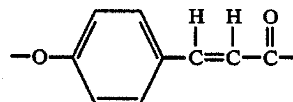
(1,4-cinnamate unit)
