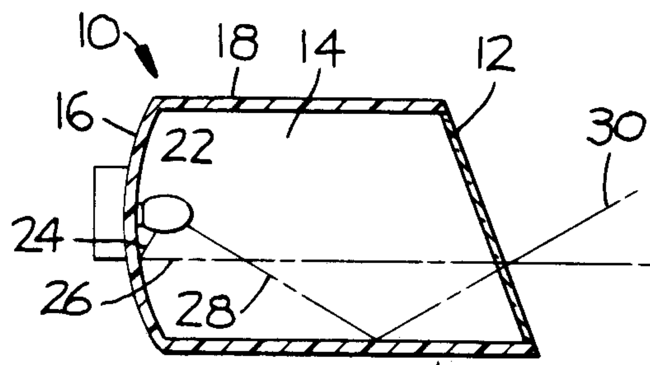
FIG. 2 PRIOR ART
