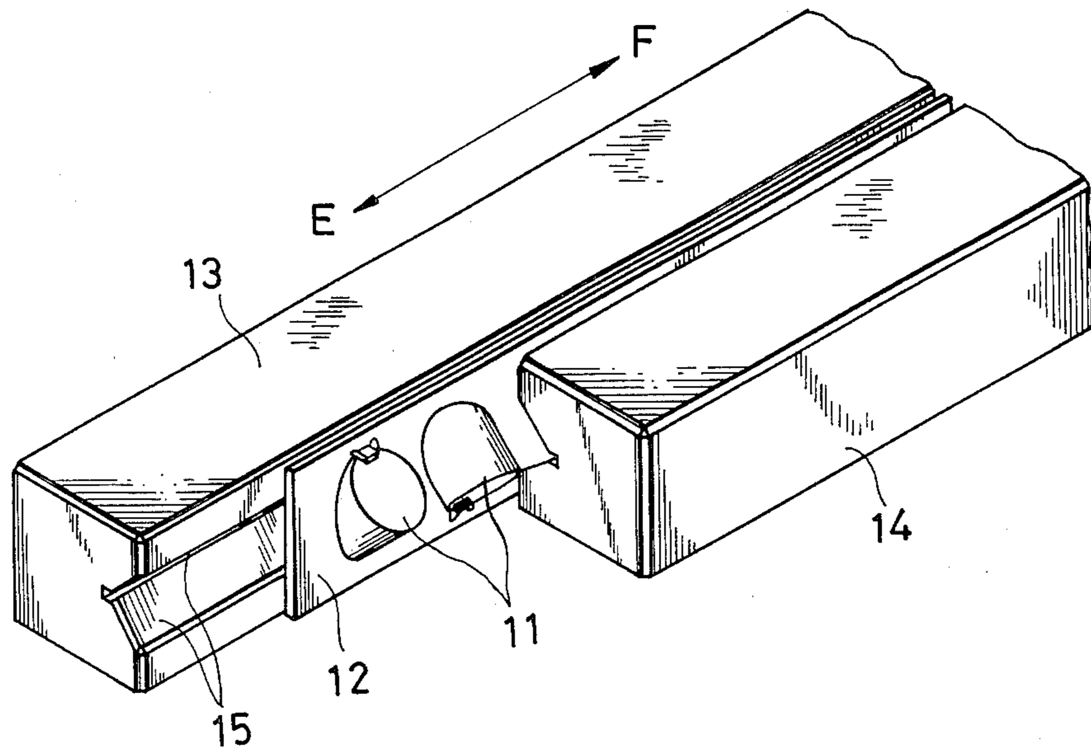
FIG. 17 (Prior Art)
