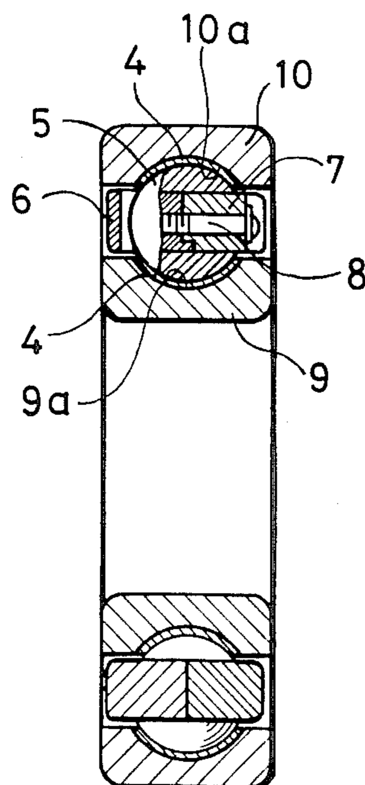
FIG. 15 (Prior Art)
