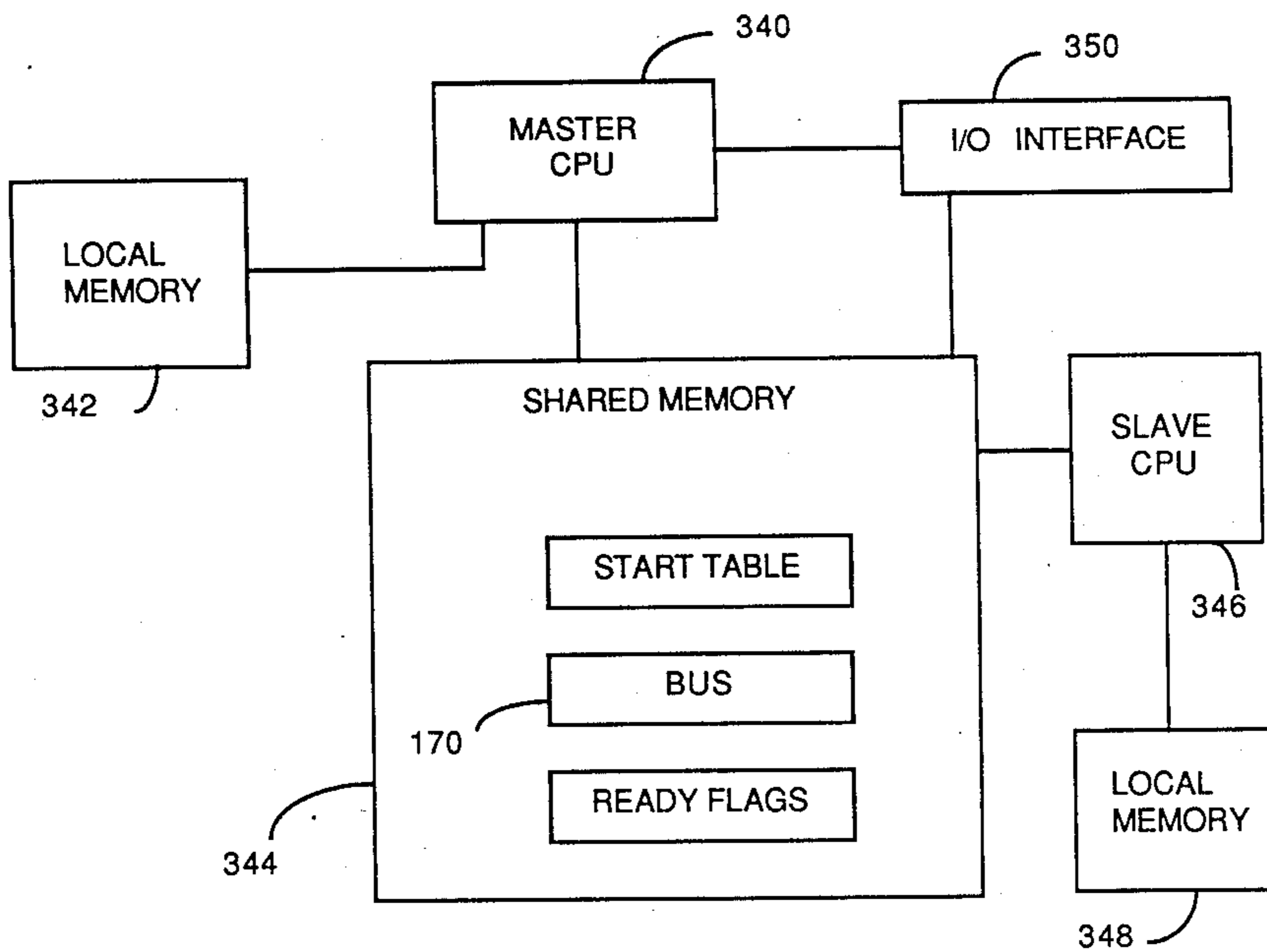
MULTIPROCESSOR CONTROLLER
