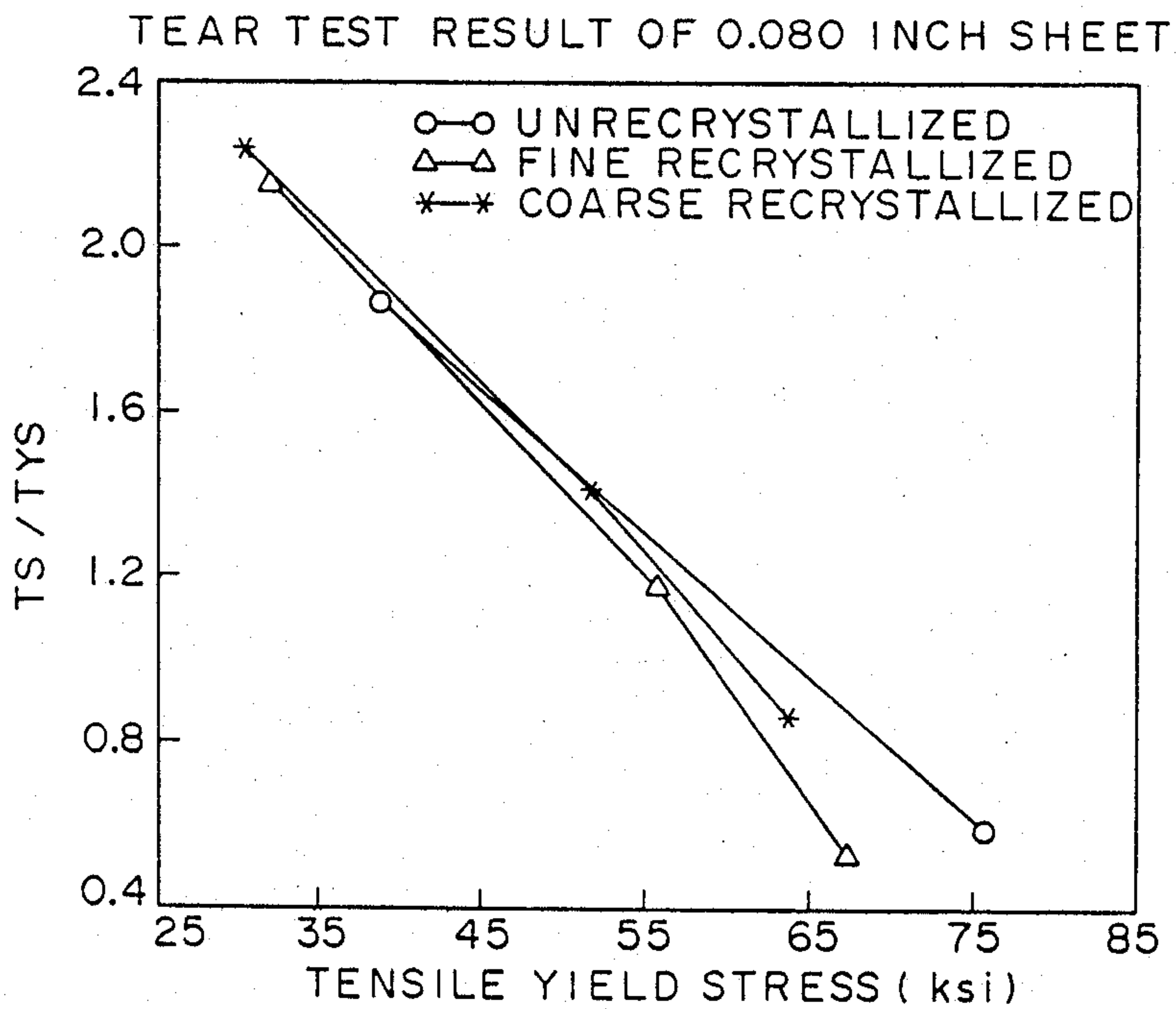
TS / TYS VS. TYS IN LONGITUDINAL DIRECTION
