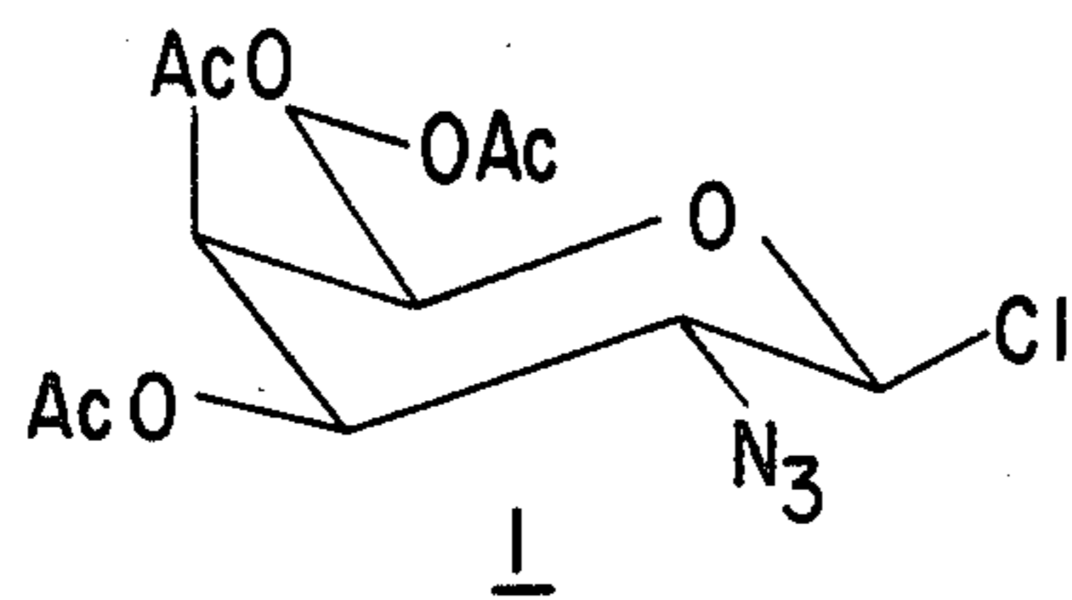
3,4,6- tri- O- acetyl- 2- azido- 2- deoxy- \beta - D- galactopyranosyl chloride
