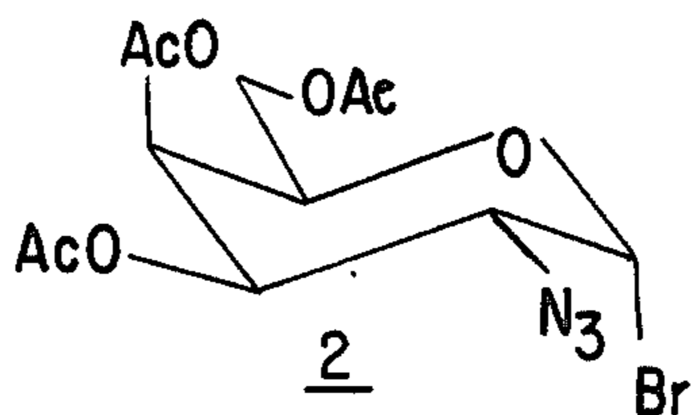
3,4,6- tri- O- acetyl- 2- azido- 2- deoxy- \alpha - D- galactopyranosyl bromide
