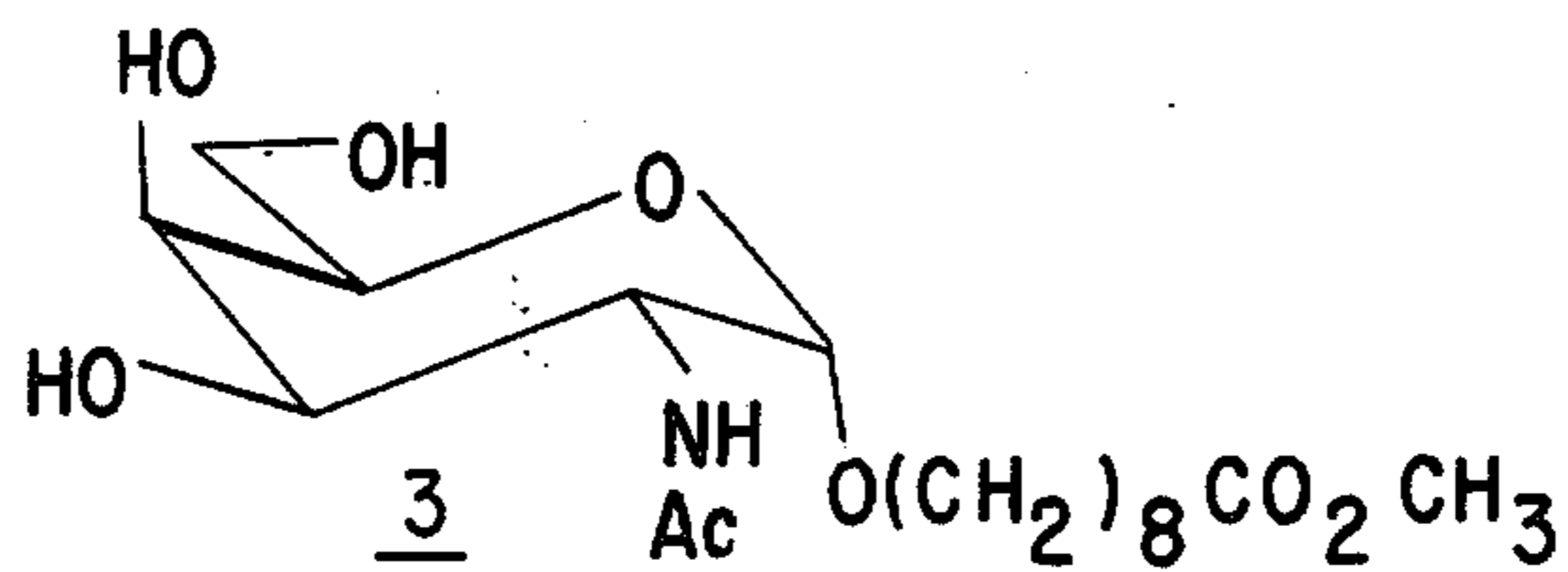
8- methoxycarbonyloctyl - 2- acetamido 2- deoxy- \alpha - D- galactopyranoside
