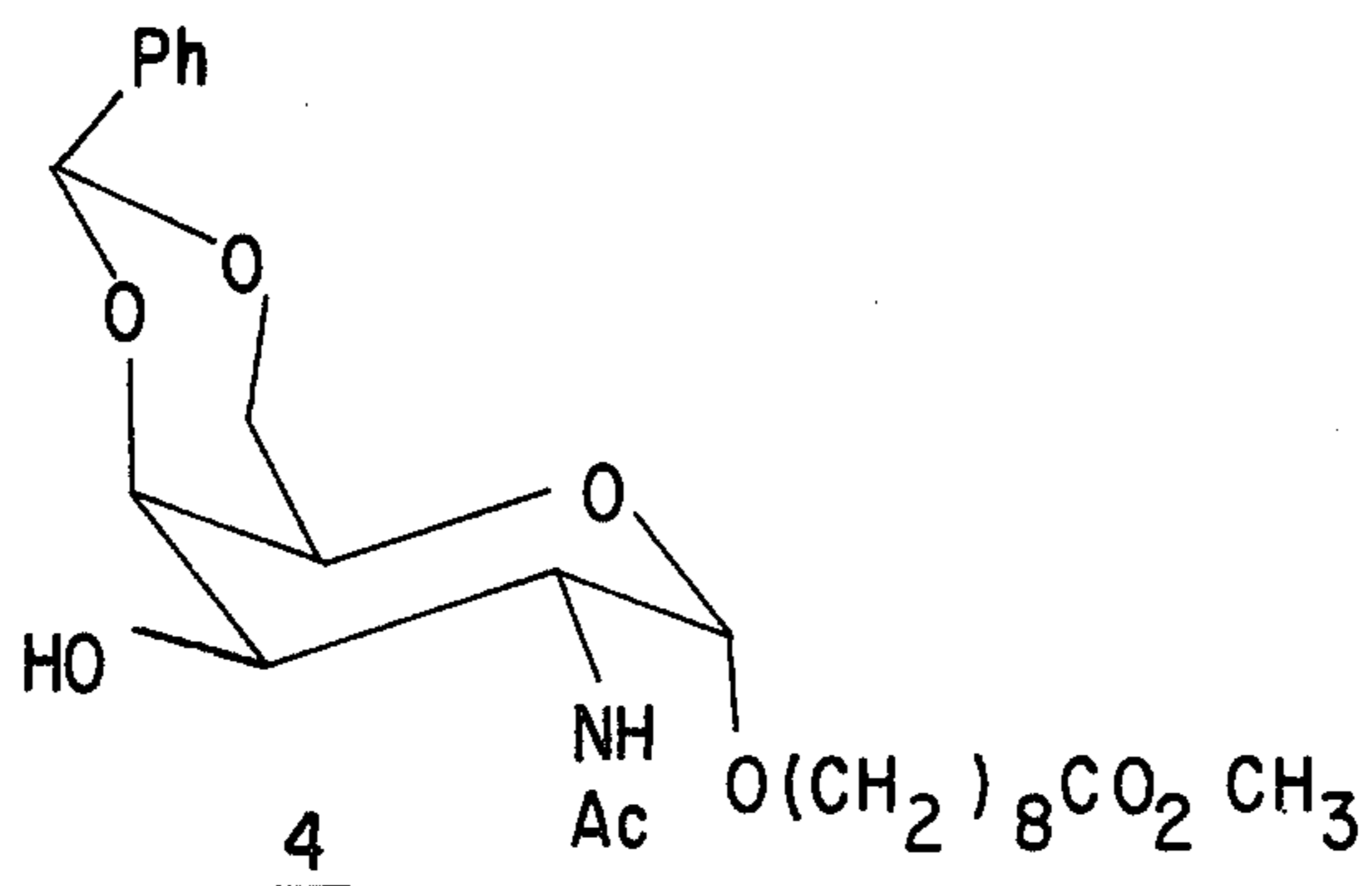
8-methoxycarbonyloctyl-2-acetamido 4,6-O-benzylidene-2-deoxy- \alpha -D-galactopyranoside
