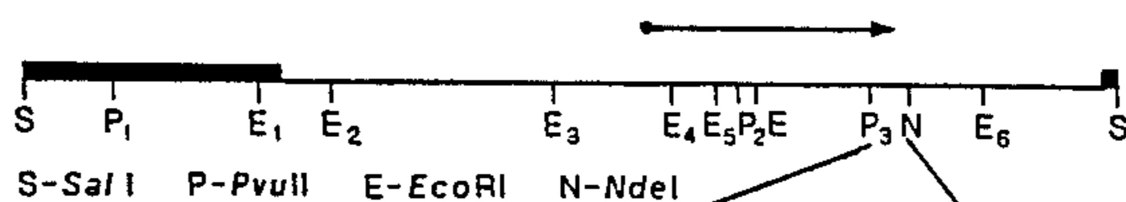
(A) DNA SEQUENCE OF THE 3' FLANKING REGION OF THE CRYSTAL PROTEIN GENE ( Cry )
