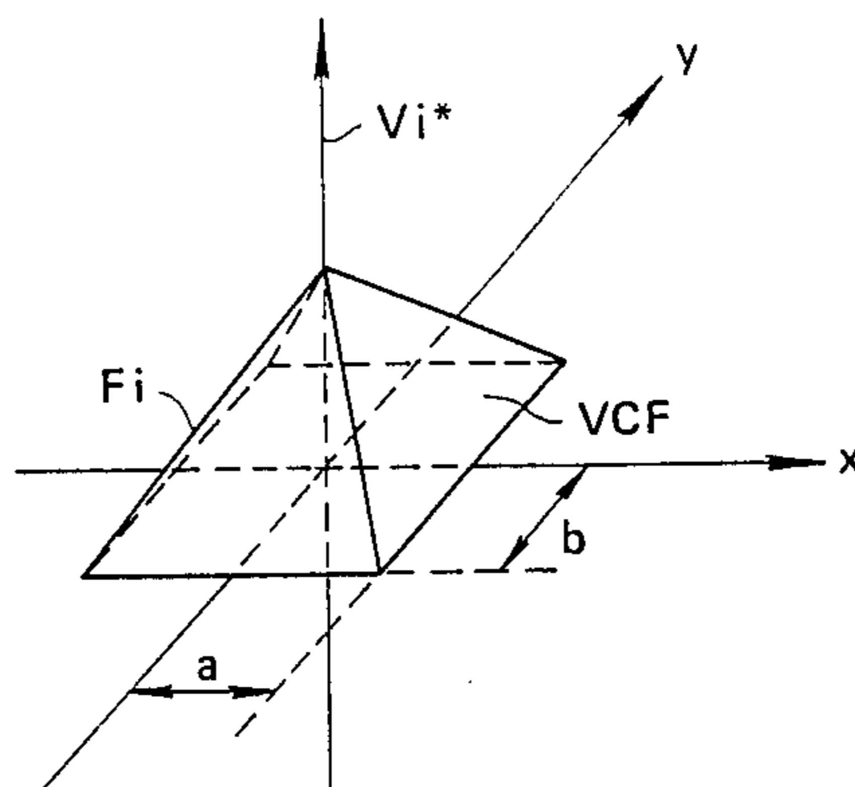
SQUARE CONE TYPE F_i
