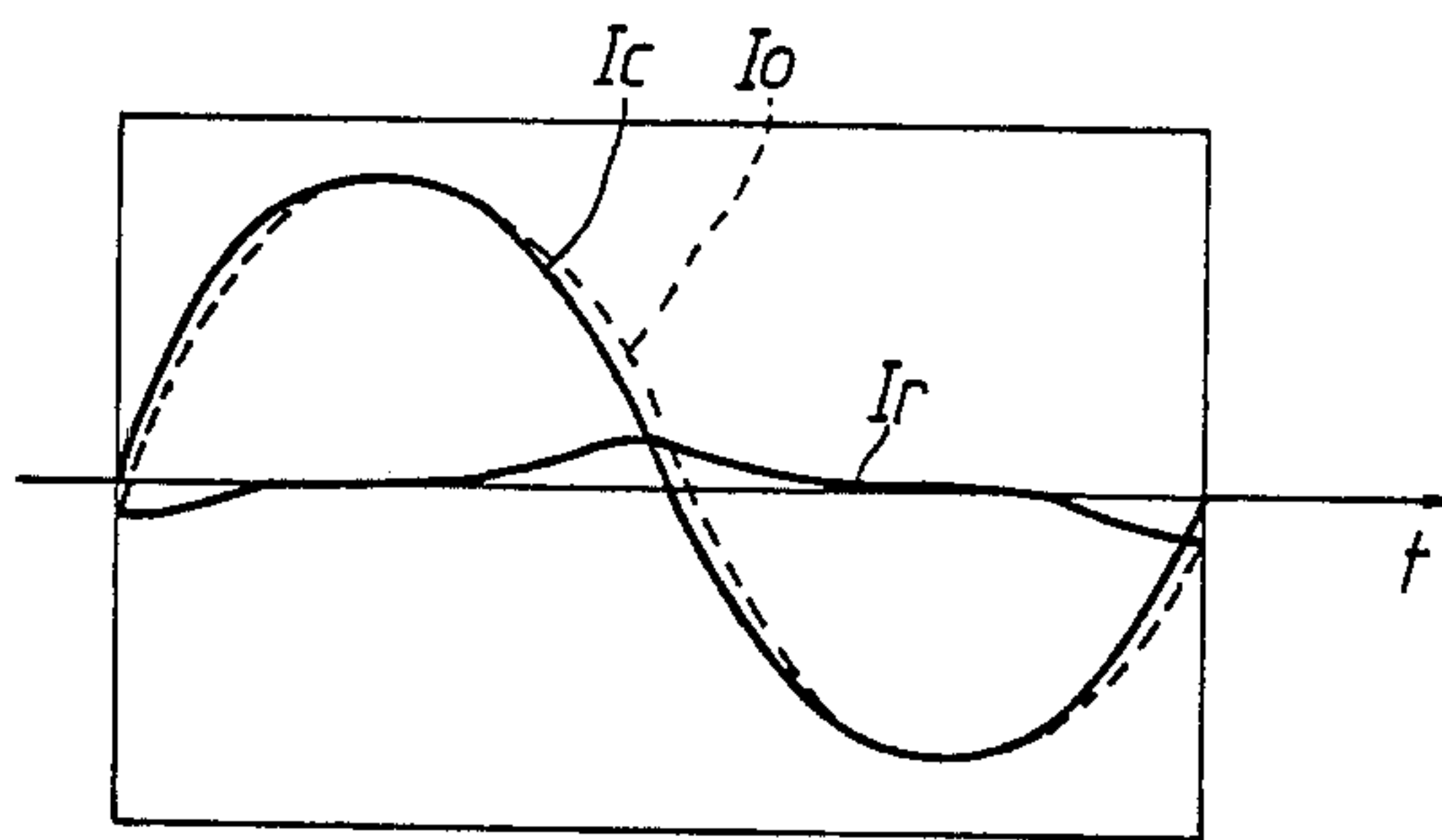
FIG. 8. PRIOR ART
