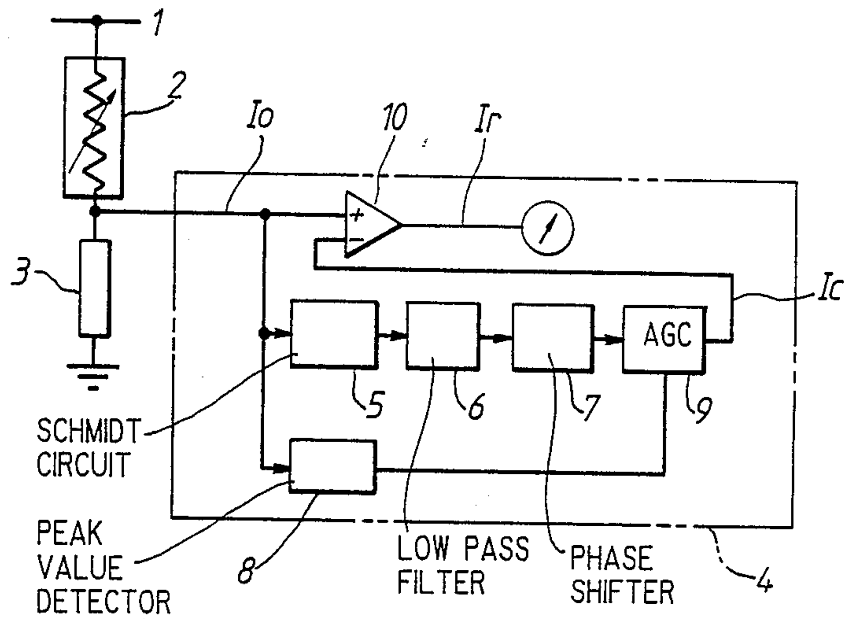
FIG. 6. PRIOR ART
