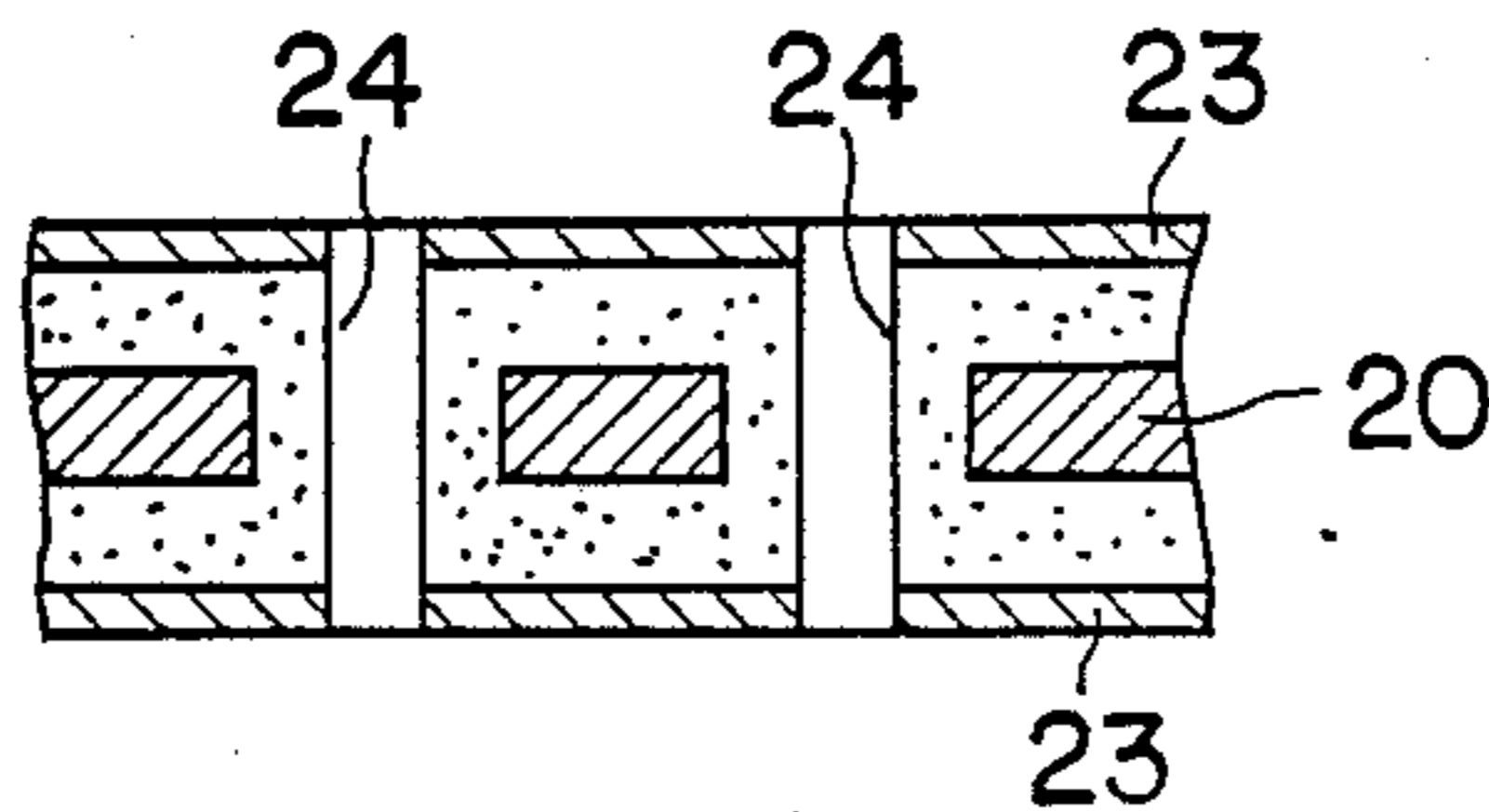
Fig. 2c PRIOR ART
